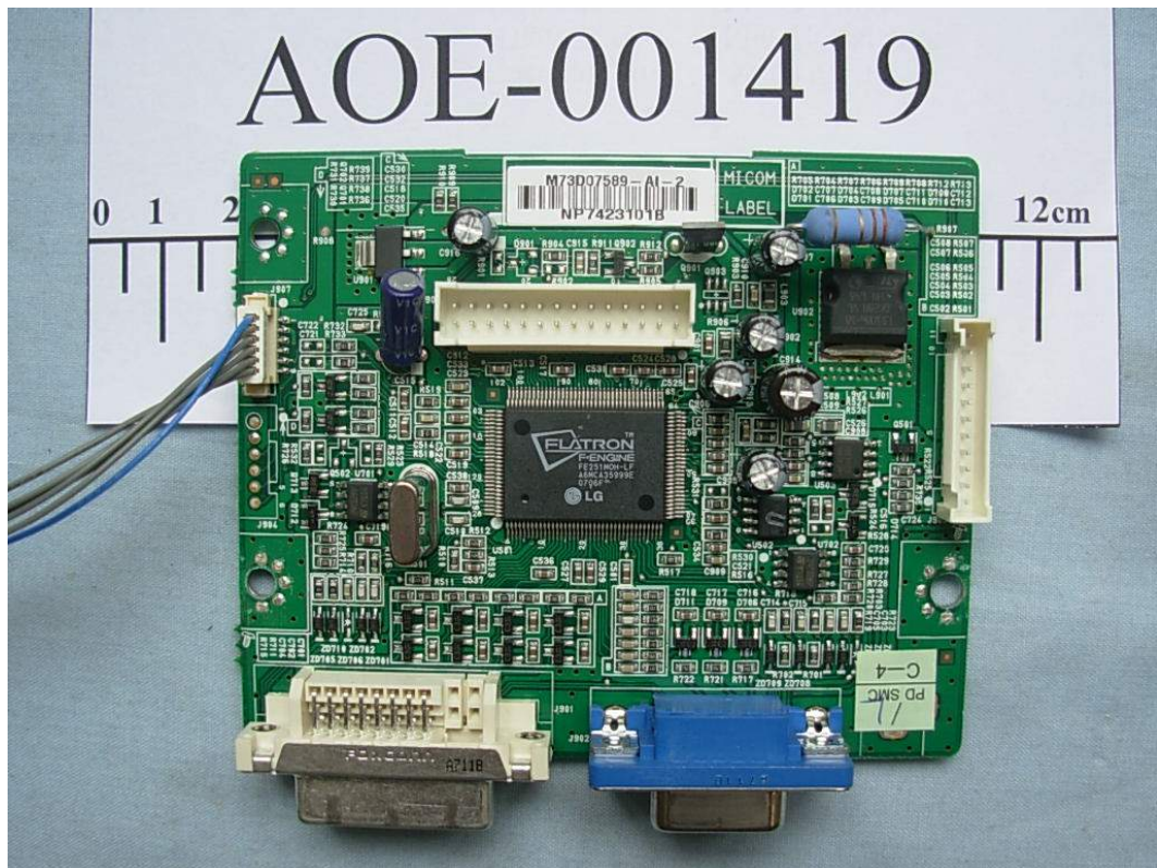
FIGURE 7 LCD MONITOR (M/N: L1954TS) MAIN BOARD (COMPONENT SIDE)
