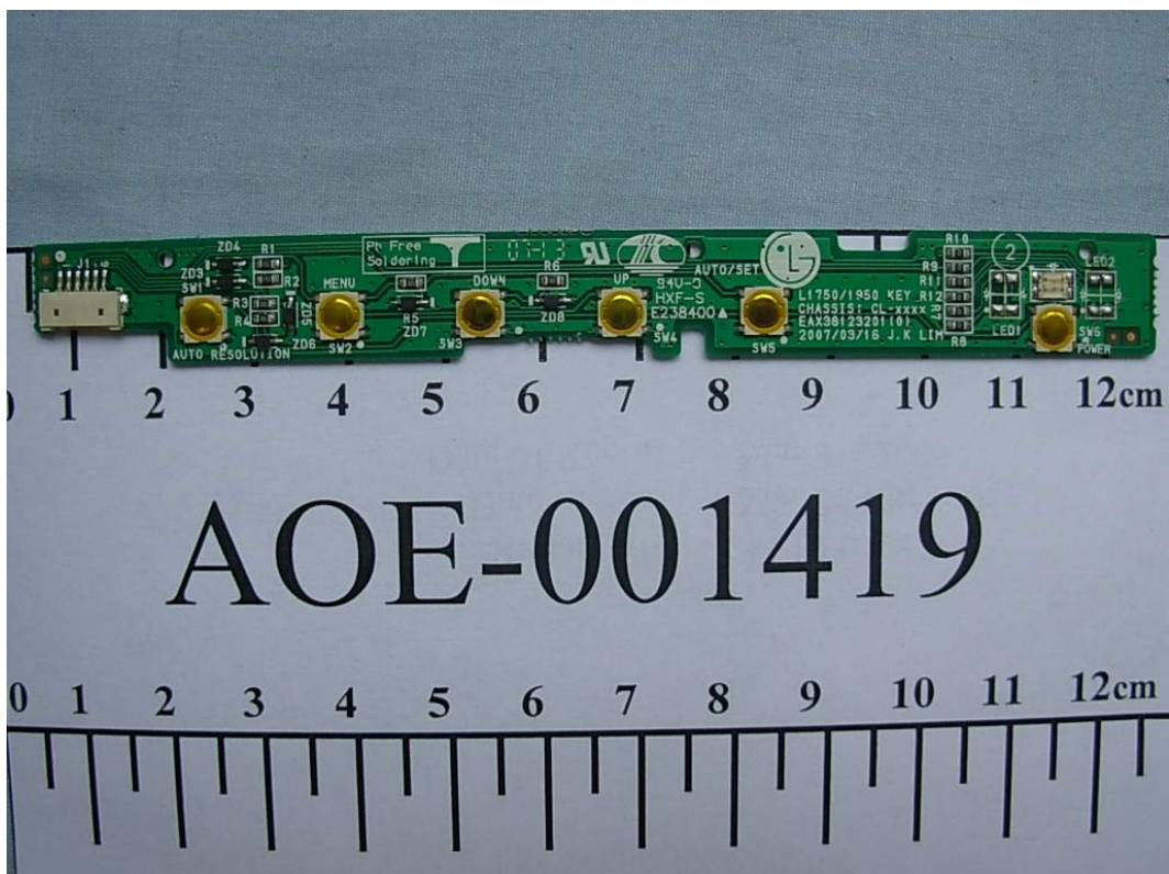
FIGURE 2 LCD MONITOR (M/N: L1954TS) BUTTON BOARD FRONT
