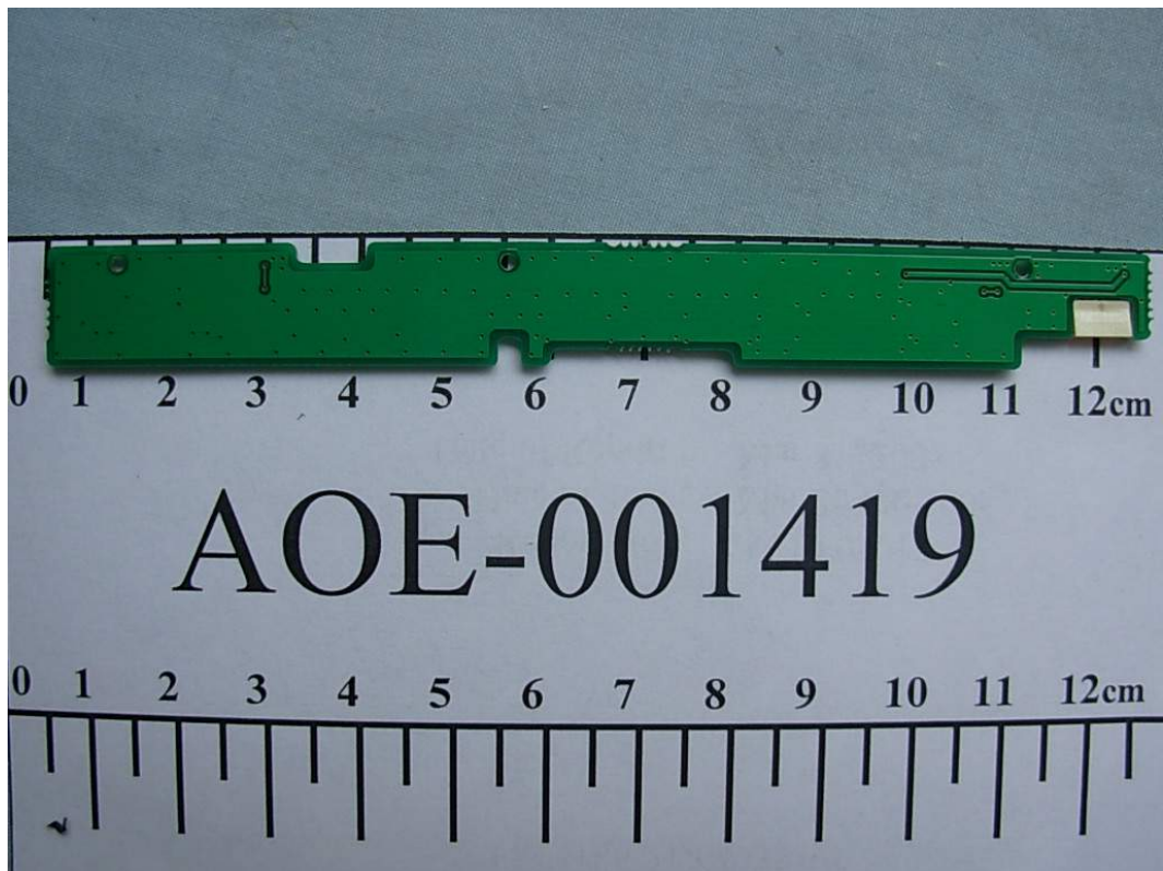
FIGURE 3 LCD MONITOR (M/N: L1954TS) BUTTON BOARD BACK
