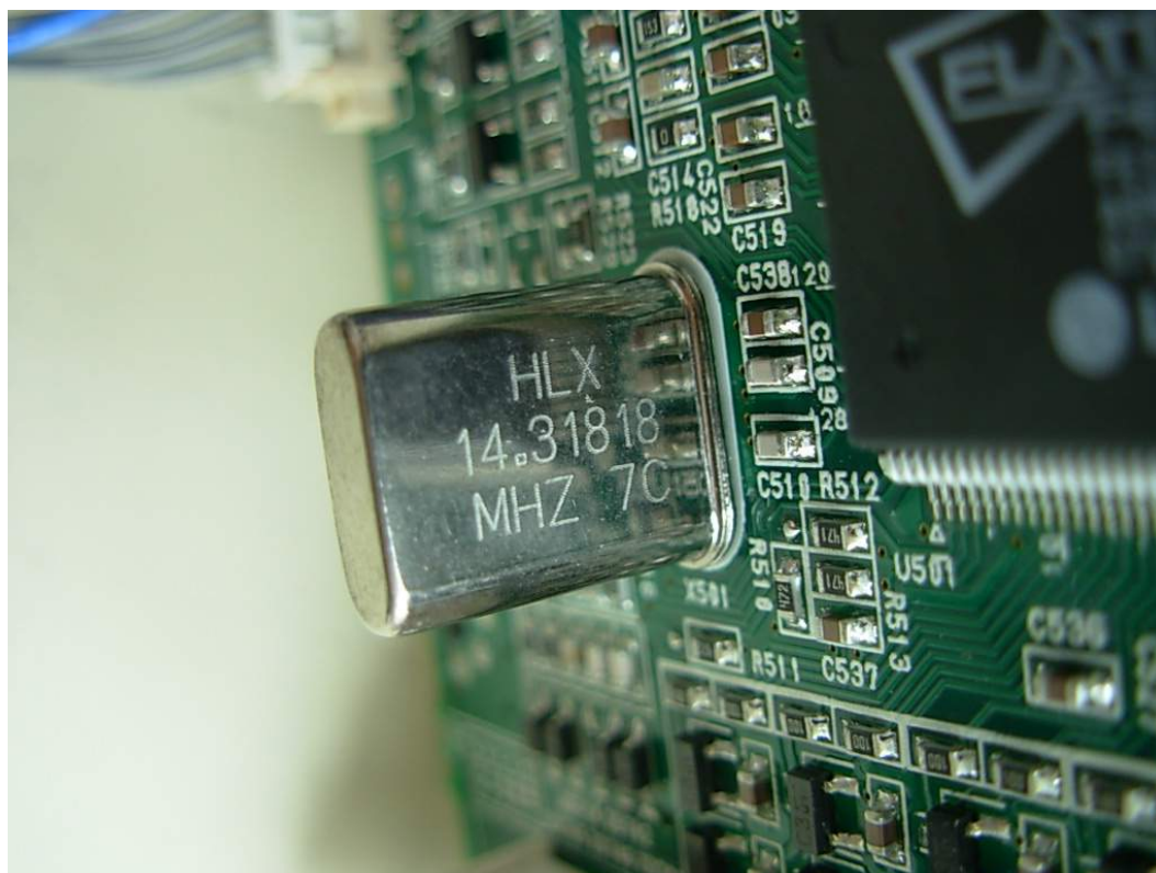
FIGURE 10 LCD MONITOR (M/N: L1954TS) CRYSTAL ON MAIN BOARD
