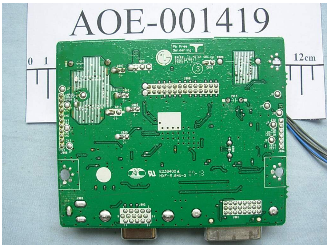
FIGURE 8 LCD MONITOR (M/N: L1954TS) MAIN BOARD (SOLDERED SIDE)
