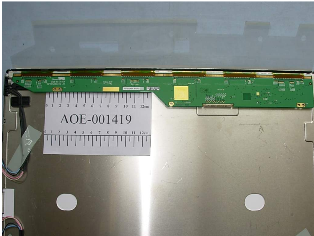
FIGURE 15 LCD MONITOR (M/N: L1954TS) LCD PANEL MAIN BOARD FRONT
