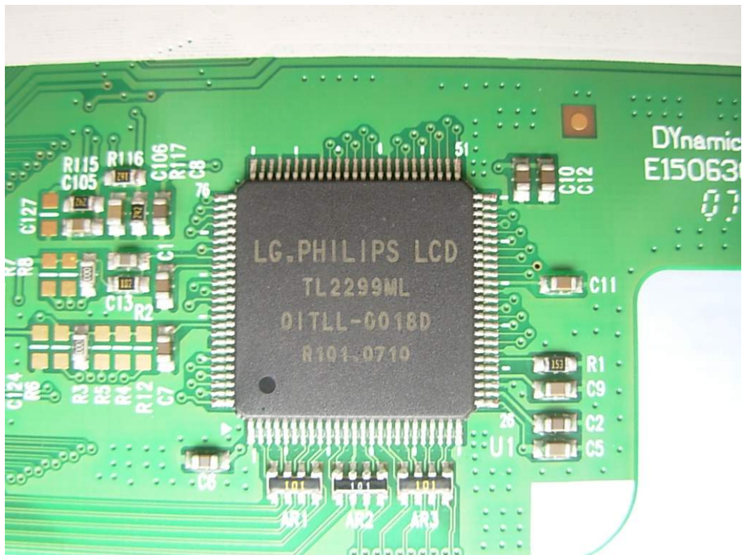
FIGURE 19 LCD MONITOR (M/N: L1954SMS) CHIP ON LCD PANEL MAIN BOARD
