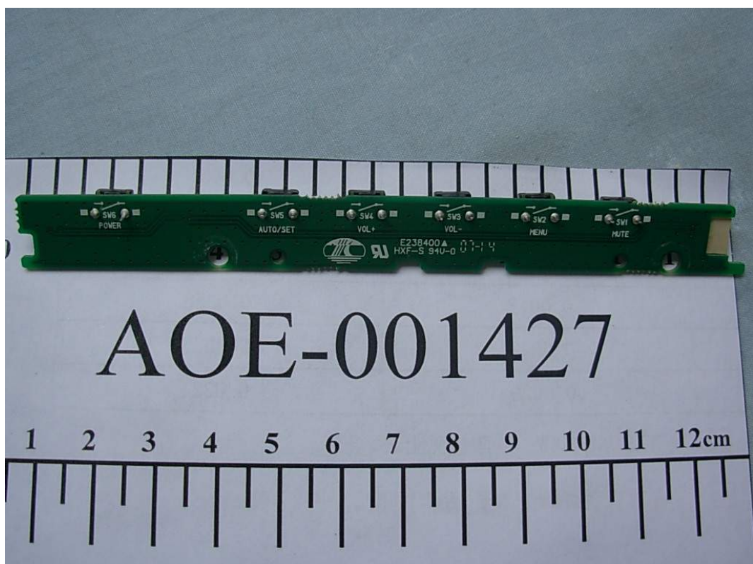
FIGURE 4 LCD MONITOR (M/N: L1954SMS) BOTTOM BOARD (SOLDERED SIDE)
