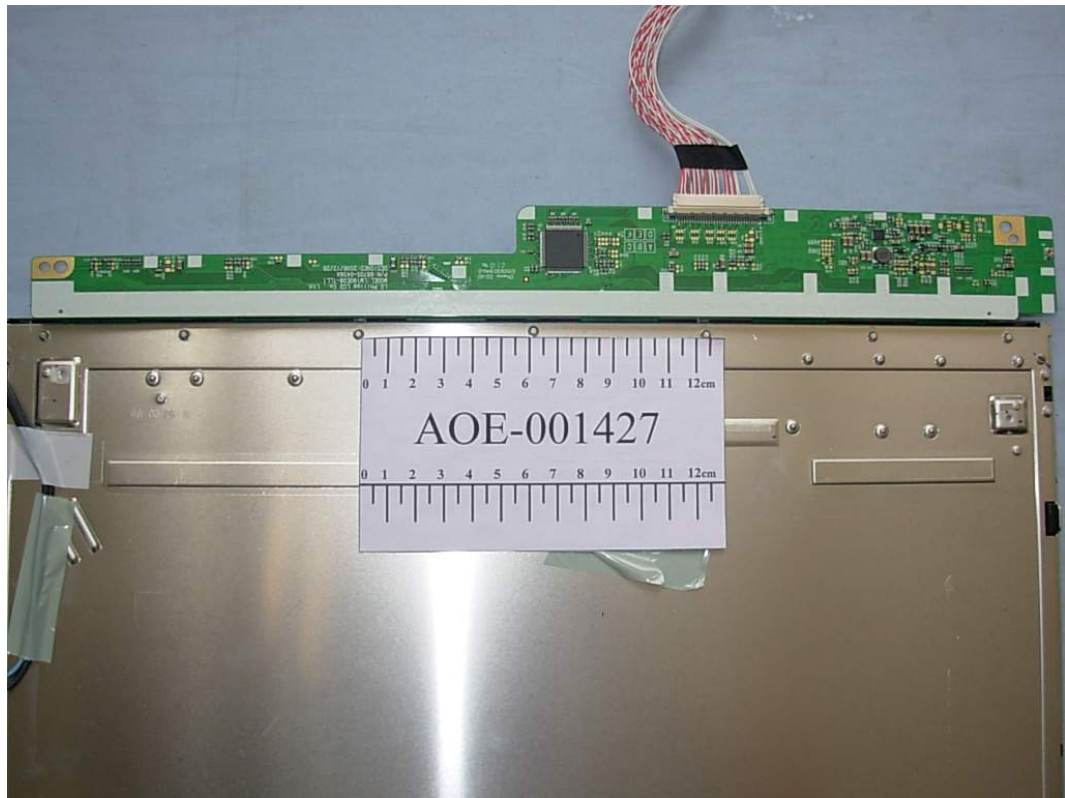
FIGURE 17 LCD MONITOR (M/N: L1954SMS) LCD PANEL MAIN BOARD (BACK VIEW)
