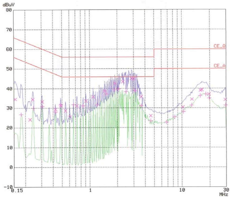
< Neutral line >
