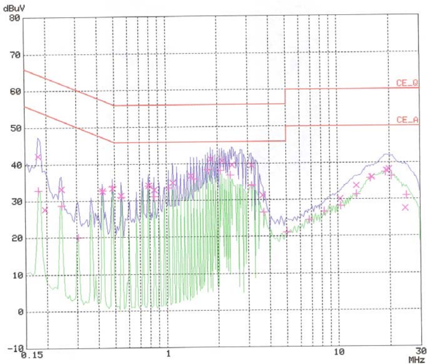
< Hot line >
