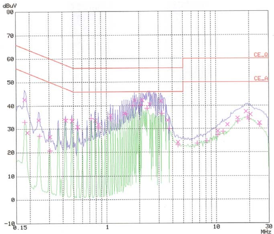
< Neutral line >
