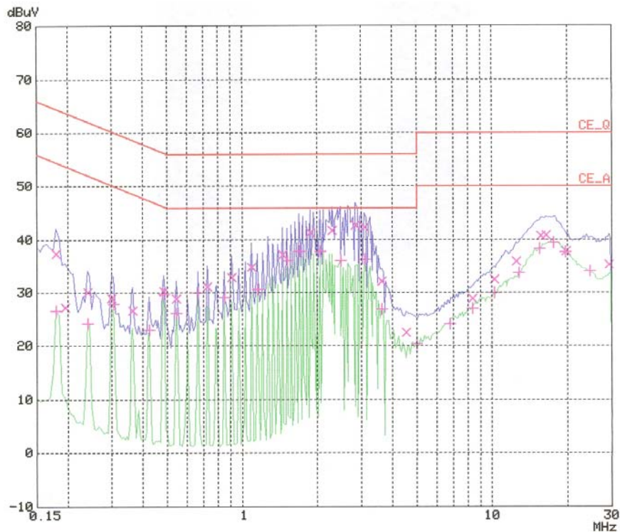
< Hot line >
