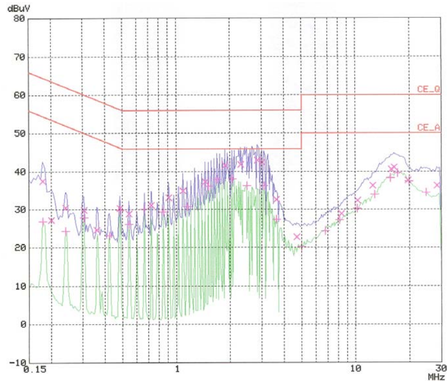
< Hot line >
