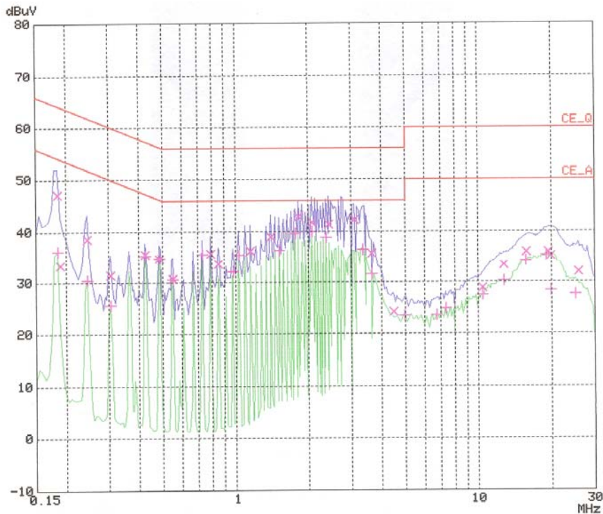
< Neutral line >
