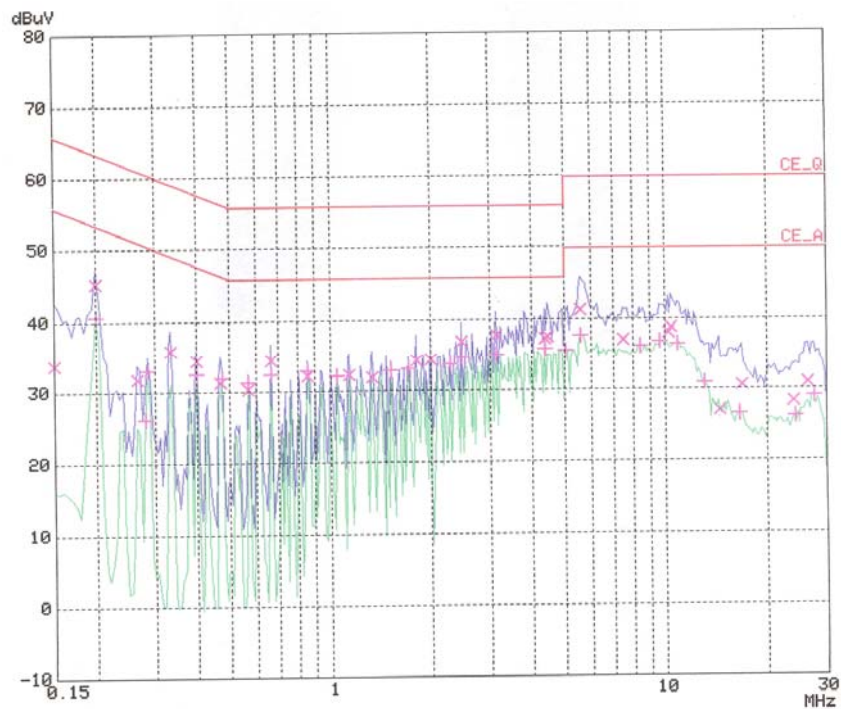
< Hot line >
