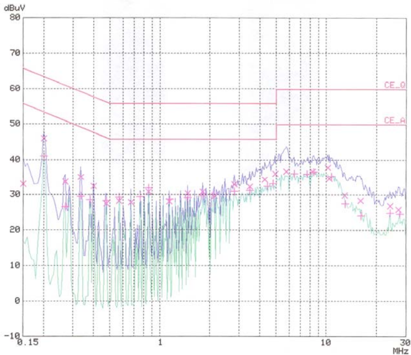
< Neutral line >
