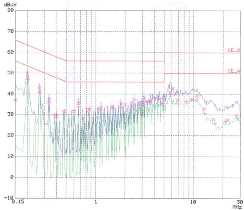
< Hot line >
