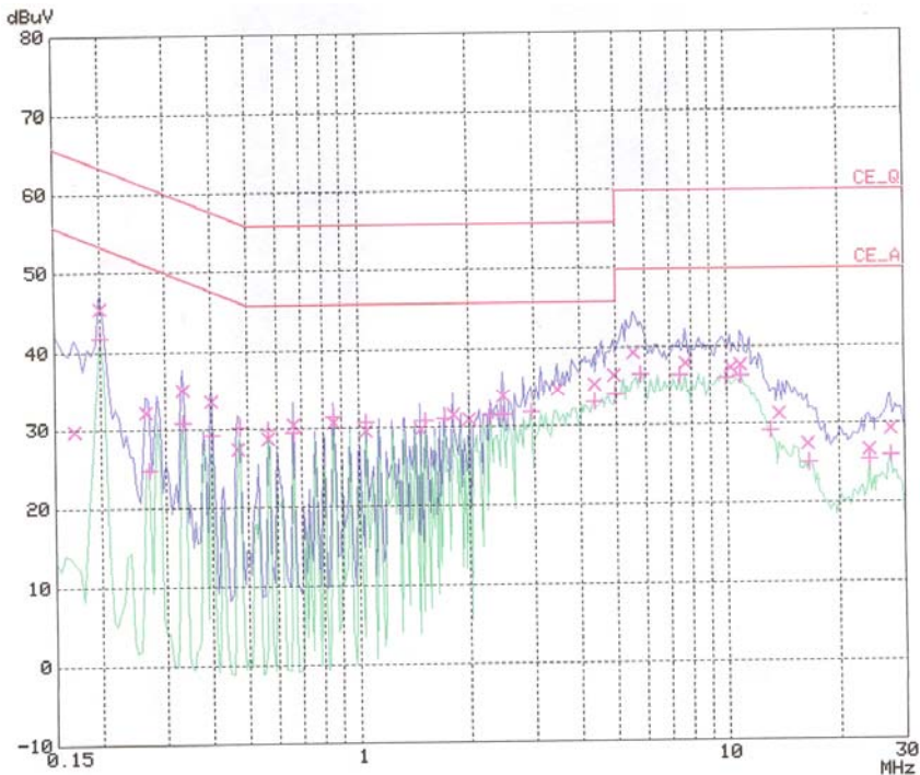
< Neutral line >
