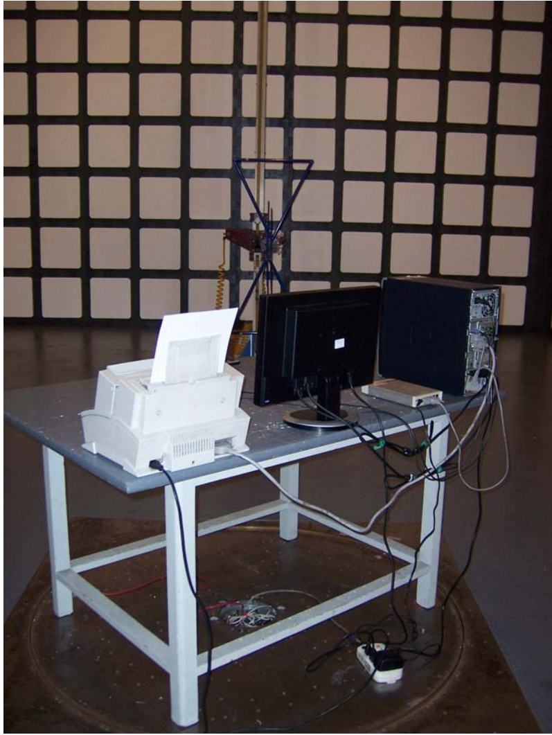
SETUP WITH MAXIMUM DETECTED EMISSION AT VERTICAL POLARIZATION (DVI 720*480@60Hz)
