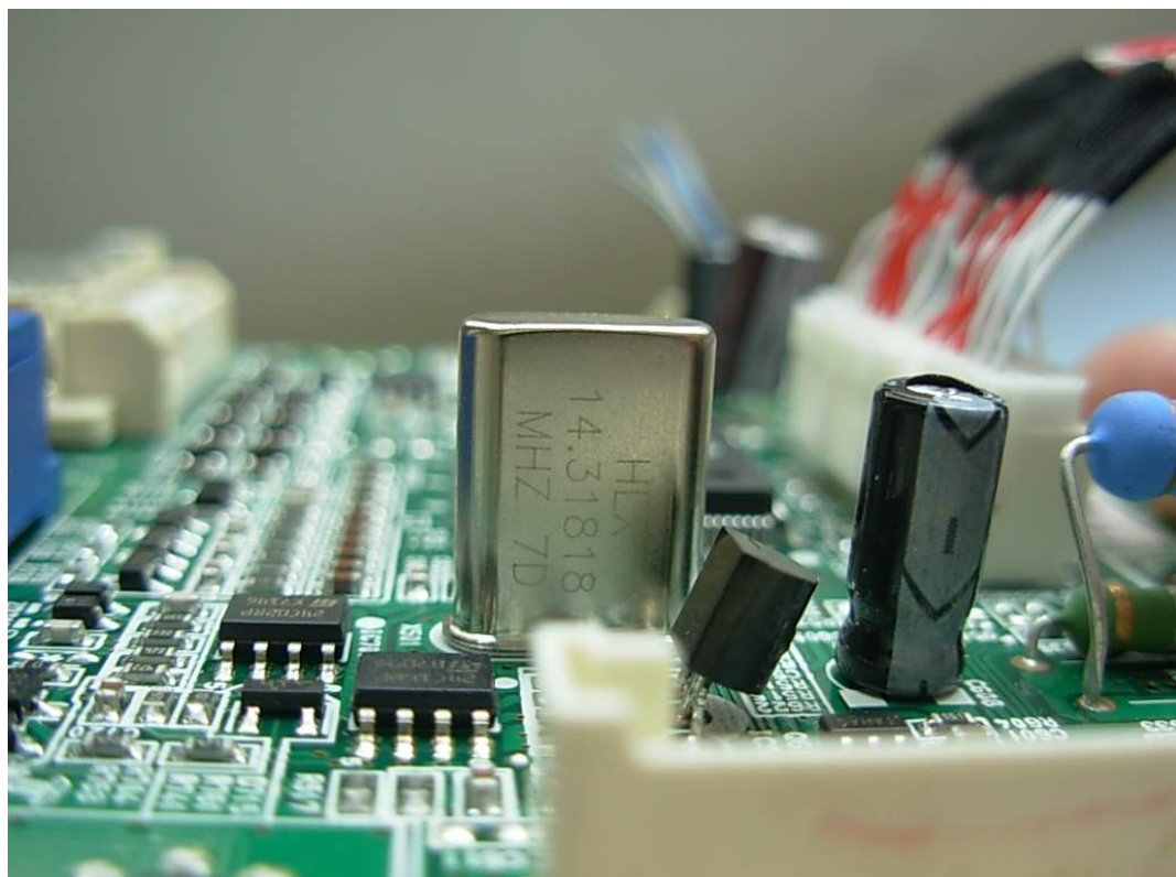
FIGURE 8 LCD MONITOR (M/N: L204WTS) CRYSTAL ON MAIN BOARD
