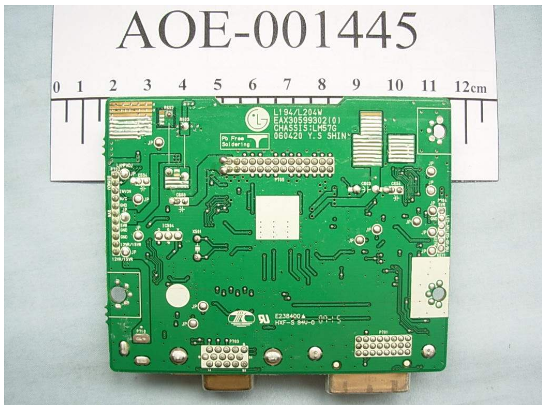
FIGURE 6 LCD MONITOR (M/N: L204WTS) MAIN BOARD (SOLDERED SIDE)
