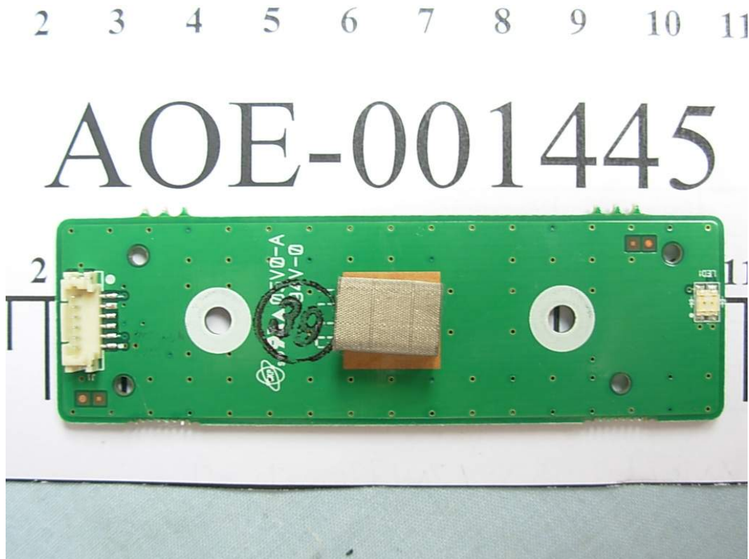
FIGURE 4 LCD MONITOR (M/N: L204WTS) BOARDS REMOVED
