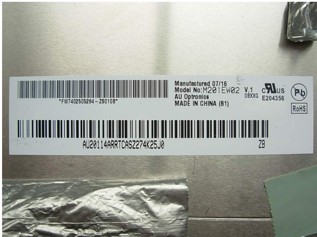
FIGURE 11 LCD MONITOR (M/N: L204WTS) LABEL ON LCD PANEL
