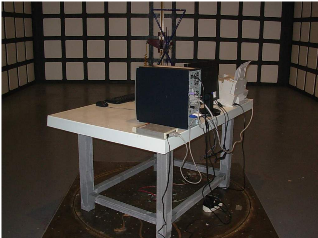
SETUP WITH MAXIMUM DETECTED EMISSION AT VERTICAL POLARIZATION (DVI 1680*1050@60Hz, LOW FREQUENCY)
