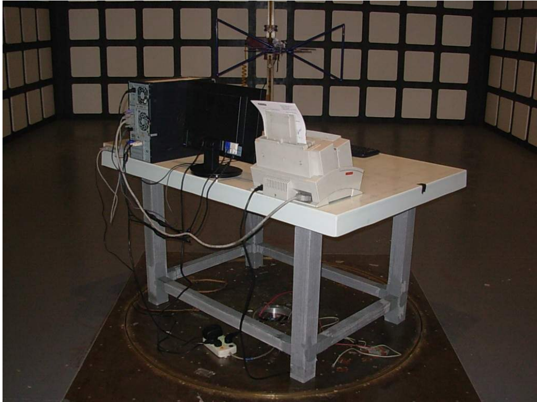
SETUP WITH MAXIMUM DETECTED EMISSION AT HORIZONTAL POLARIZATION (DVI 1680*1050@60Hz, LOW FREQUENCY)
