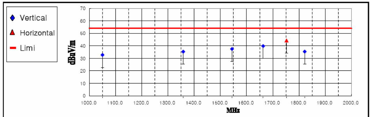
< Fig 8. Radiated emission result (1000MHz ~ 2000MHz)>
