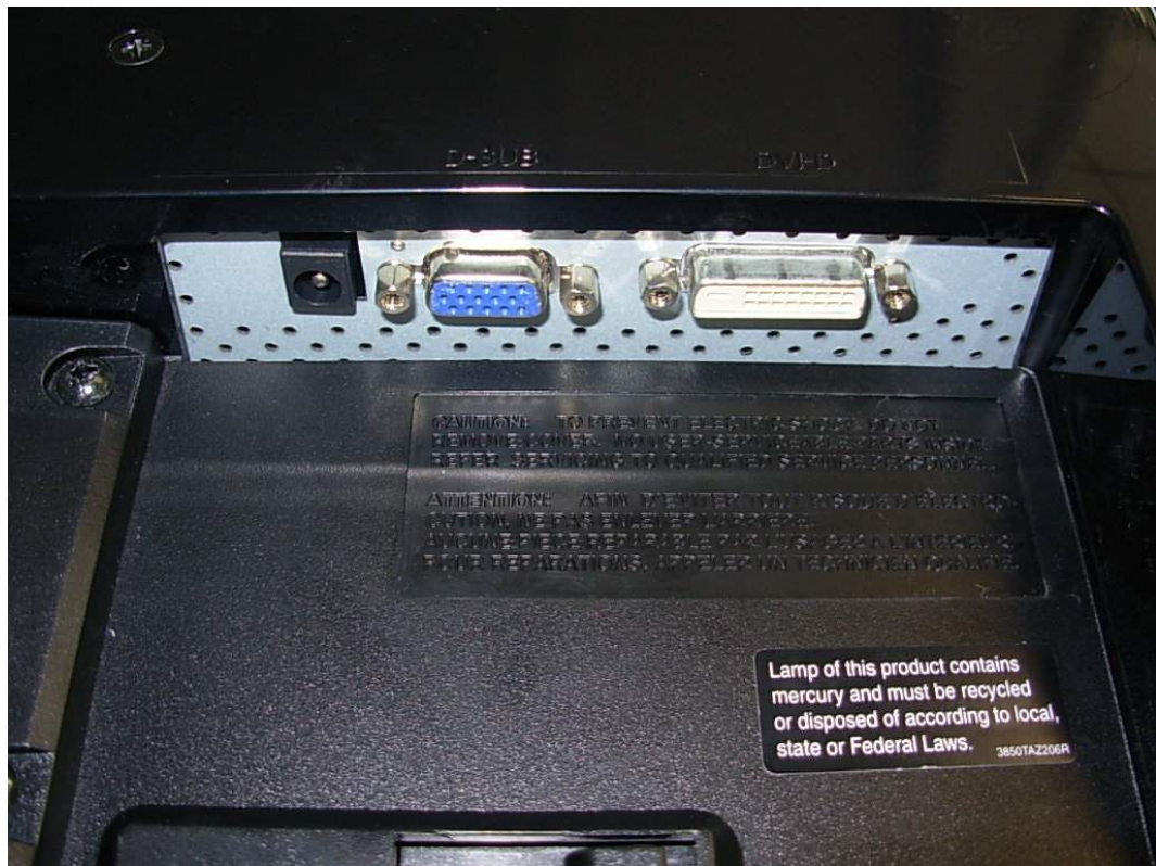
FIGURE 3 LCD MONITOR (M/N: L225WTM) PORTS
