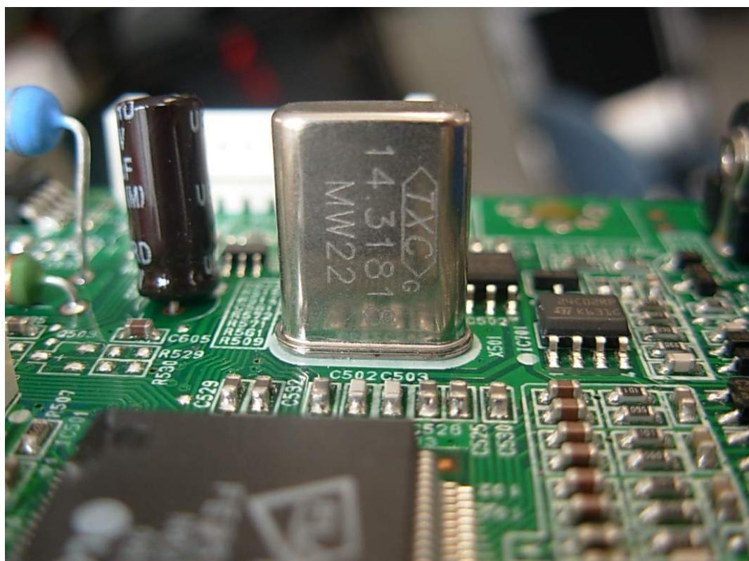
FIGURE 6 LCD MONITOR (M/N: L225WTM) CRYSTAL ON MAIN BOARD
