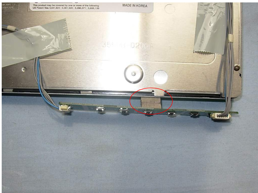
FIGURE 32 LCD MONITOR (M/N: L225WTM) DEBUG 1
