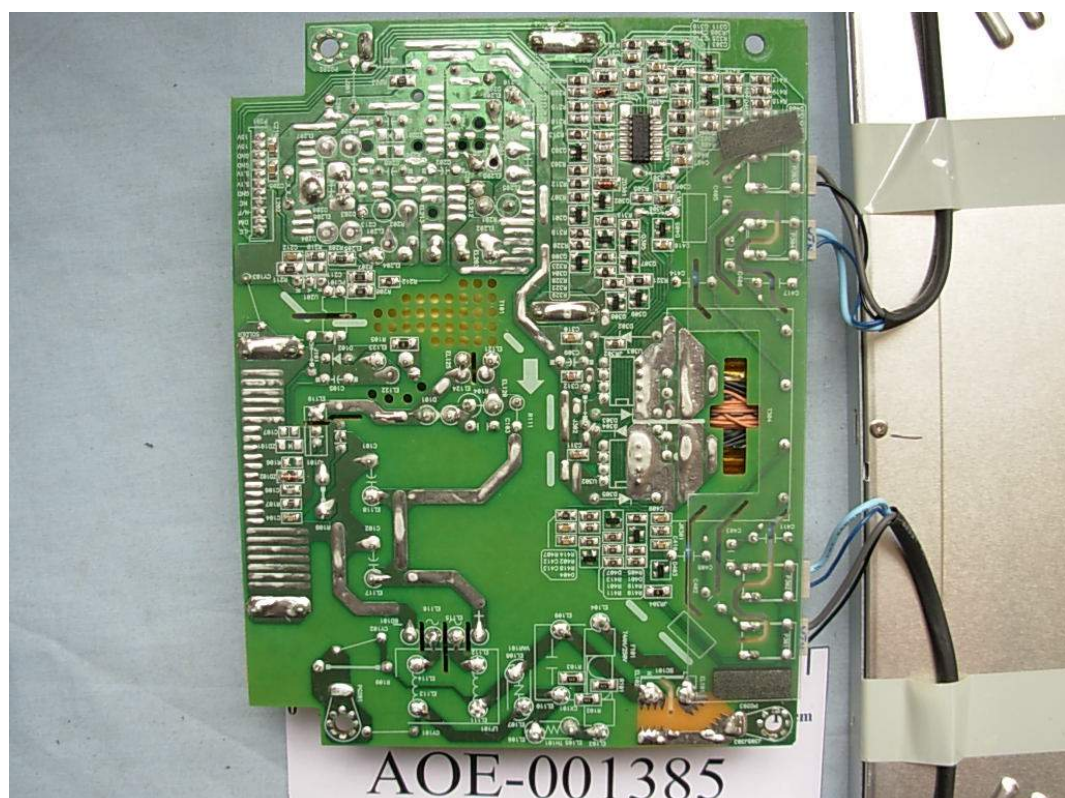
FIGURE 8 LCD MONITOR (M/N: L225WTM) POWER BOARD (SOLDERED SIDE)
