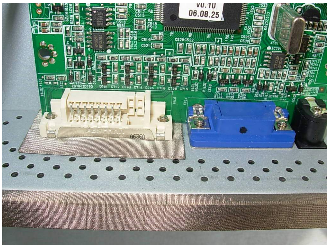
FIGURE 34 LCD MONITOR (M/N: L225WTM) DEBUG 3
