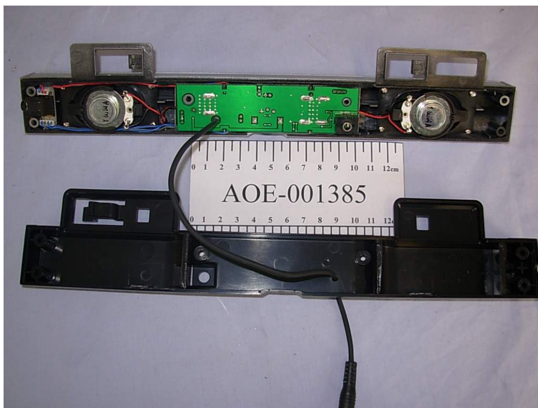
FIGURE 23 LCD MONITOR (M/N: L225WTM) SPEAKER COVER REMOVED
