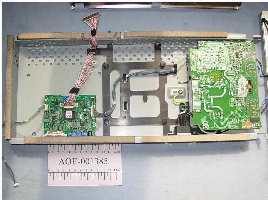
FIGURE 33 LCD MONITOR (M/N: L225WTM) DEBUG 2
