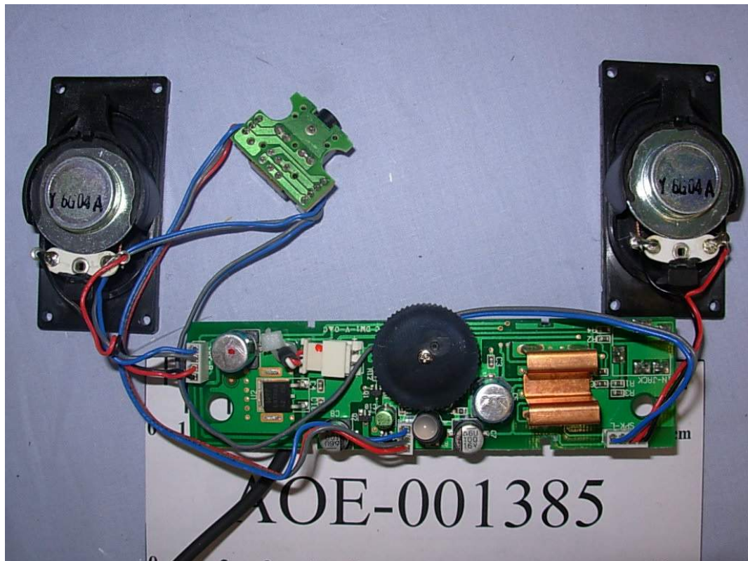
FIGURE 25 LCD MONITOR (M/N: L225WTM) SPEAKER BOARD&TRUMPET BACK
