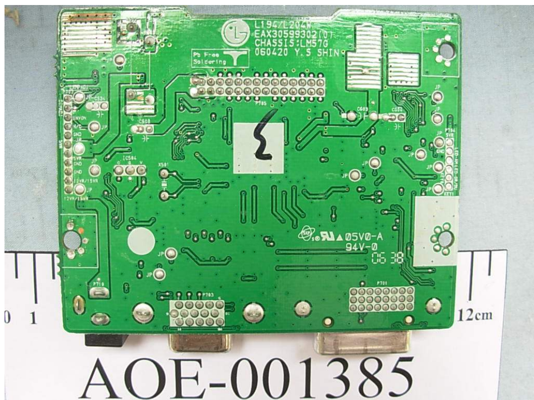
FIGURE 4 LCD MONITOR (M/N: L225WTM) MAIN BOARD (SOLDERED SIDE)
