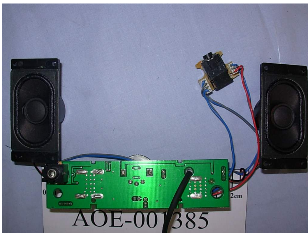
FIGURE 24 LCD MONITOR (M/N: L225WTM) SPEAKER BOARD & TRUMPET FRONT
