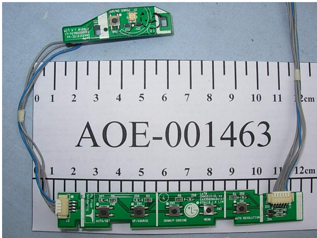
FIGURE 9 LCD MONITOR (M/N: L227WTS) LED & BUTTON BOARD (FRONT VIEW)
