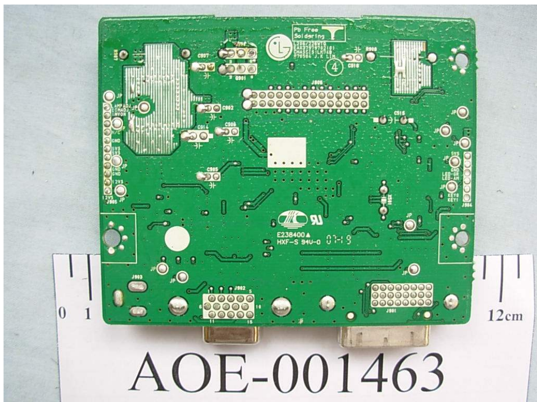
FIGURE 6 LCD MONITOR (M/N: L227WTS) MAIN BOARD (SOLDERED SIDE)
