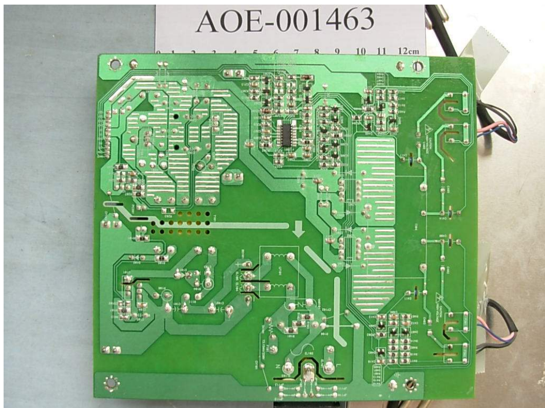
FIGURE 4 LCD MONITOR (M/N: L227WTS) POWER BOARD (SOLDERED SIDE)
