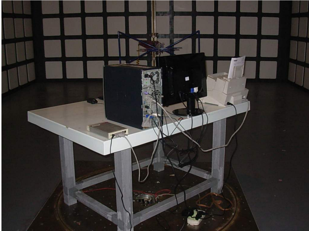
SETUP WITH MAXIMUM DETECTED EMISSION AT HORIZONTAL POLARIZATION (DVI 1680*1050@60Hz)
