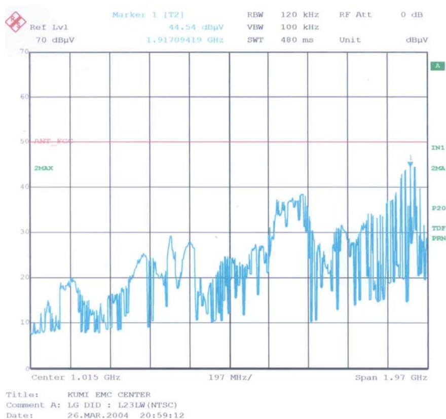
< Fig 7. Antenna power conduction result >
