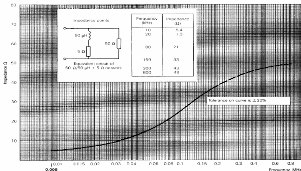
Fig 2. Impedance of LISN
