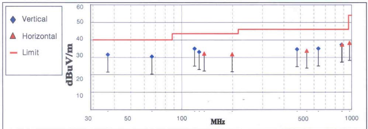
&lt; Fig 5. Radiated emission result &gt;
