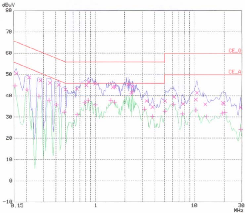
< Hot line >
