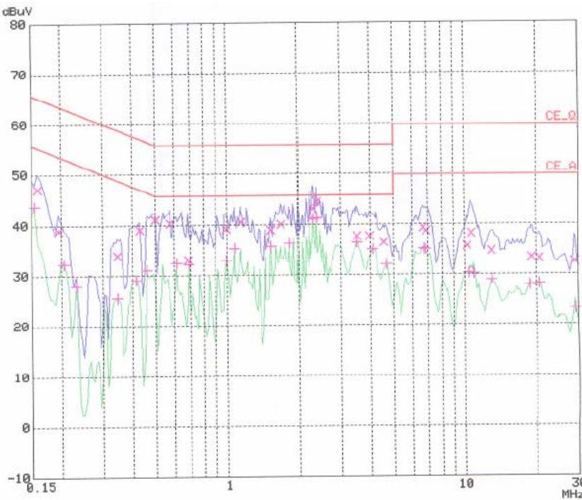
< Neutral line >
