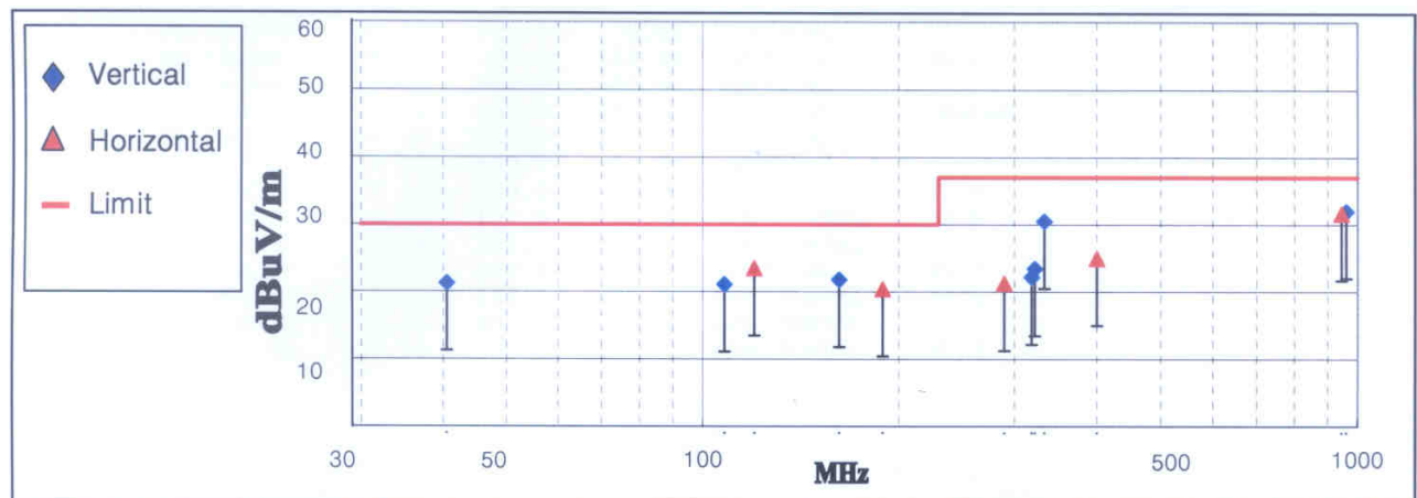
< Fig 4. Radiated Emission _ Analog(30MHz ~ 1000MHz) >
