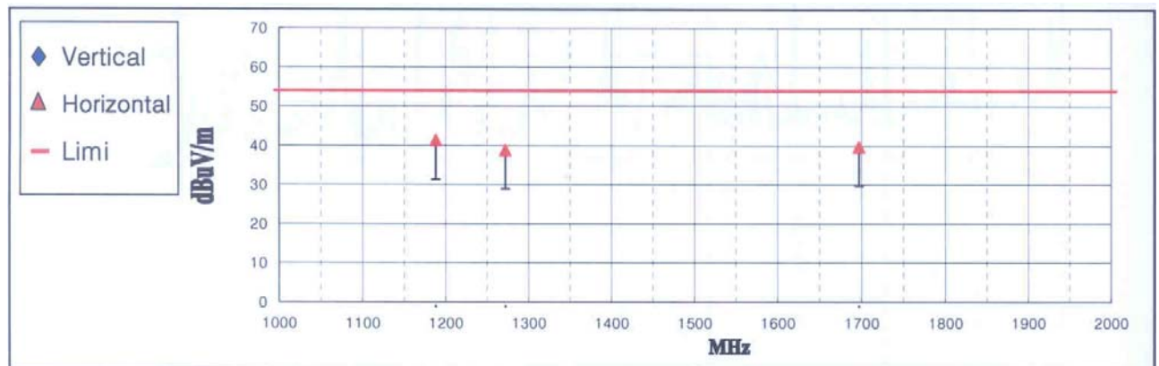
< Fig 5. Radiated Emission _ Analog(1000MHz ~ 2000MHz) >
