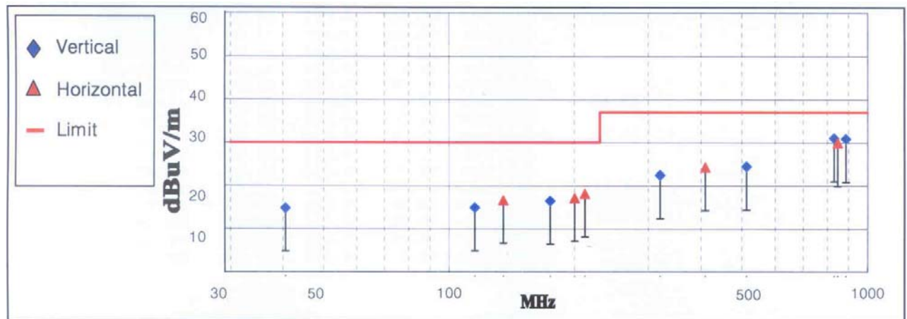
< Fig 6. Radiated Emission _ Digital(30MHz ~ 1000MHz) >
