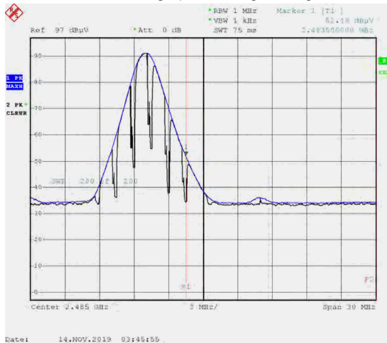
Radiated Restricted Band Edges plot – Peak Reading (8DPSK, Ch.78)
