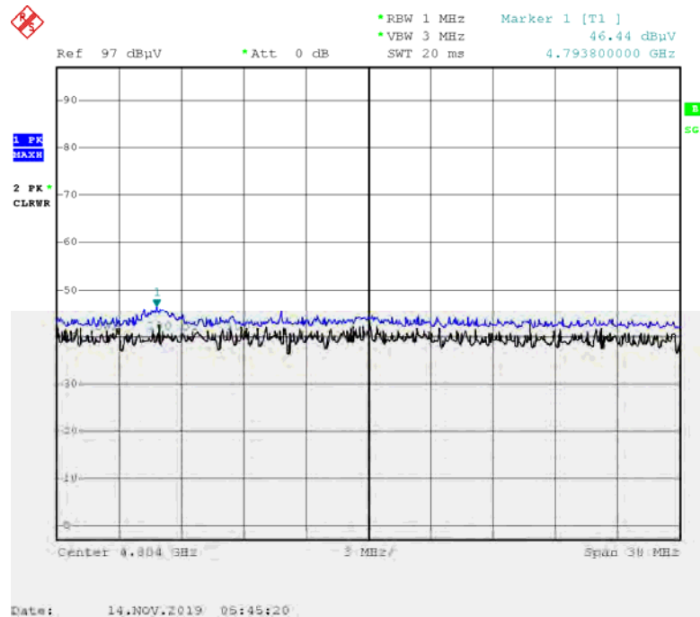
Radiated Spurious Emissions plot – Peak Reading (GFSK, Ch.0 2nd Harmonic)
