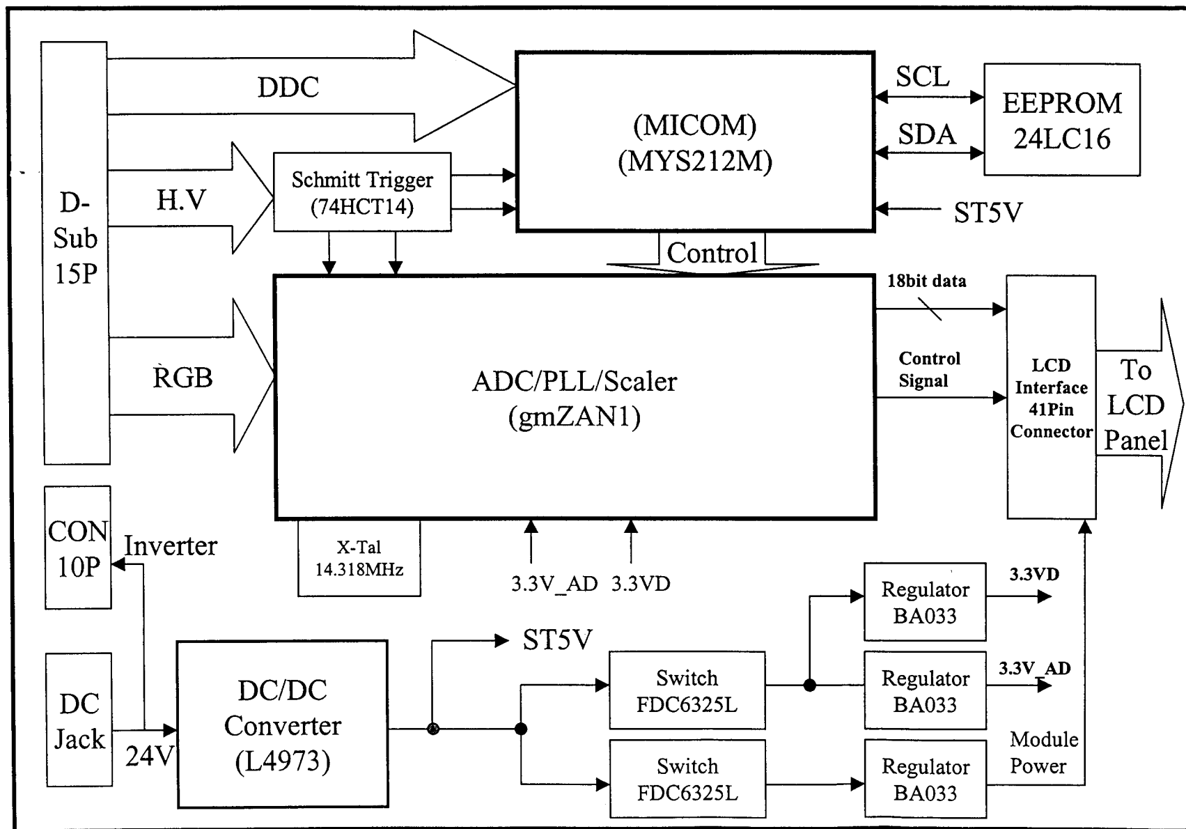
Block Diagram(LB570F)
