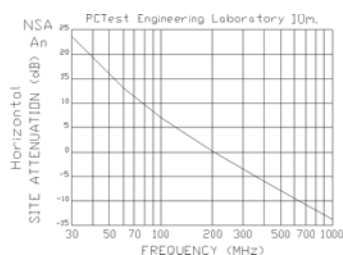
Fig. 5. NSA Theoretical Attenuation Curves (Horiz. Pol.)
