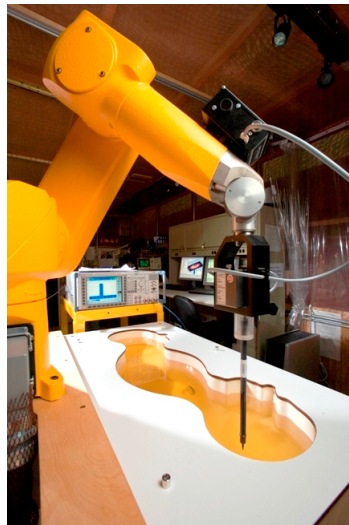
Figure 3-2 DASY4 SAR Measurement System
