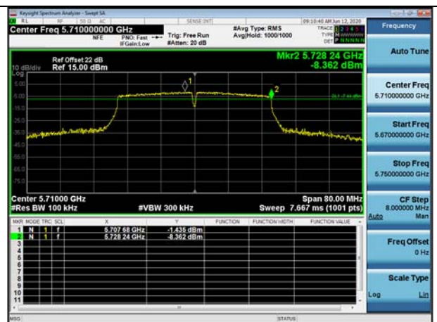
802.11ac_VHT40 CH.142
