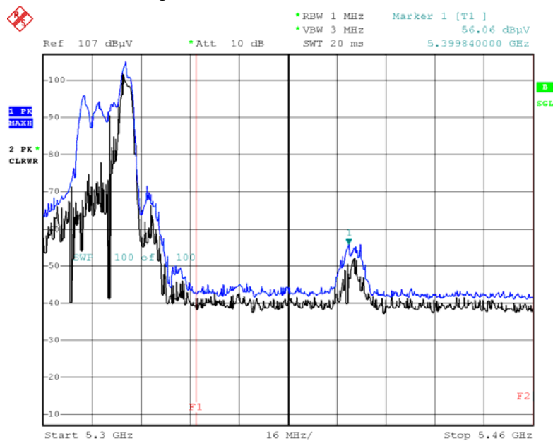
Peak Reading (802.11ax(HE80), Ch.58, X-H) - 52 T (RU 52)
