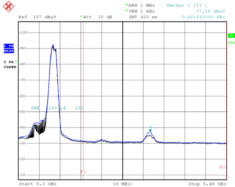
Average Reading (802.11ax(HE80), Ch.58, X-H) - 52 T (RU 52)
