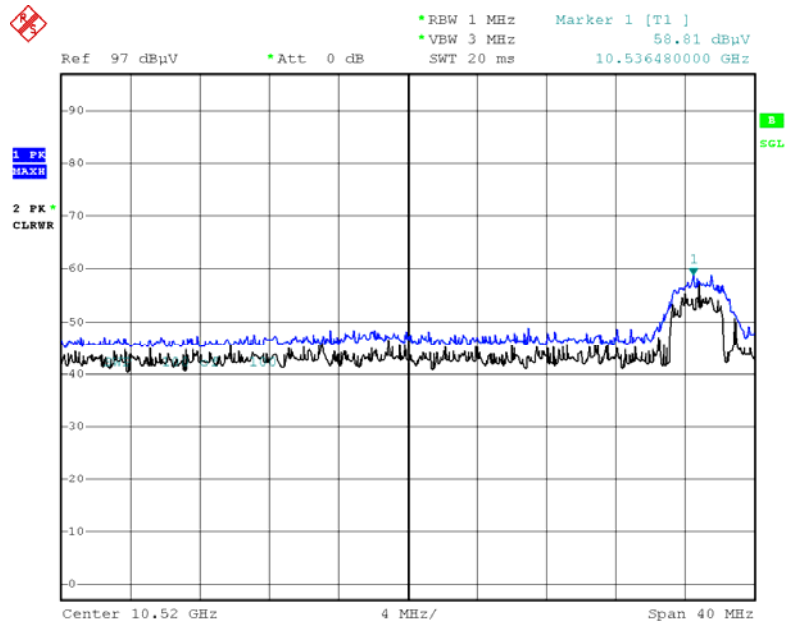
Peak Reading (802.11ax(HE20), Ch.52 2nd Harmonic, Z-V)_ Test case1
