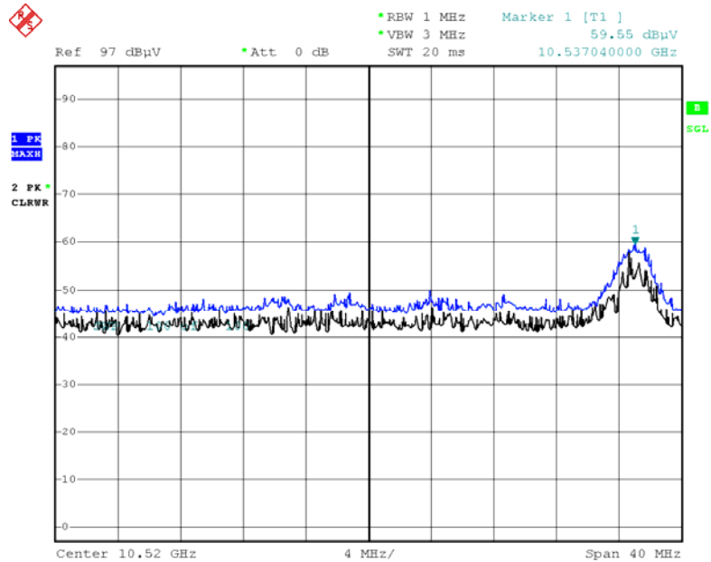
Peak Reading (802.11ax(HE20), Ch.52 2nd Harmonic, Z-H)_ Test case2
