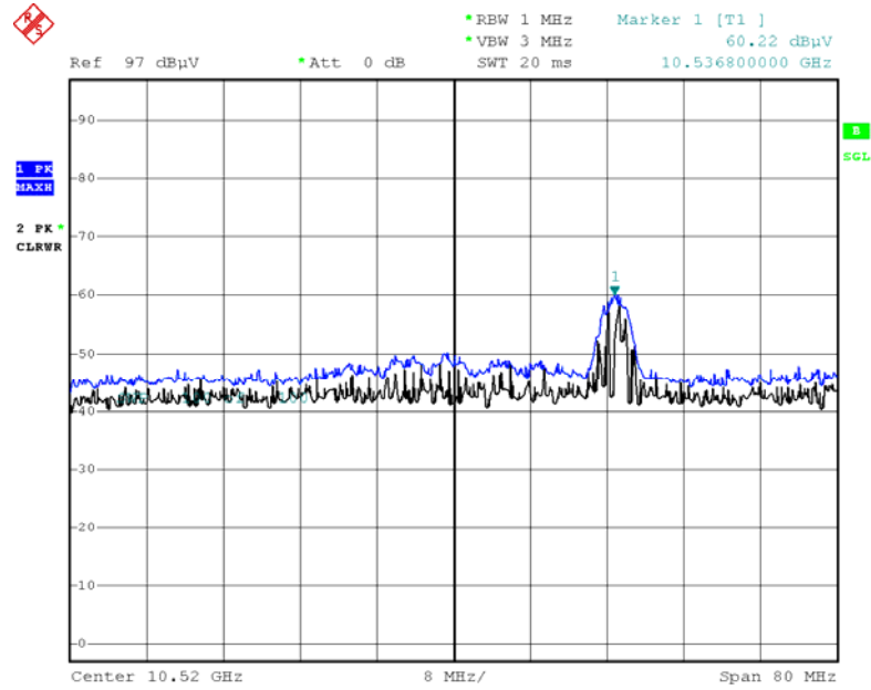
Peak Reading (802.11ax(HE20), Ch.52 2nd Harmonic, Z-H) - 26 T (RU 8)
