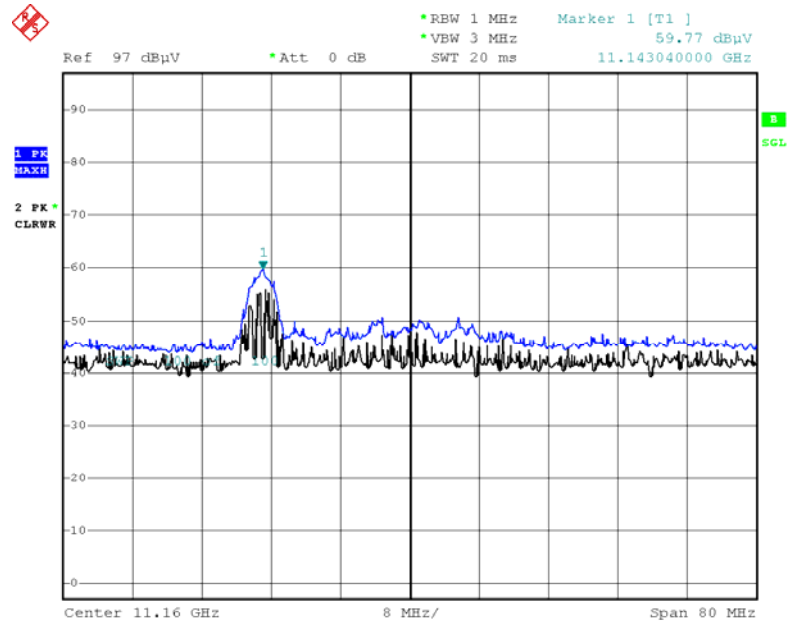
Peak Reading (802.11ax(HE20), Ch.116 2nd Harmonic, H) - 26 T (RU 0)
