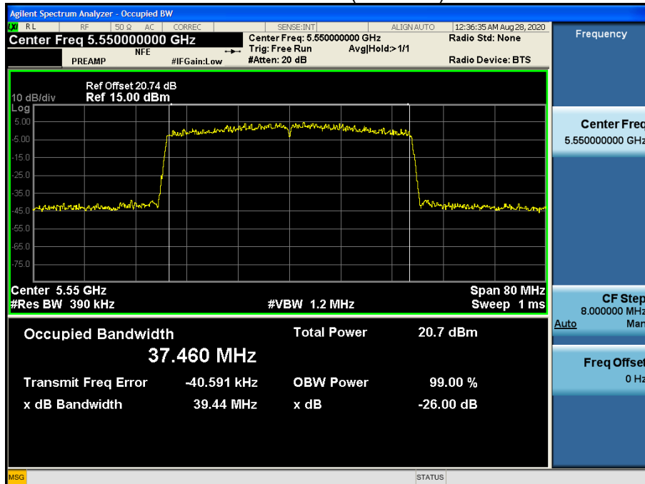
Bandwidth 40M Ch.110(5550MHz) RU 65
