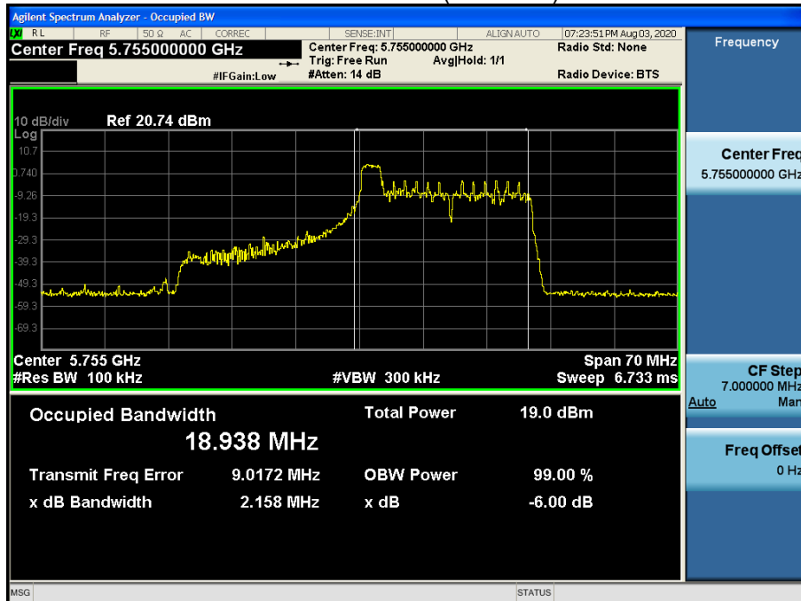
Bandwidth 40M Ch.151(5755MHz) RU 9
