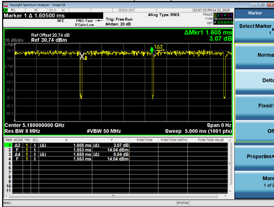
Bandwidth 20M Ch.36(5180MHz) 52Tone MCS0
