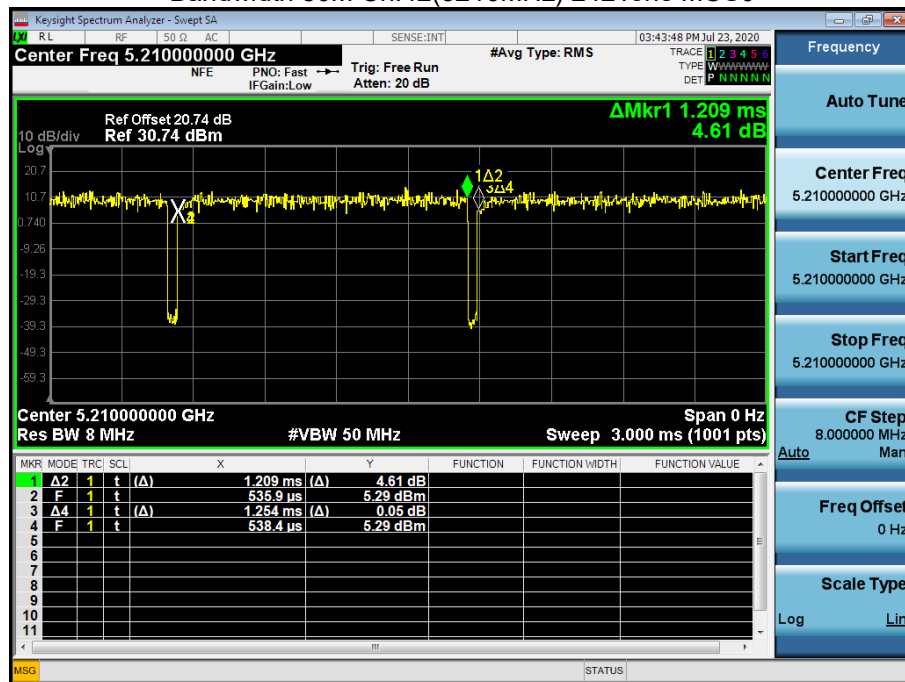
Bandwidth 80M Ch.42(5210MHz) 484Tone MCS0
