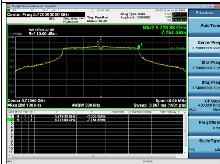
802.11ac_VHT20 CH.144
