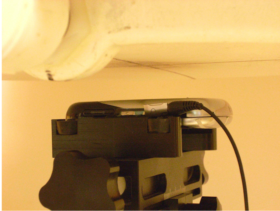
Figure 19-9 SAR Test Setup Photo 9
