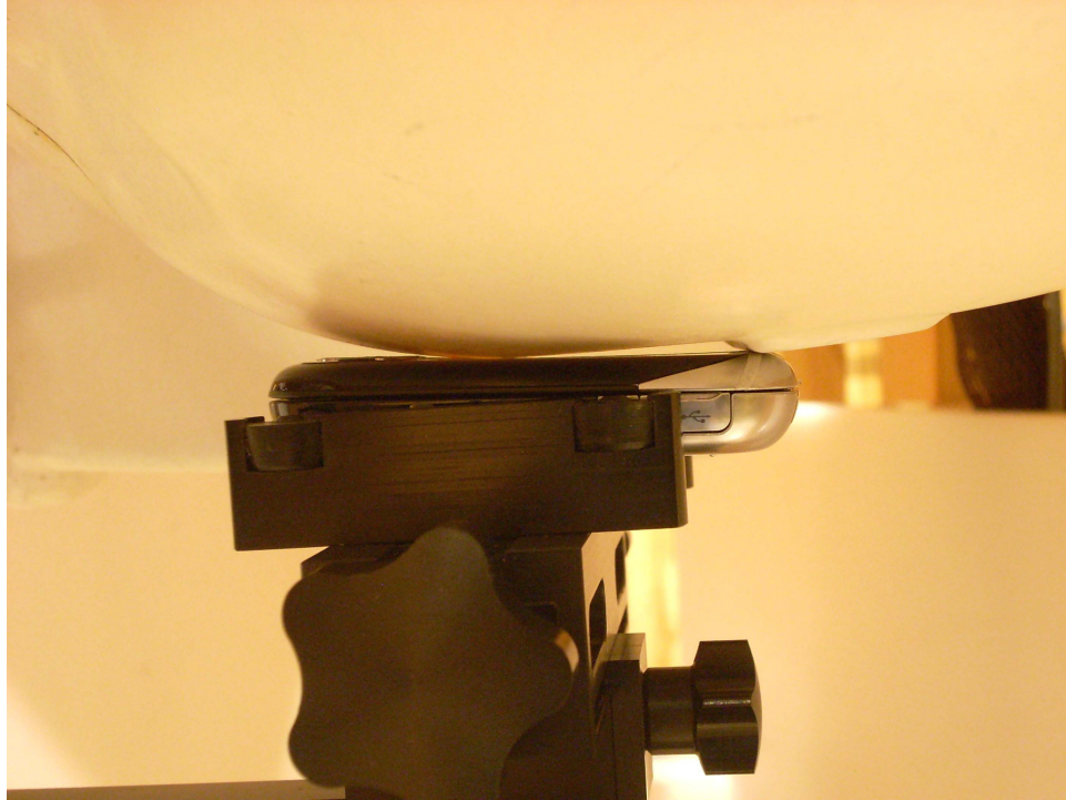
Figure 19-5 SAR Test Setup Photo 5
