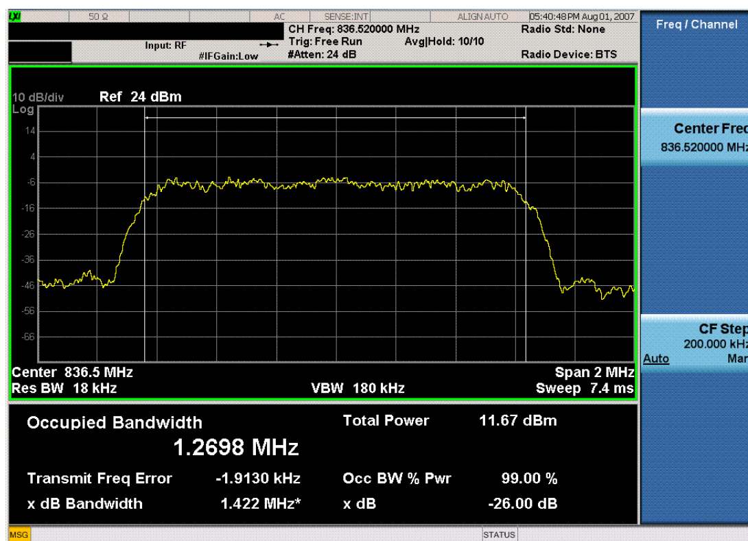
Plot 7-22. Occupied Bandwidth Plot (Cellular CDMA Mode – Ch. 384)
