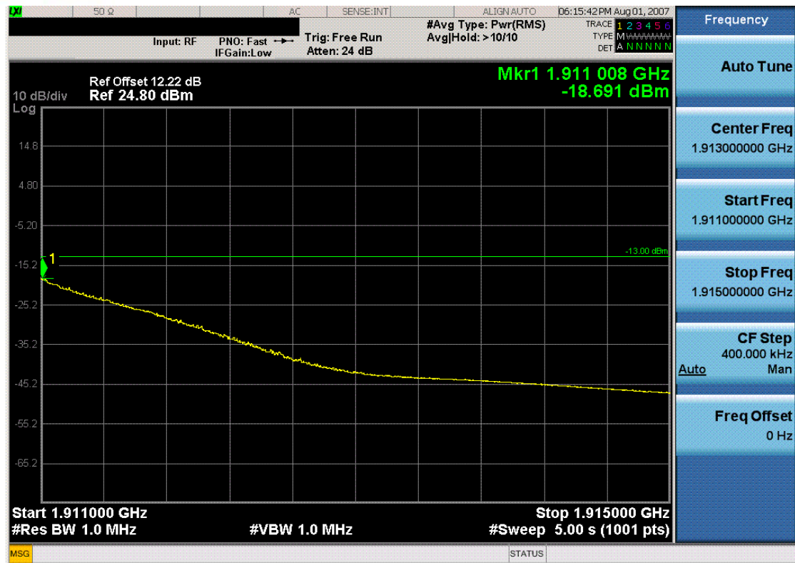
Plot 7-37. 4MHz Span Plot (PCS CDMA Mode – Ch. 1175)
