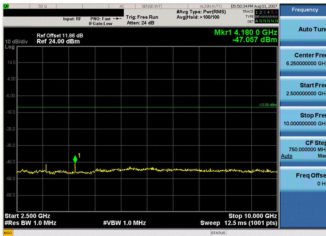
Plot 7-21. Conducted Spurious Plot (Cellular CDMA Mode – Ch. 384)
