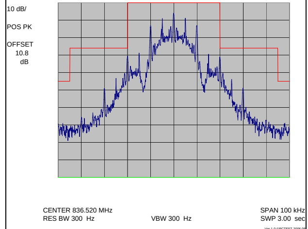
Plot 7-13. Wide Band Data Signal (WBD)
