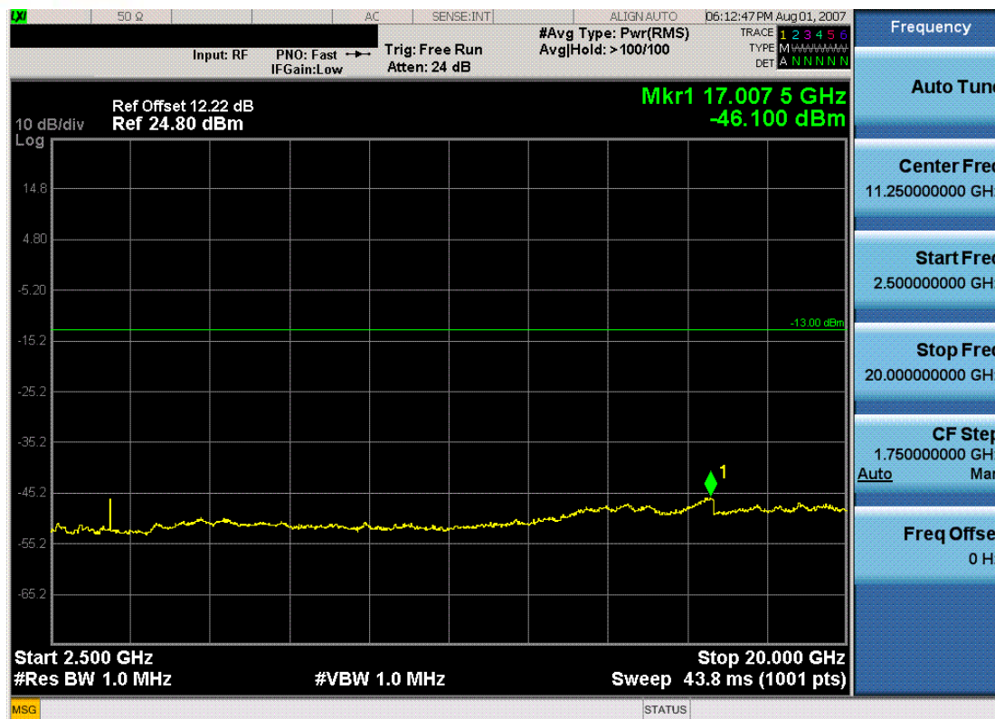
Plot 7-35. Conducted Spurious Plot (PCS CDMA Mode – Ch. 1175)
