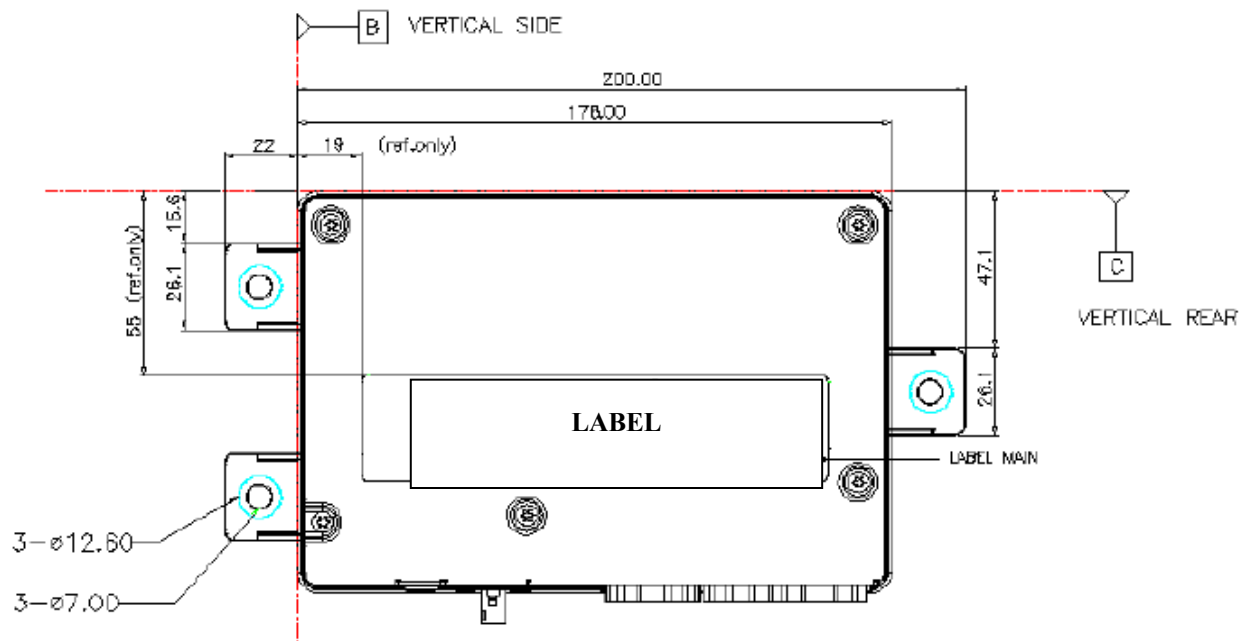
Figure 1.2 LABEL LOCATION
