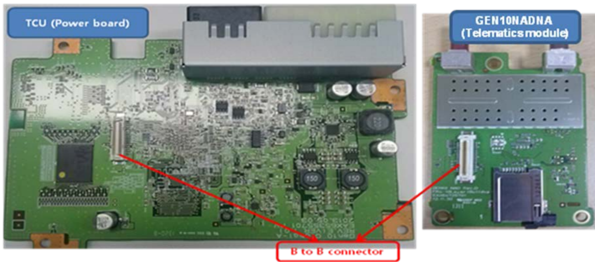
[Fig.1] VCP [module(NAD) + Power board(TCU)] setting information
