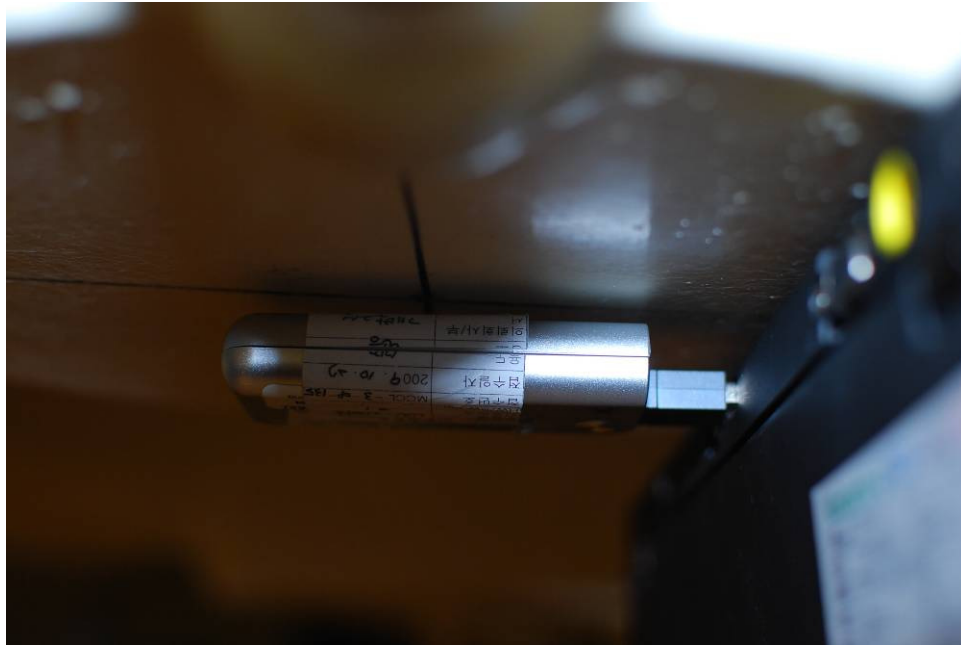
Figure 17-2 SAR Test Set Up Photo 2 Side B, Theta 180, Phi 180
