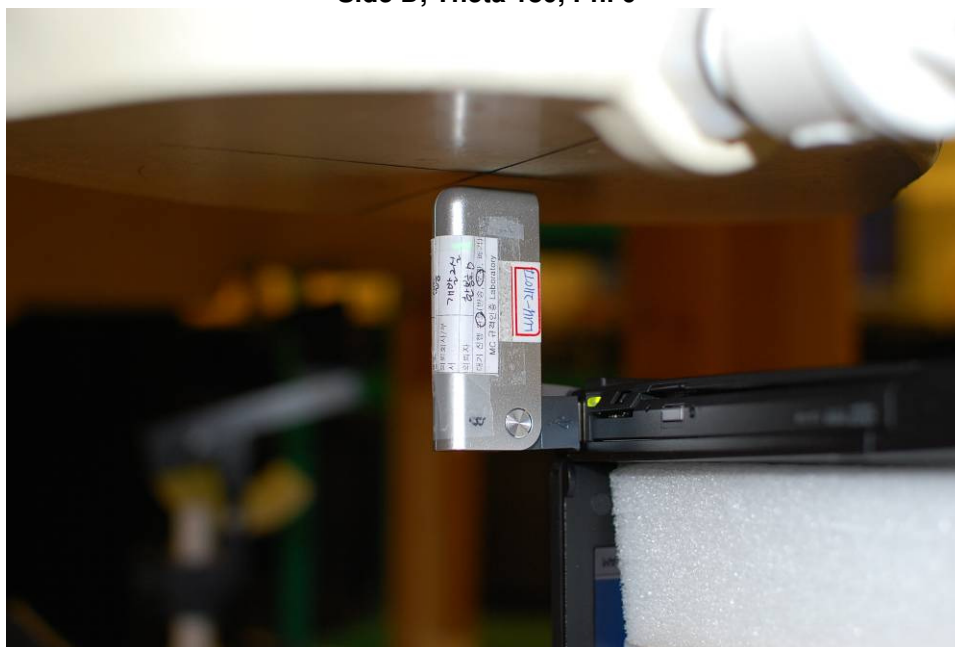
Figure 17-6 SAR Test Set Up Photo 6 Top Rounded Edge, Theta 90, Phi 0
