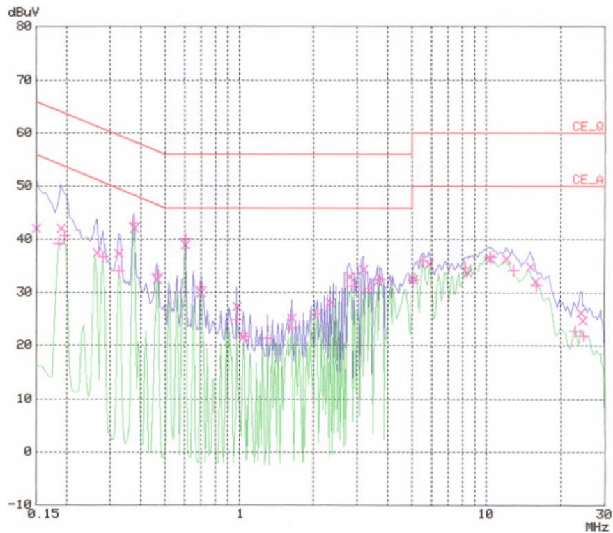
< Hot line >
