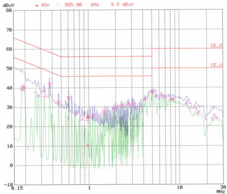
< Neutral line >
