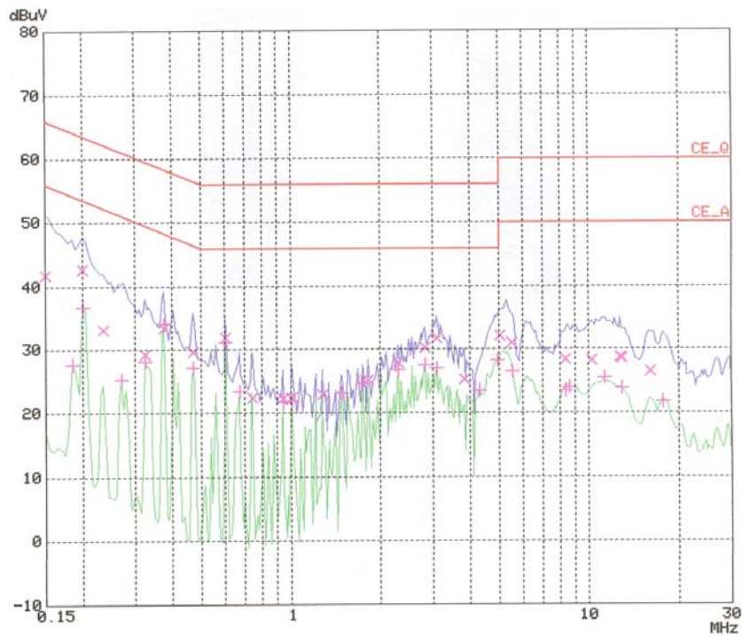
< Hot line >
