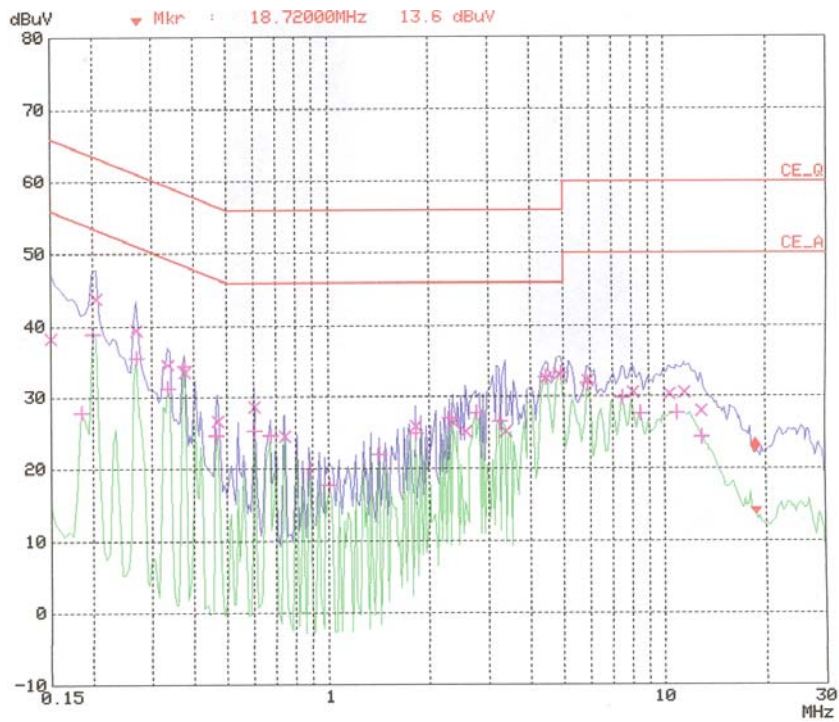
< Neutral line >
