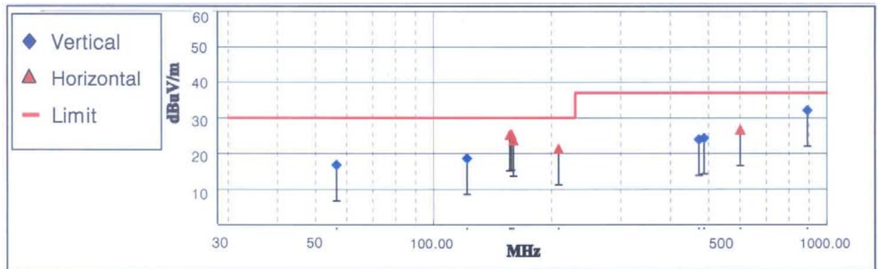
< Fig 6. Radiated Emission _ Digital (30MHz ~ 1000MHz) >
