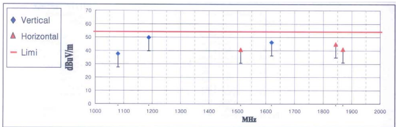
Fig 5. Radiated Emission _ Analog (1000MHz ~ 2000MHz) >
