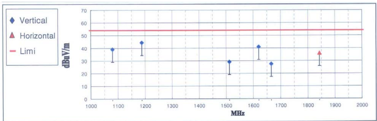
< Fig 7. Radiated Emission _ Digital (1000MHz ~ 2000MHz) >
