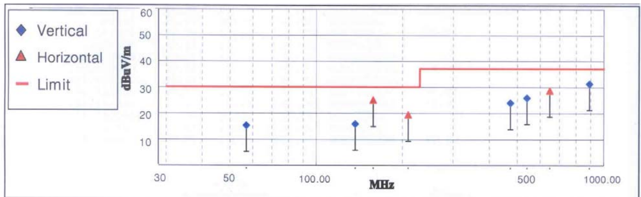
Fig 4. Radiated Emission _ Analog (30MHz ~ 1000MHz) >
