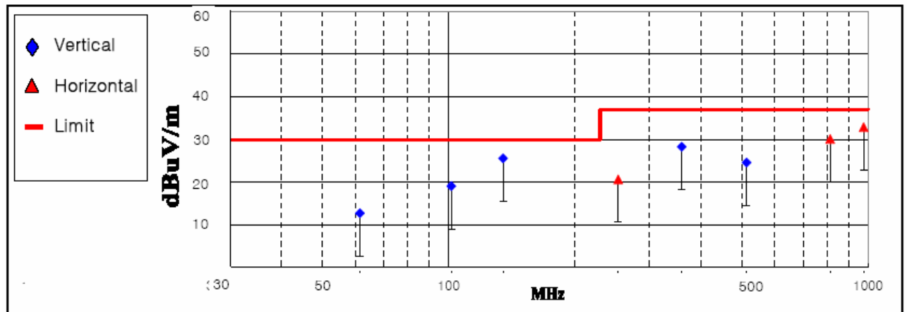
&lt; Fig 6. Radiated emission result (30MHz ~ 1000MHz)&gt;
