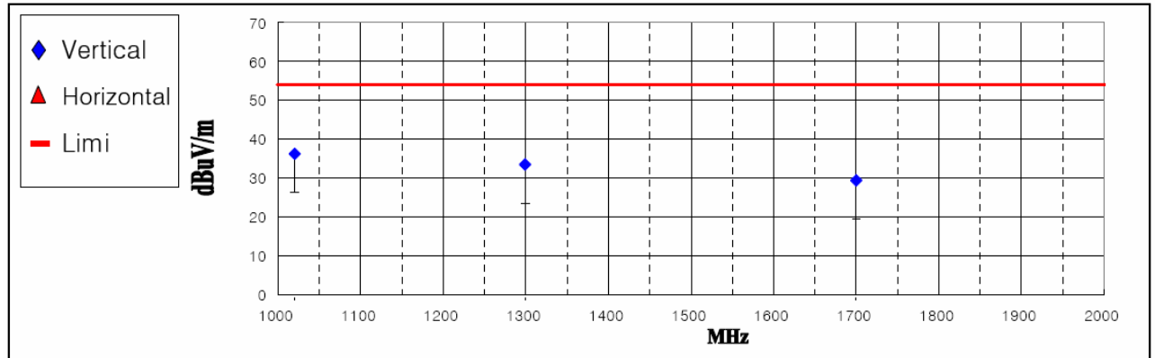
&lt; Fig 6. Radiated emission result (1000MHz ~ 2000MHz)&gt;
