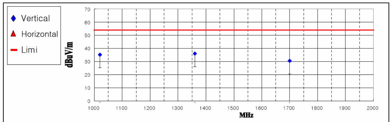
&lt; Fig 7. Radiated emission result (1000MHz ~ 2000MHz)&gt;
