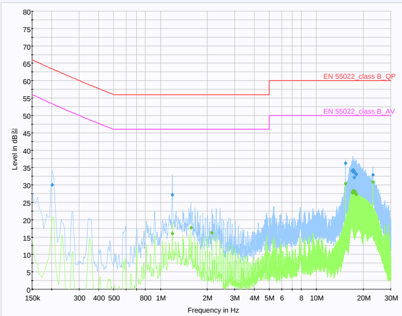
< Hot line >
