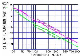
Figure 9. Normalized Site Attenuation Curves (H&V)
