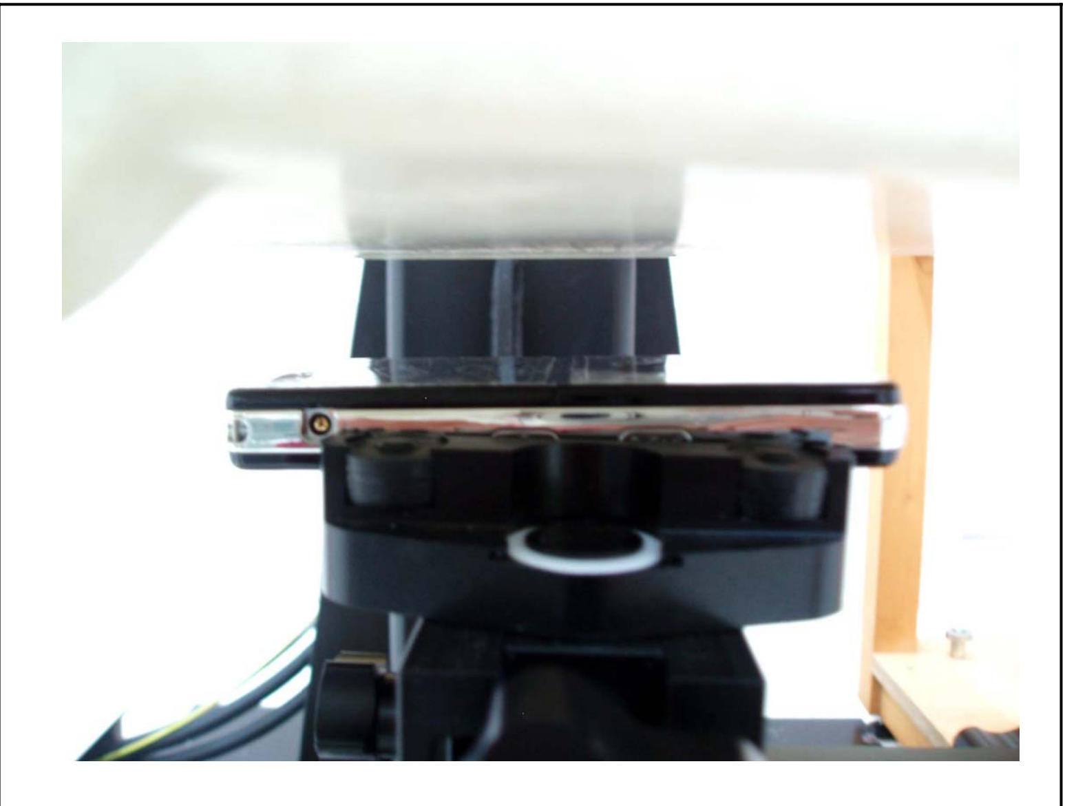
Figure 15 Body SAR Test Setup – w/o Holster
