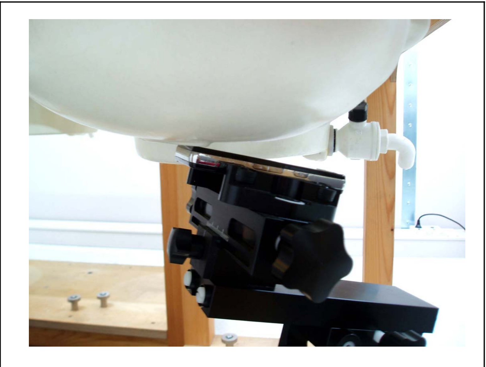
Figure 6 Right Head SAR Test Setup – Ear Tilt Position
