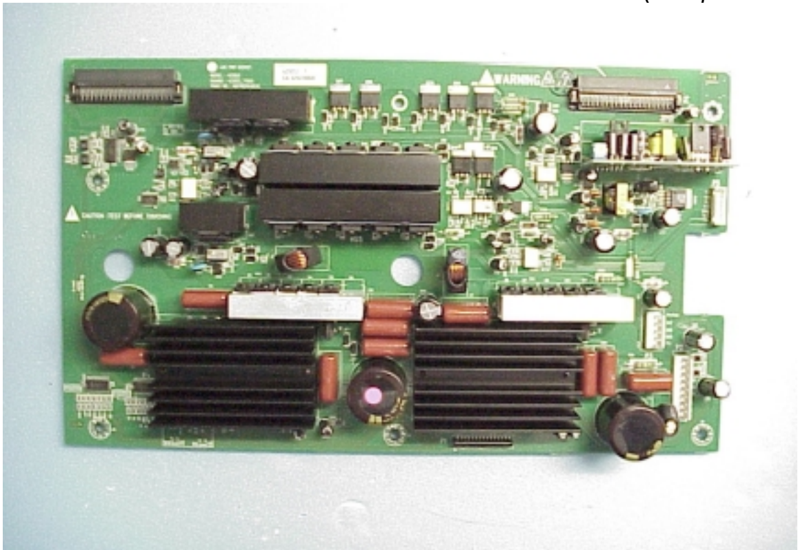
Figure 11 Y Board (Component Side)
