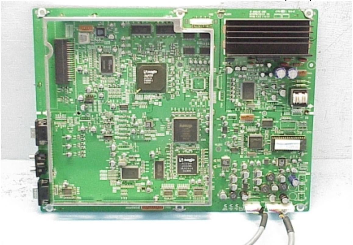
Figure 14 Main Board (Component Side)
