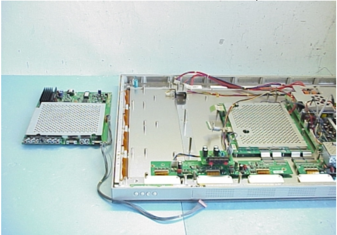
Figure 13 Internal Frame (Removed Main PCB)
