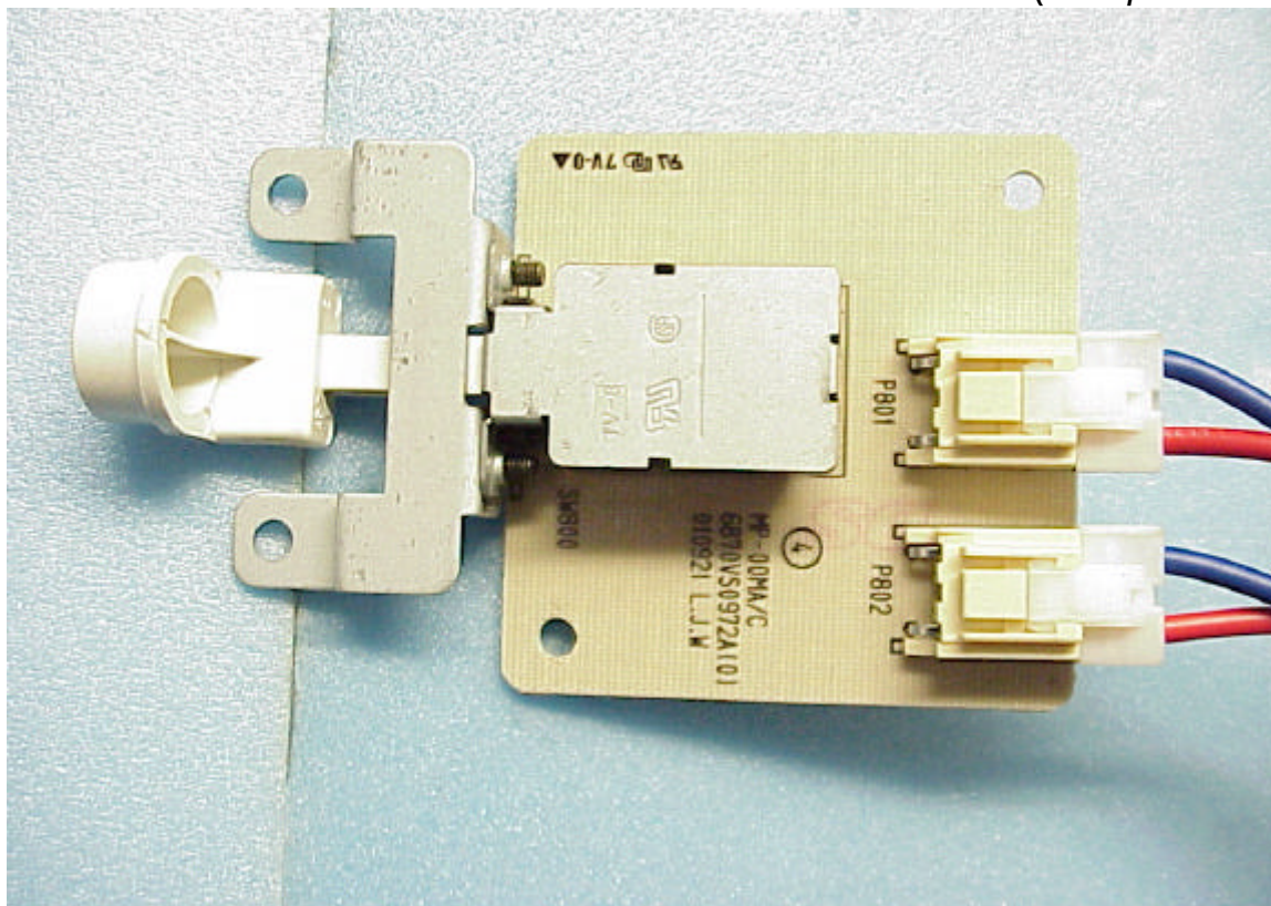
Figure 26 Switch Board (Component Side)
