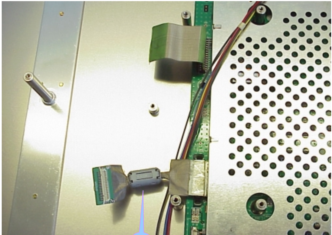
Figure 7 Internal Frame
