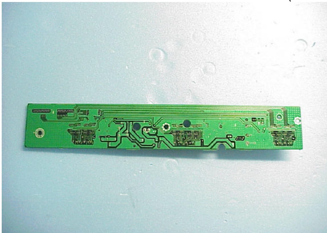
Figure 25 X-Drive Board (Solder Side)
