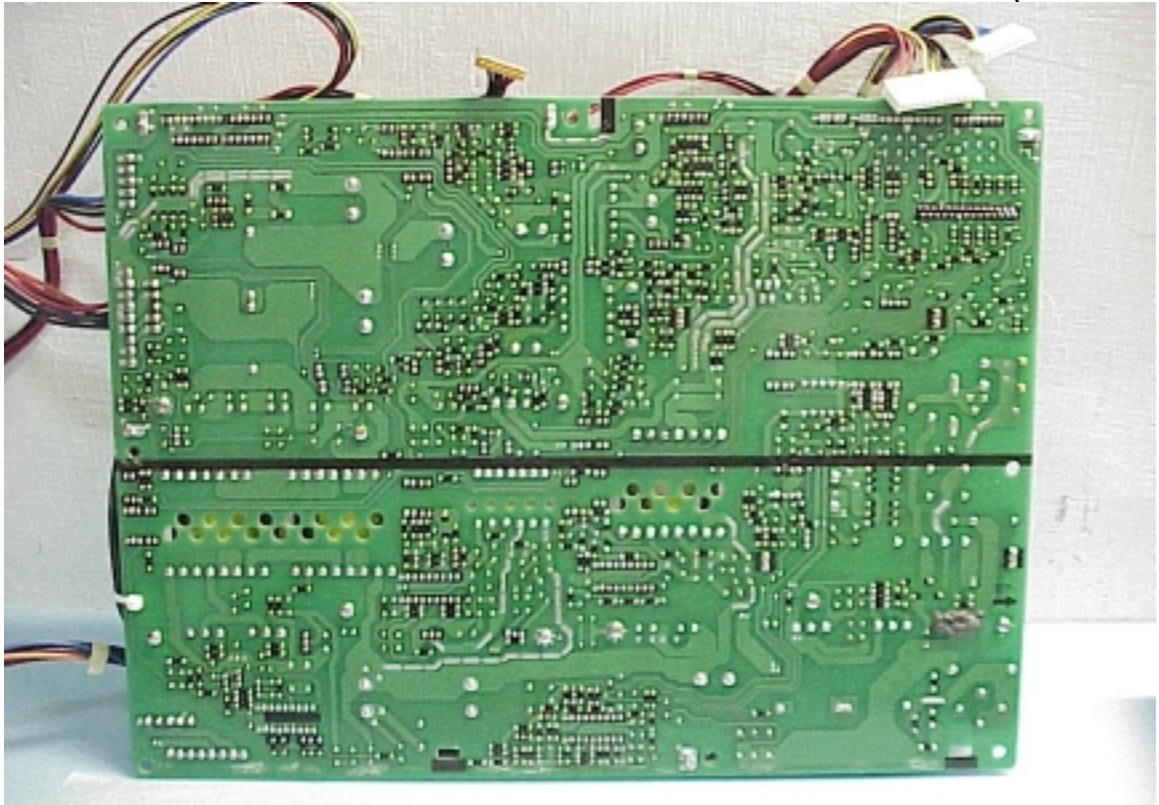
Figure 19 Power Board (Solder Side)
