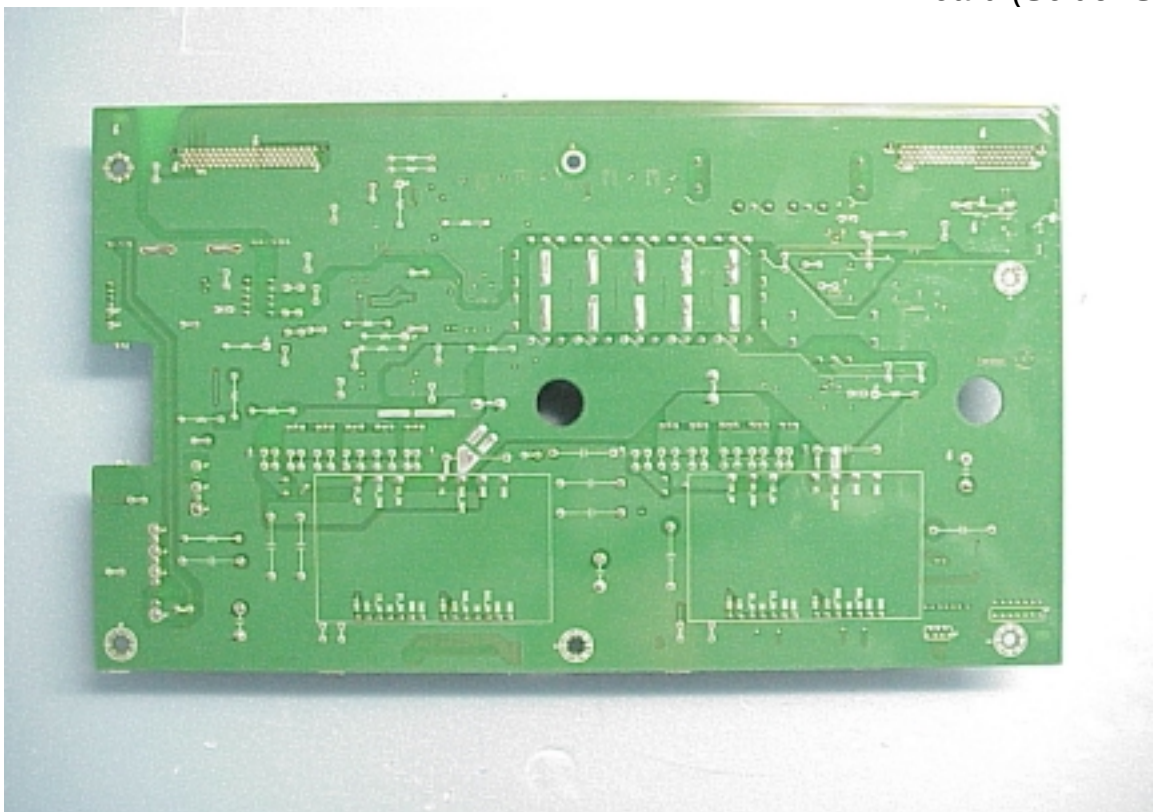
Figure 12 Y Board (Solder Side)
