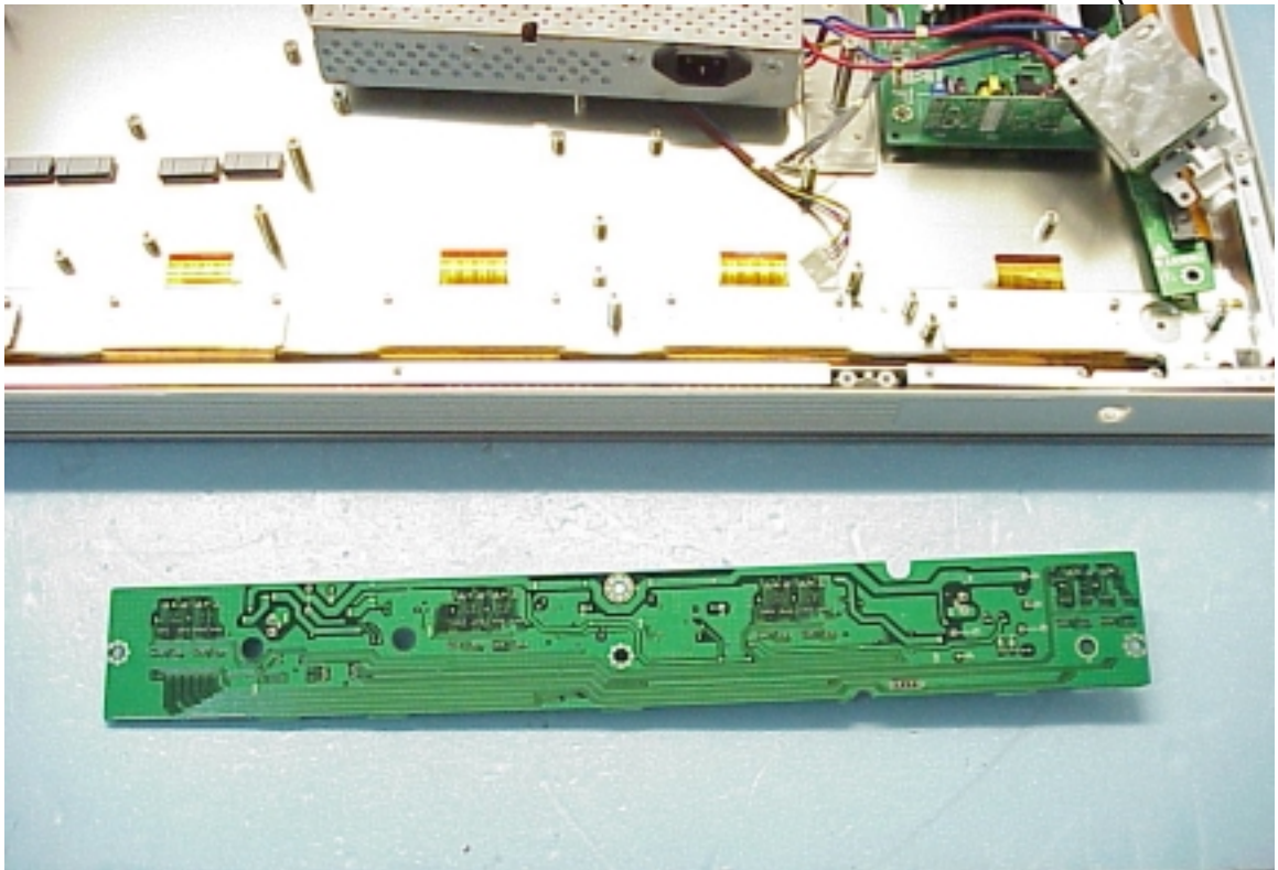
Figure 23 X-Drive Board (Solder Side)
