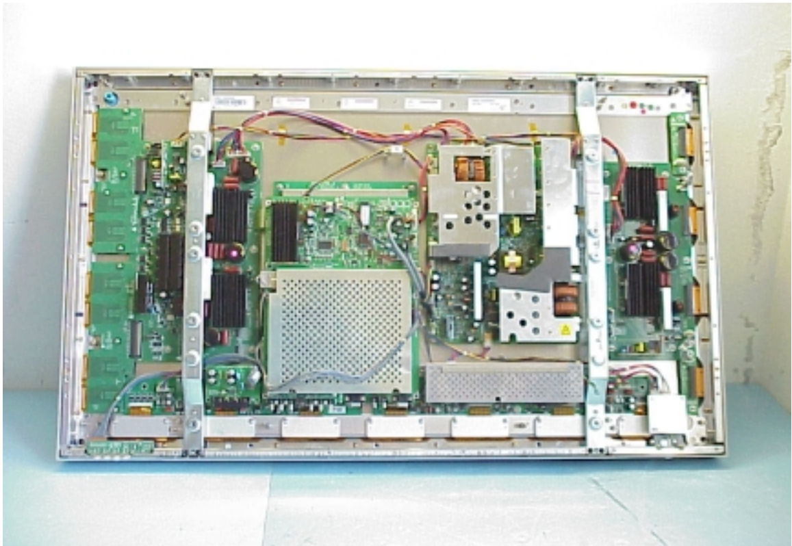
Figure 5 Internal View
