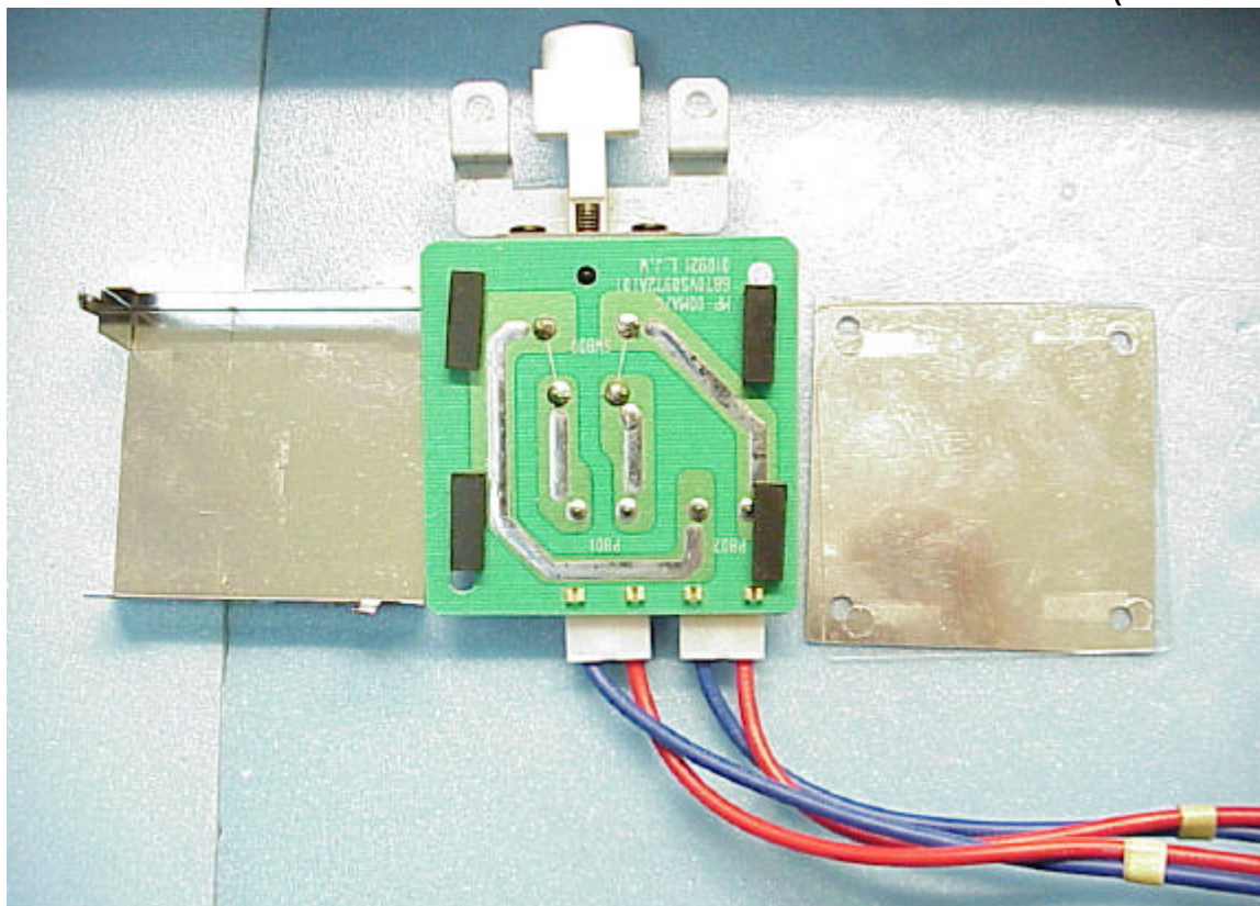
Figure 27 Switch Board (Solder Side)
