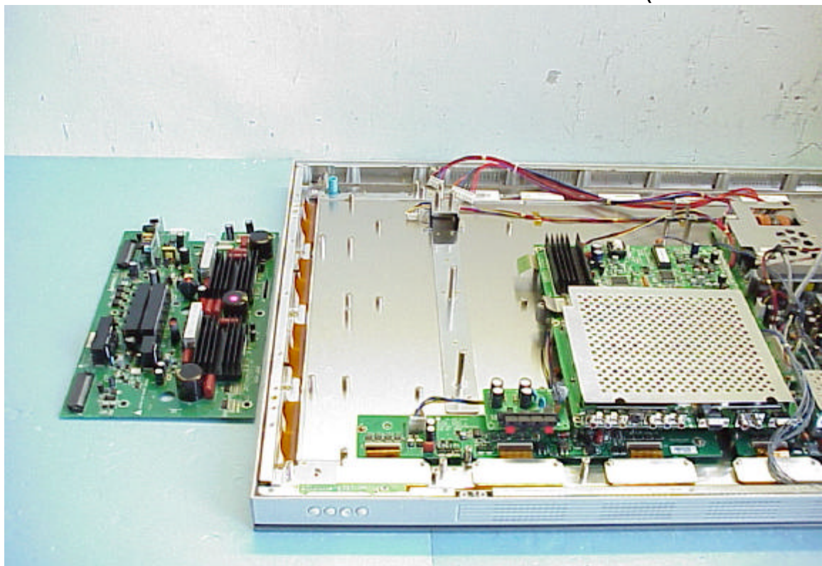
Figure 10 Internal Frame (Removed Y Board)
