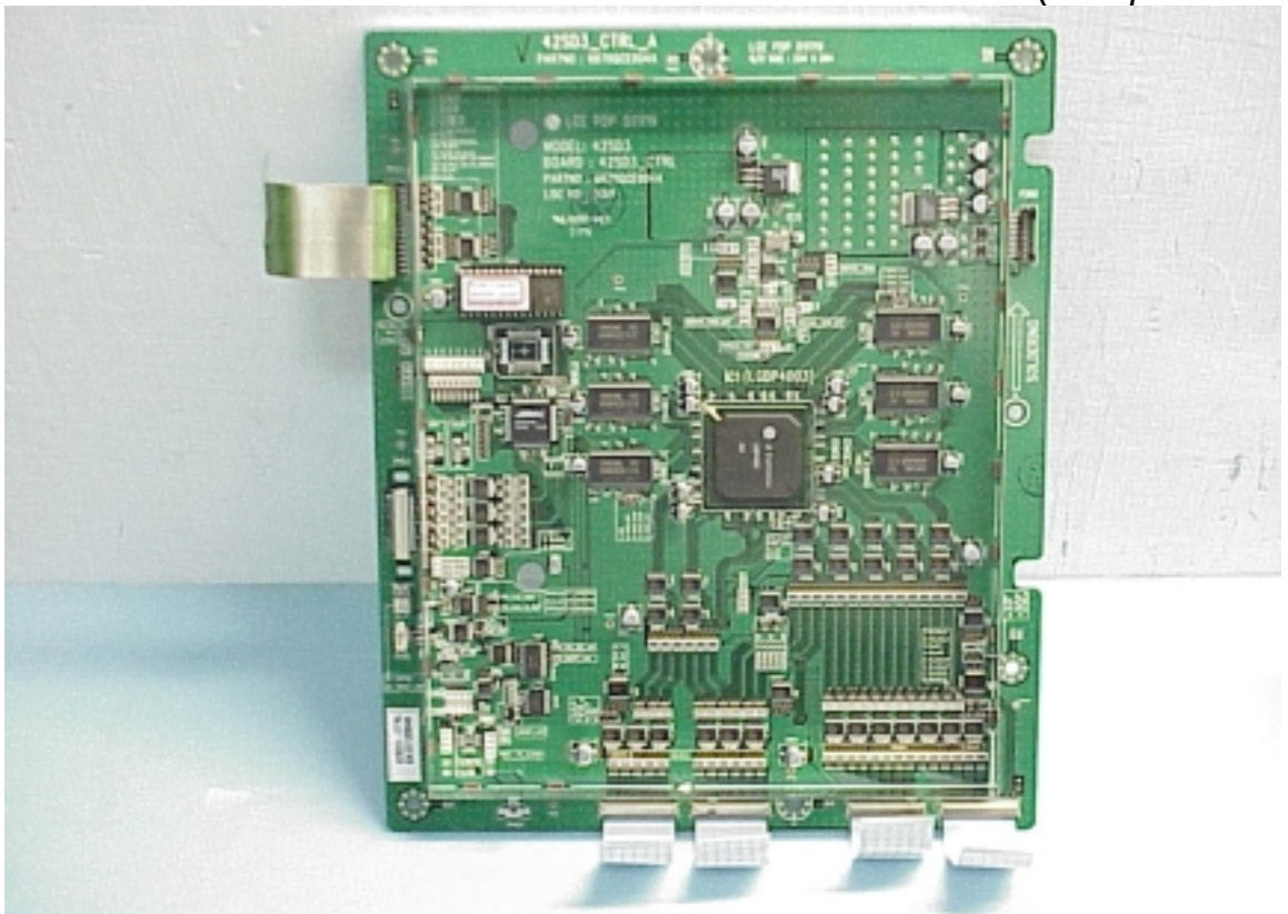
Figure 16 Control Board (Component Side)
