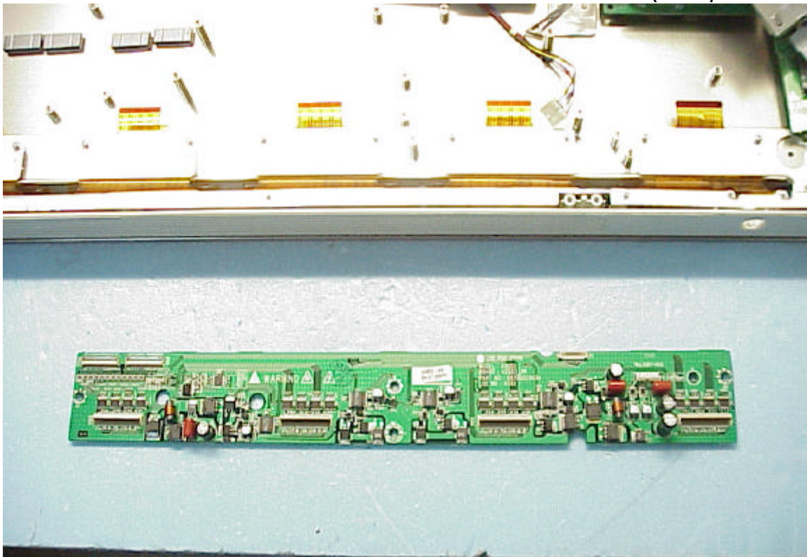
Figure 22 X-Drive Board (Component Side)
