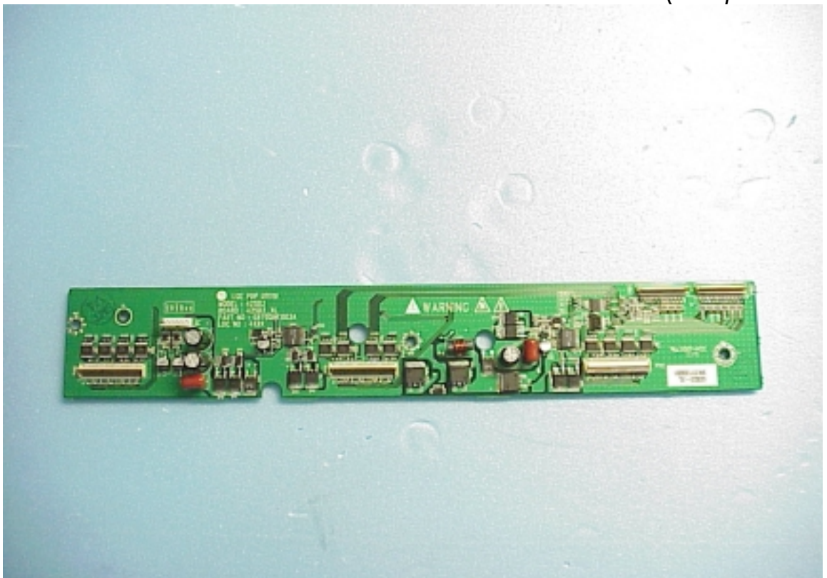
Figure 24 X-Drive Board (Component Side)
