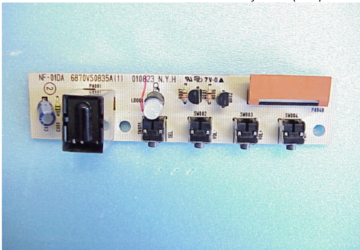
Figure 28 Control Key Board (Component Side)
