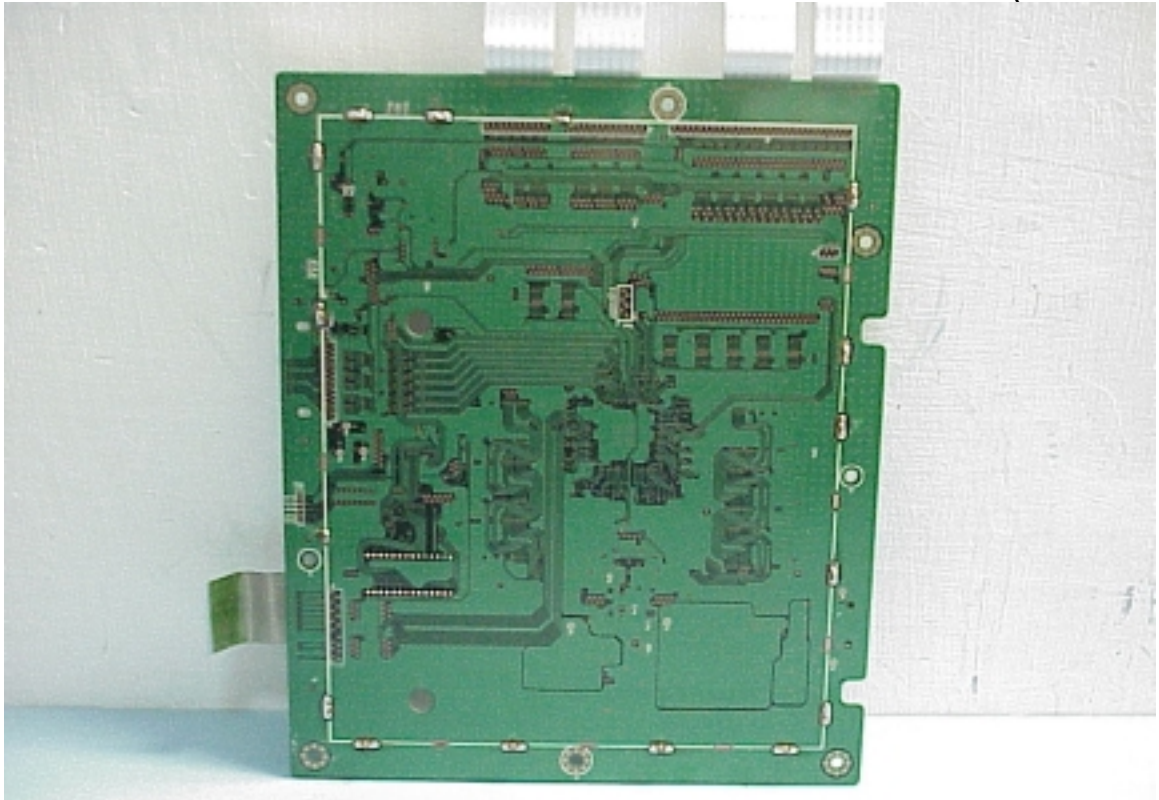
Figure 17 Control Board (Solder Side)
