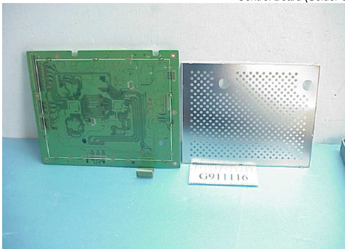
Figure 26 Control Board (Solder Side)
