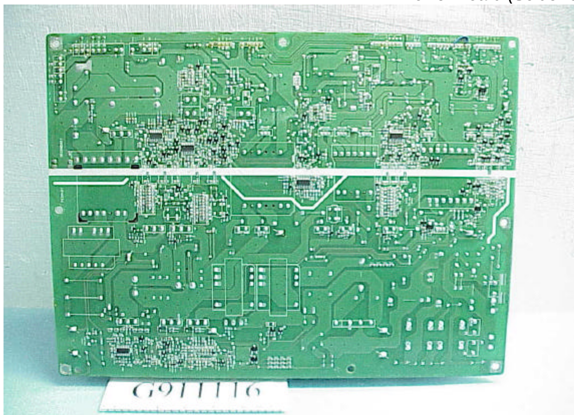
Figure 29 Power Board (Solder Side)
