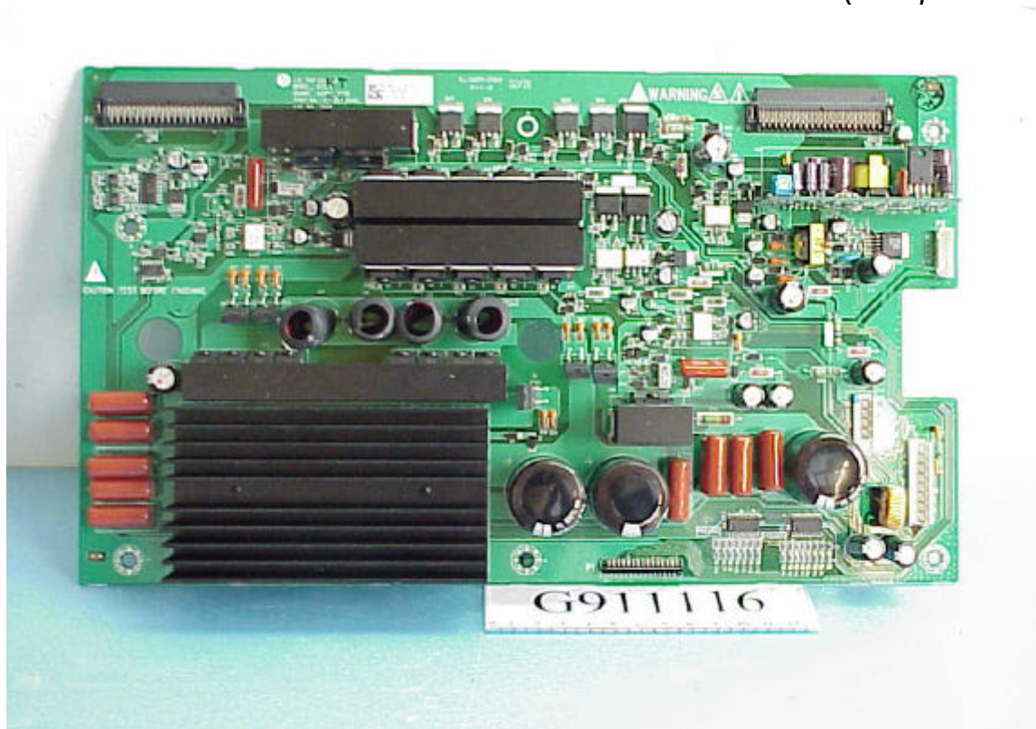
Figure 20 Y Board (Component Side)
