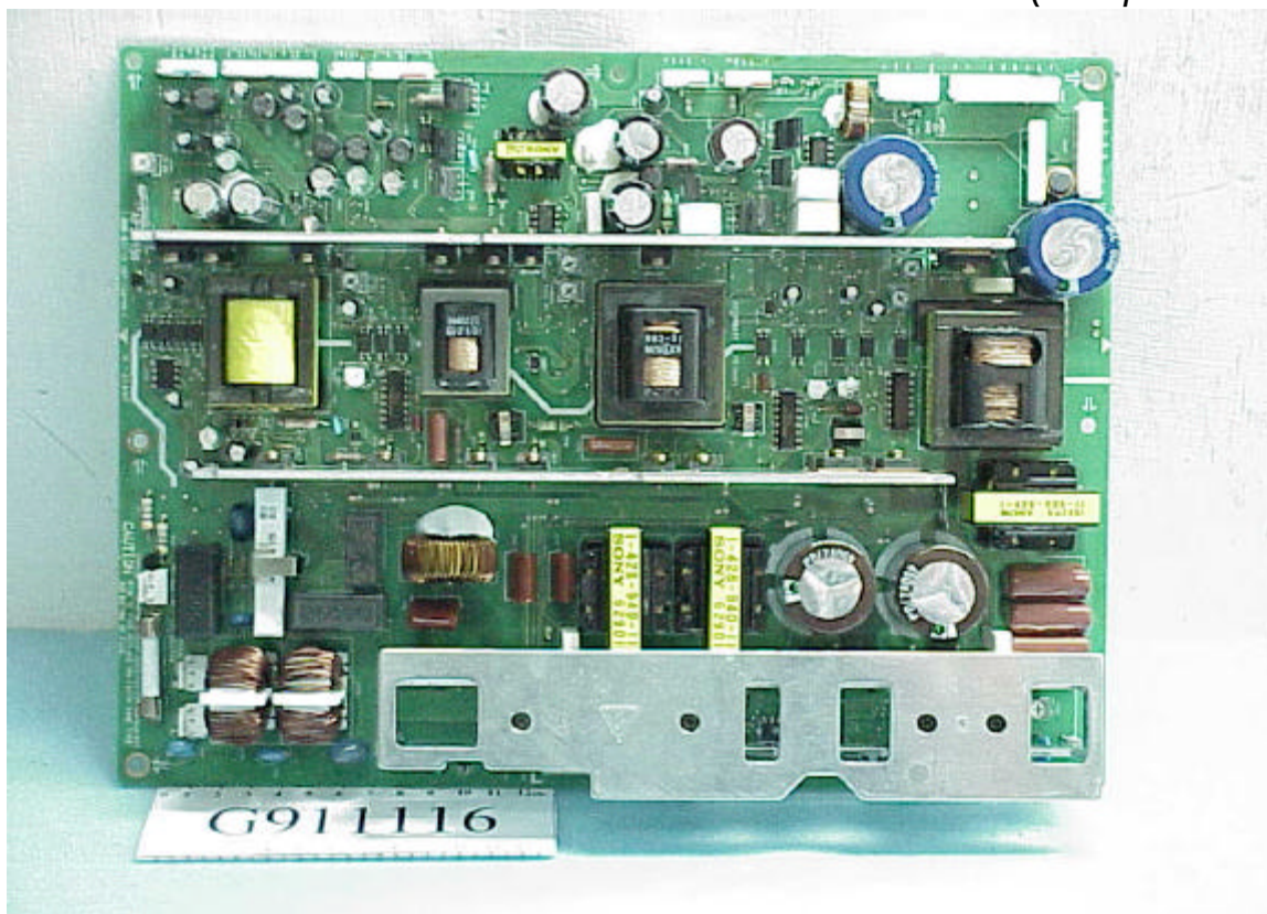
Figure 28 Power Board (Component Side)
