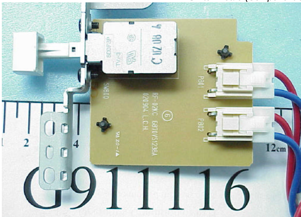
Figure 30 Switch Board (Component Side)
