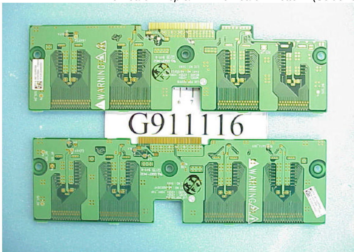
Figure 19 Y Drive Board – Top & Y Drive Board – Bottom (Solder Side)
