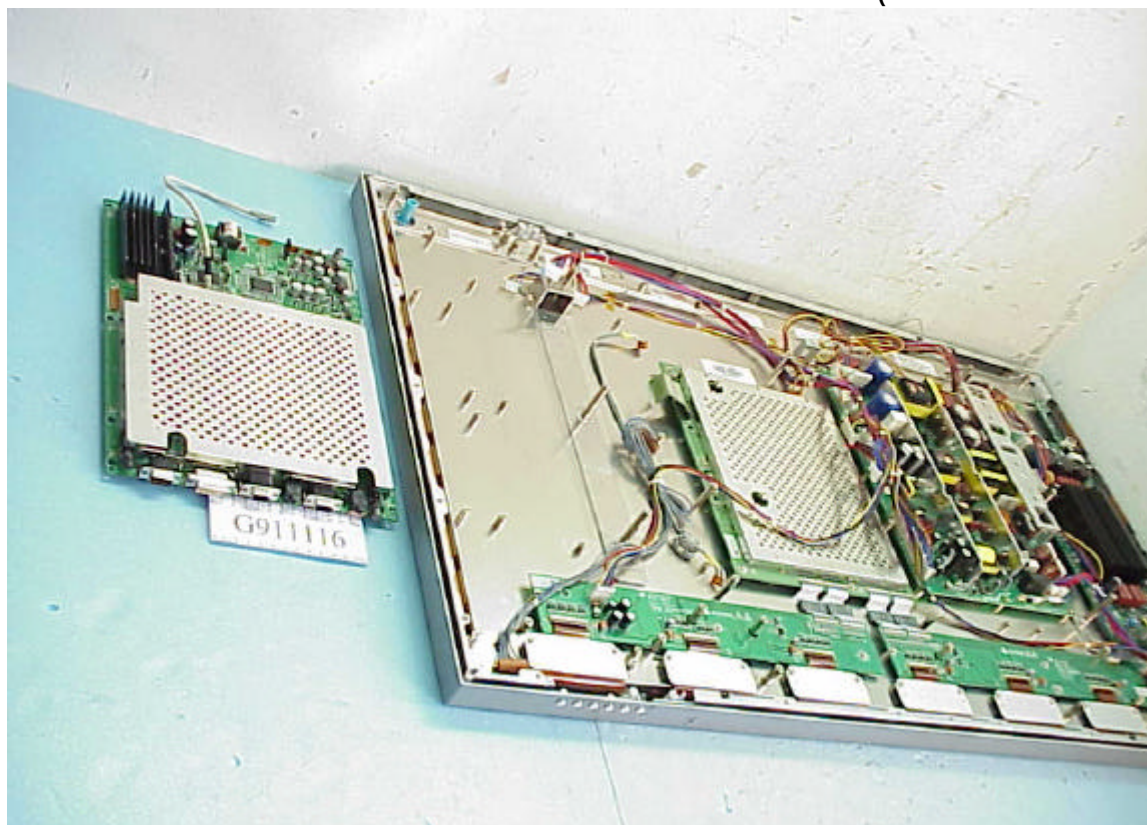
Figure 22 Internal View (Remove Main Board)
