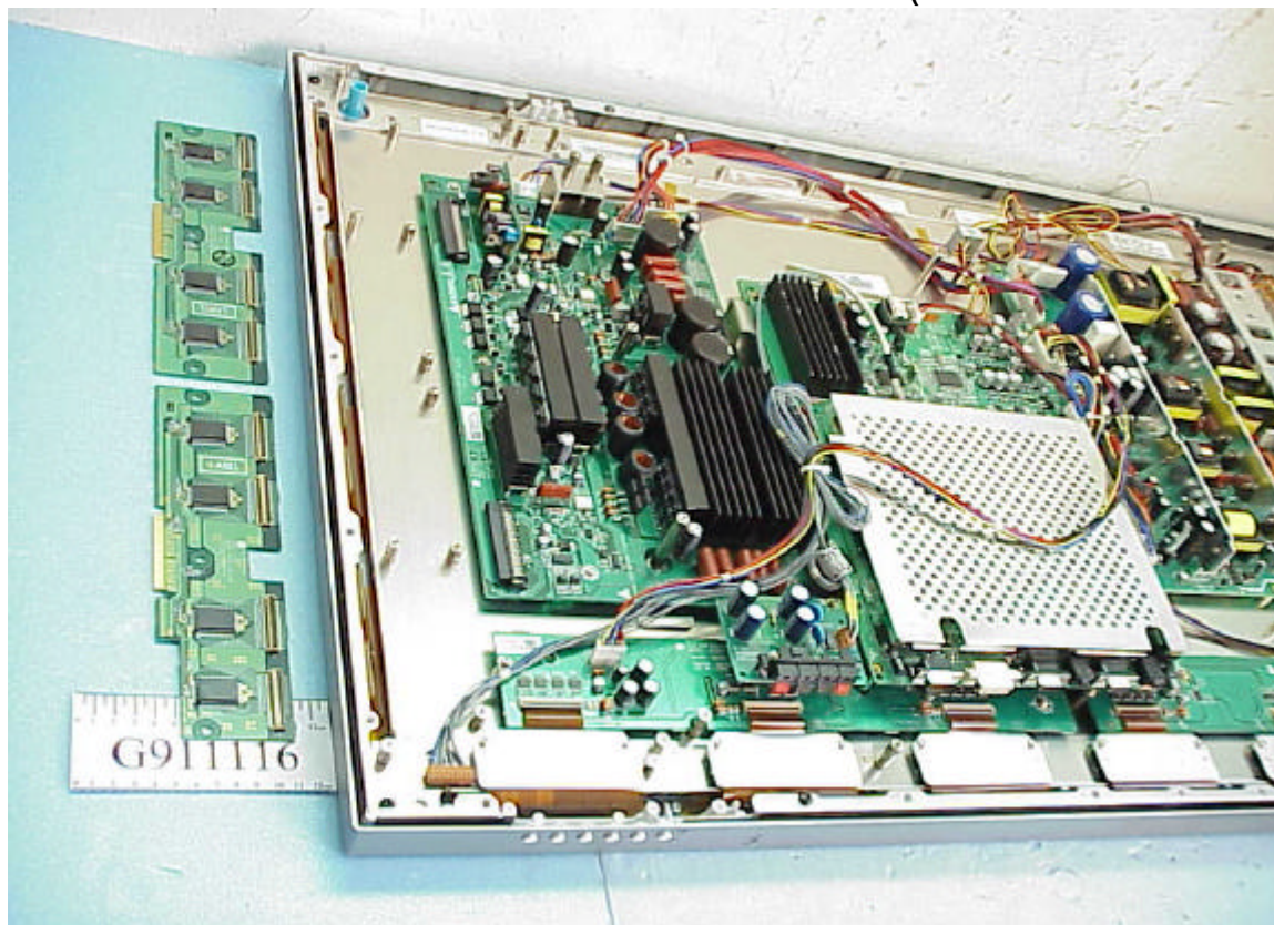
Figure 17 Internal View (Remove Y Drive Boards)
