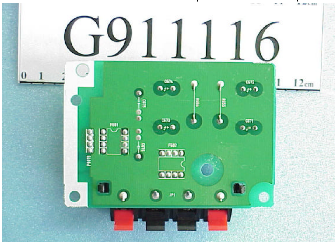
Figure 41 Speaker Control Board (Solder Side)
