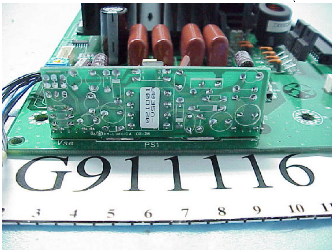
Figure 35 Z-SUS Drive Board (Solder Side)
