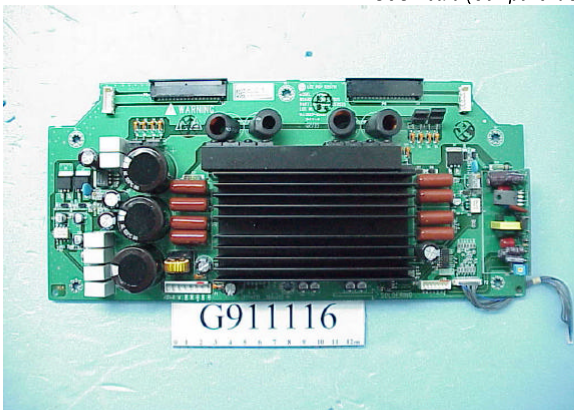
Figure 32 Z-SUS Board (Component Side)
