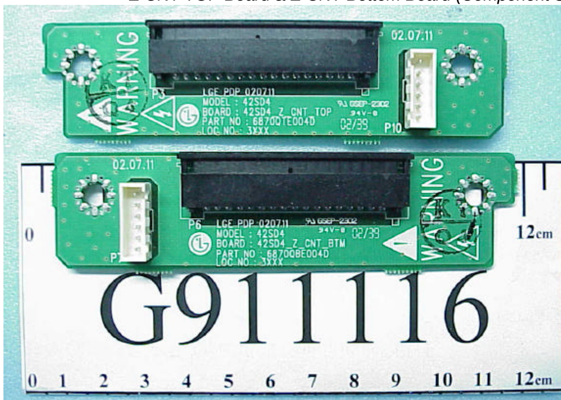
Figure 36 Z-CNT TOP Board & Z-CNT Bottom Board (Component Side)
