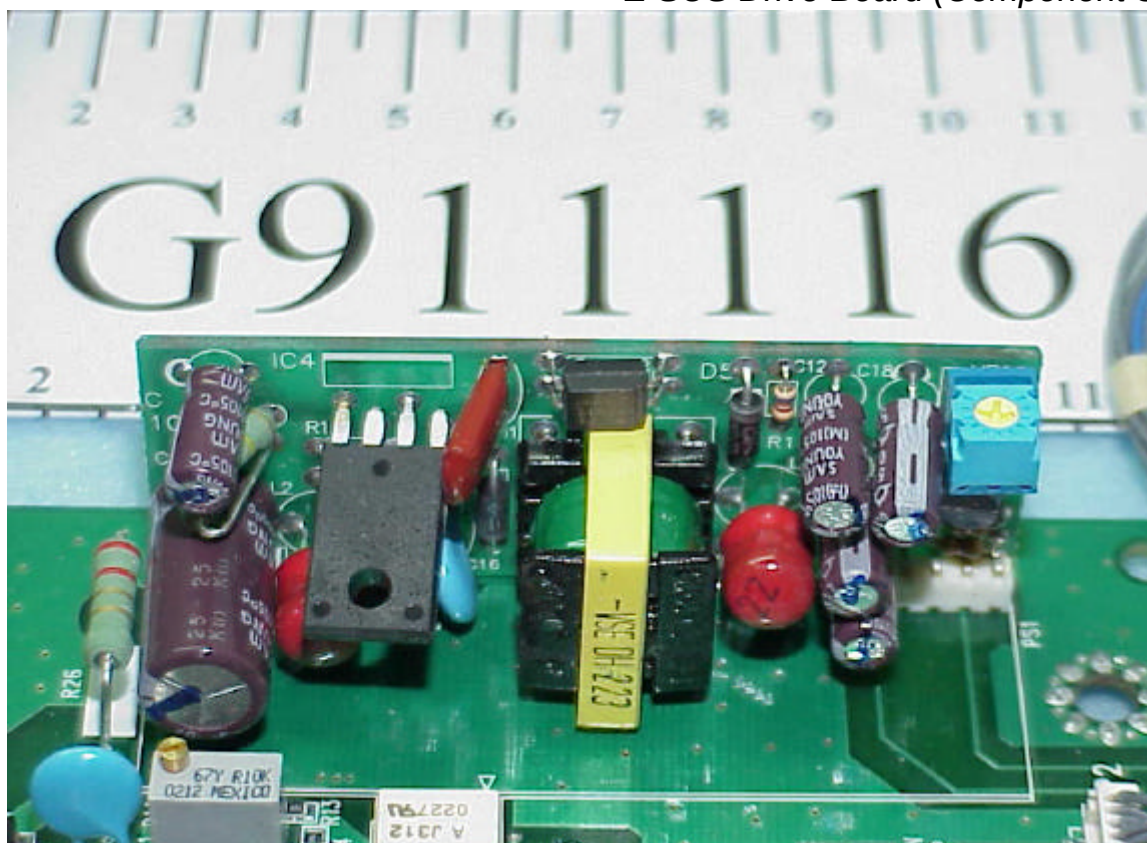
Figure 34 Z-SUS Drive Board (Component Side)
