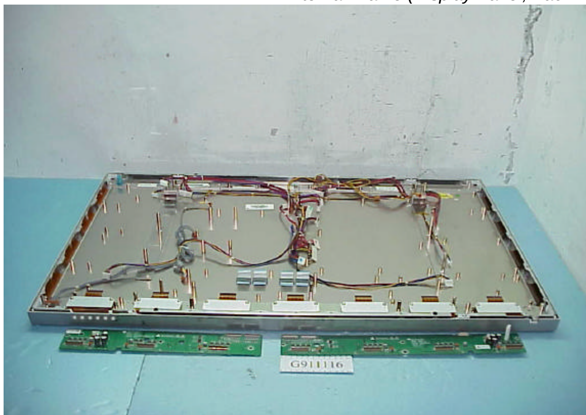
Figure 42 Internal Frame (Display Panel, Back View)
