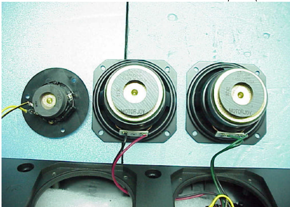
Figure 49 Speaker (Internal View)
