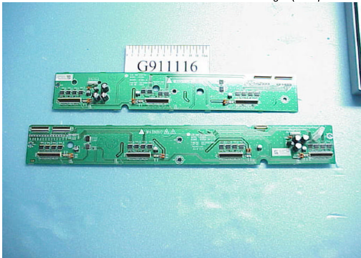
Figure 38 X Drive Board – Left & X Drive Board – Right (Component Side)
