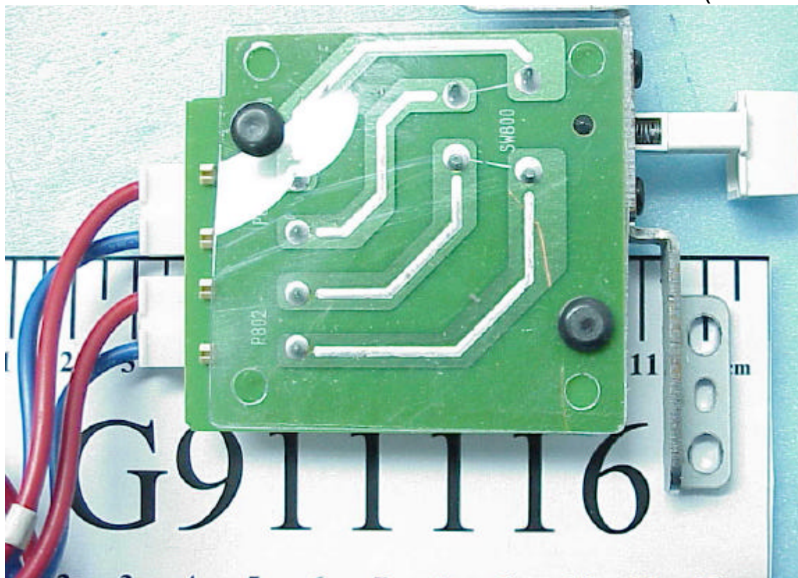
Figure 31 Switch Board (Solder Side)
