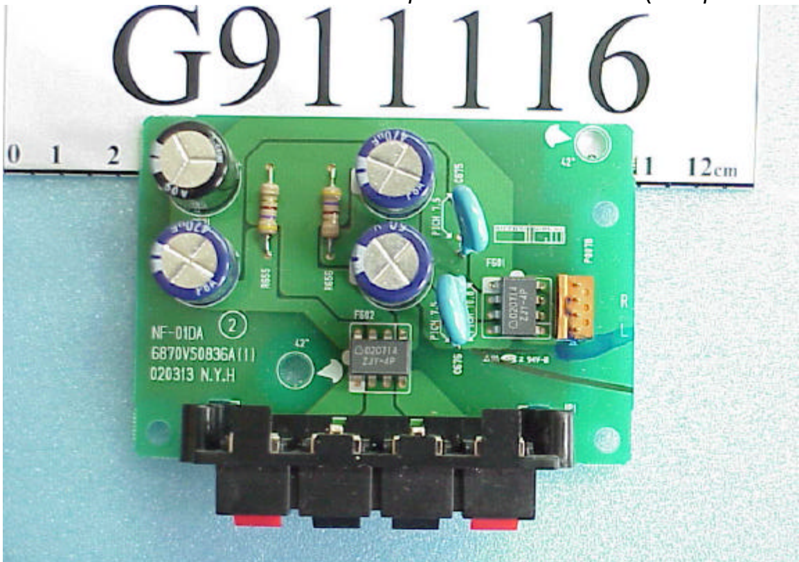
Figure 40 Speaker Control Board (Component Side)
