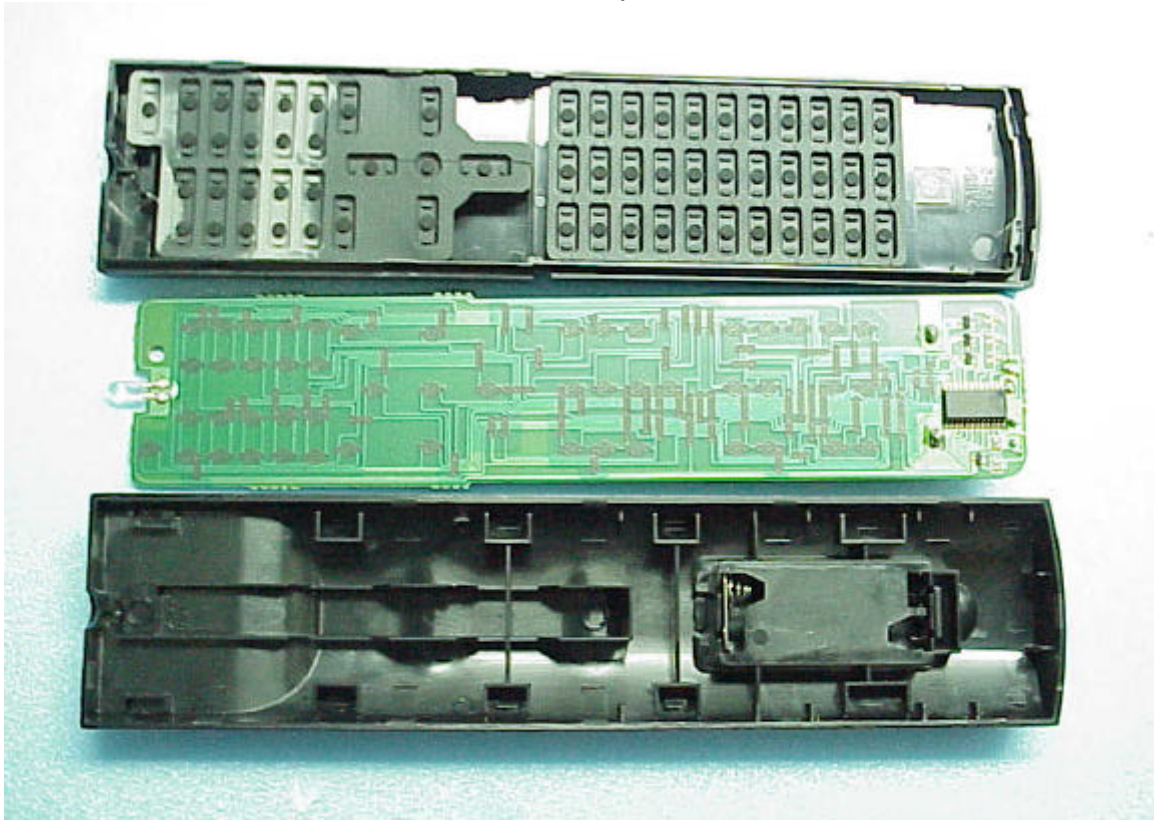
Figure 53 Remote Control (Remove Case Covers, Frame of Internal)
