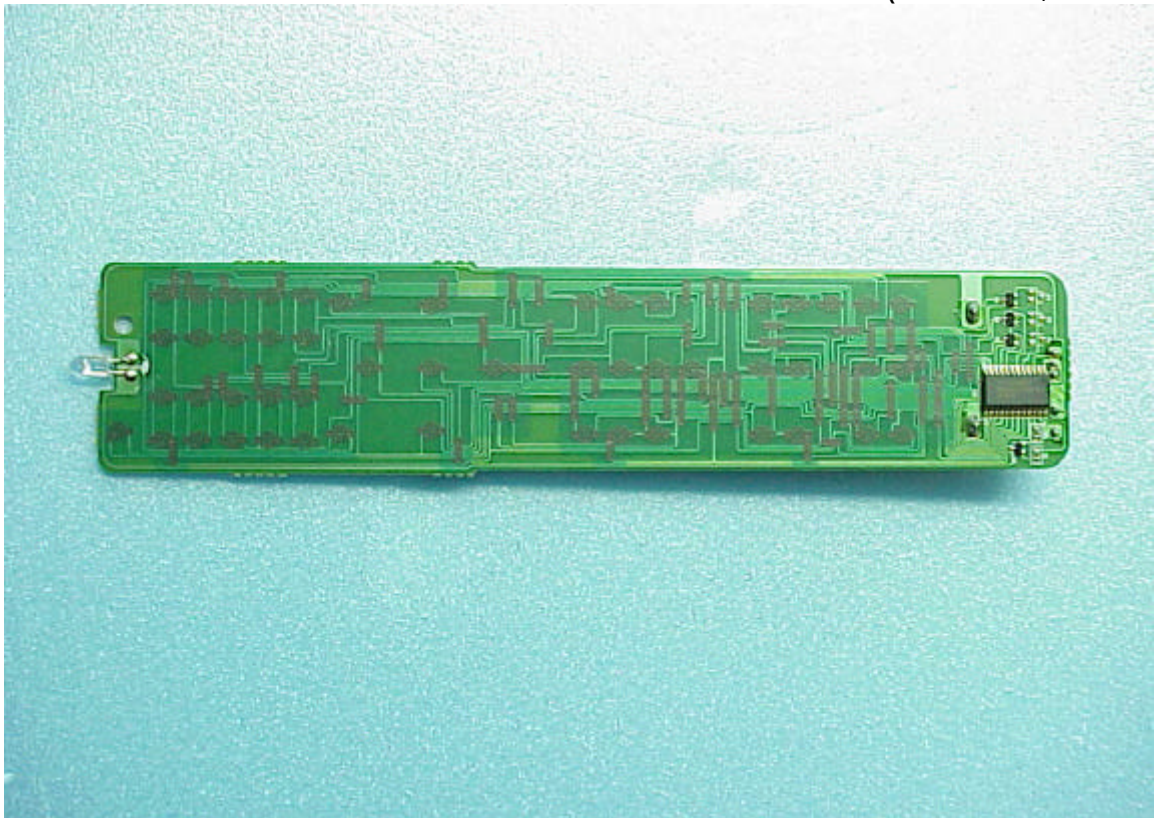
Figure 54 Remote Control (PCB View, Back Side)
