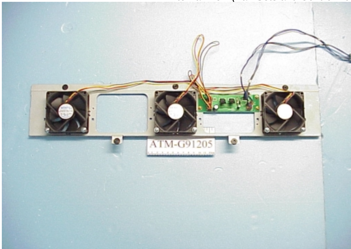
Figure 11 Internal View (Fan Sets and Control Board)
