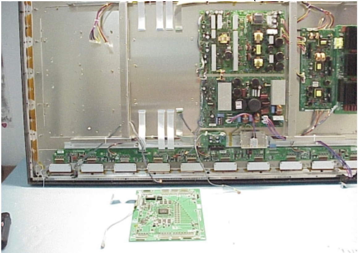
Figure 23 Frame of Internal (Removed Control Board)
