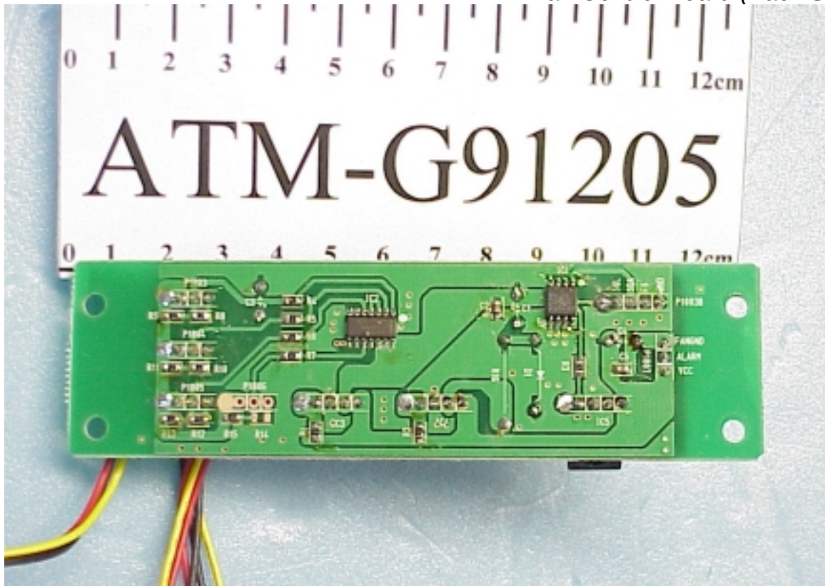
Figure 13 Fan Control Board (Back Side)
