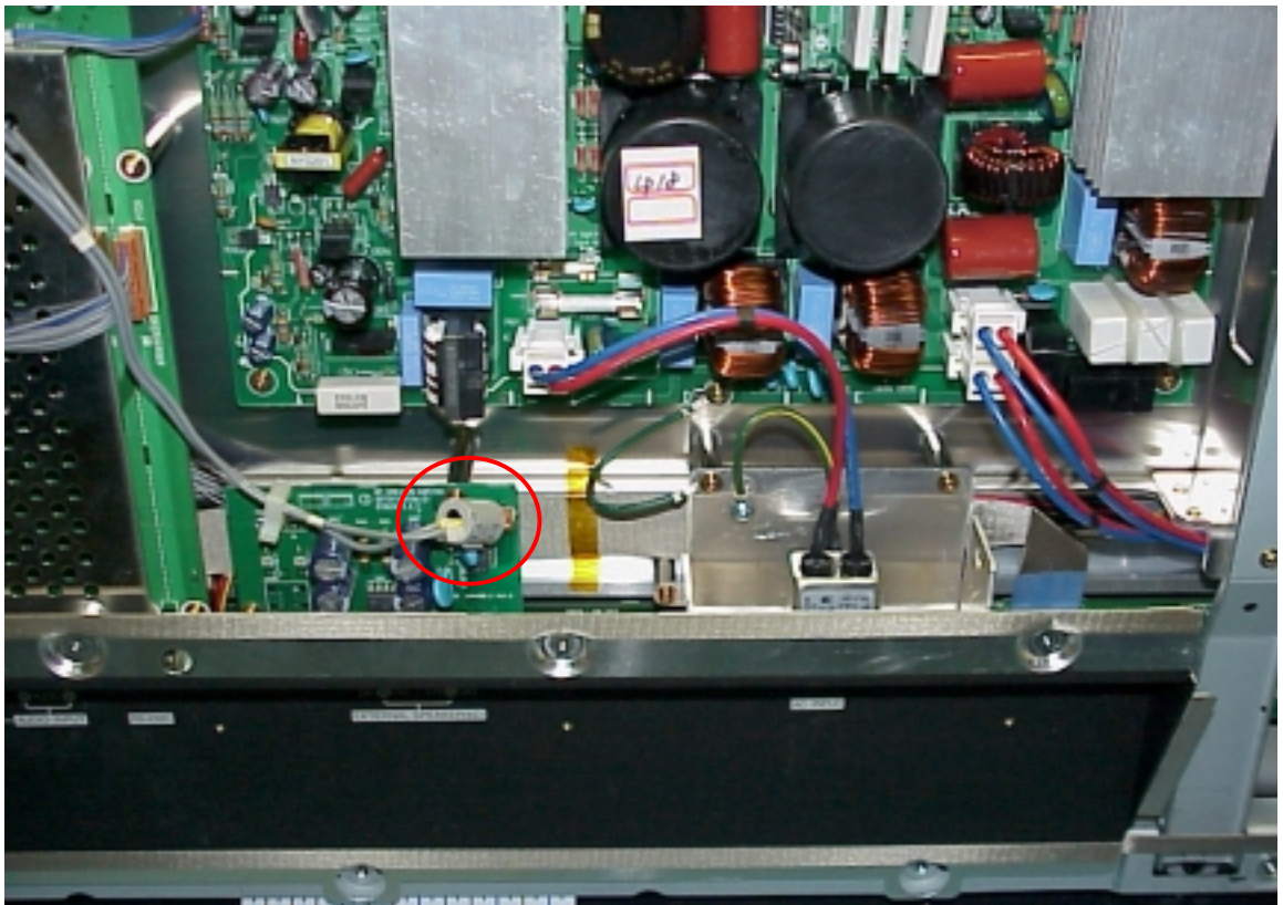
Figure 8 Internal View
