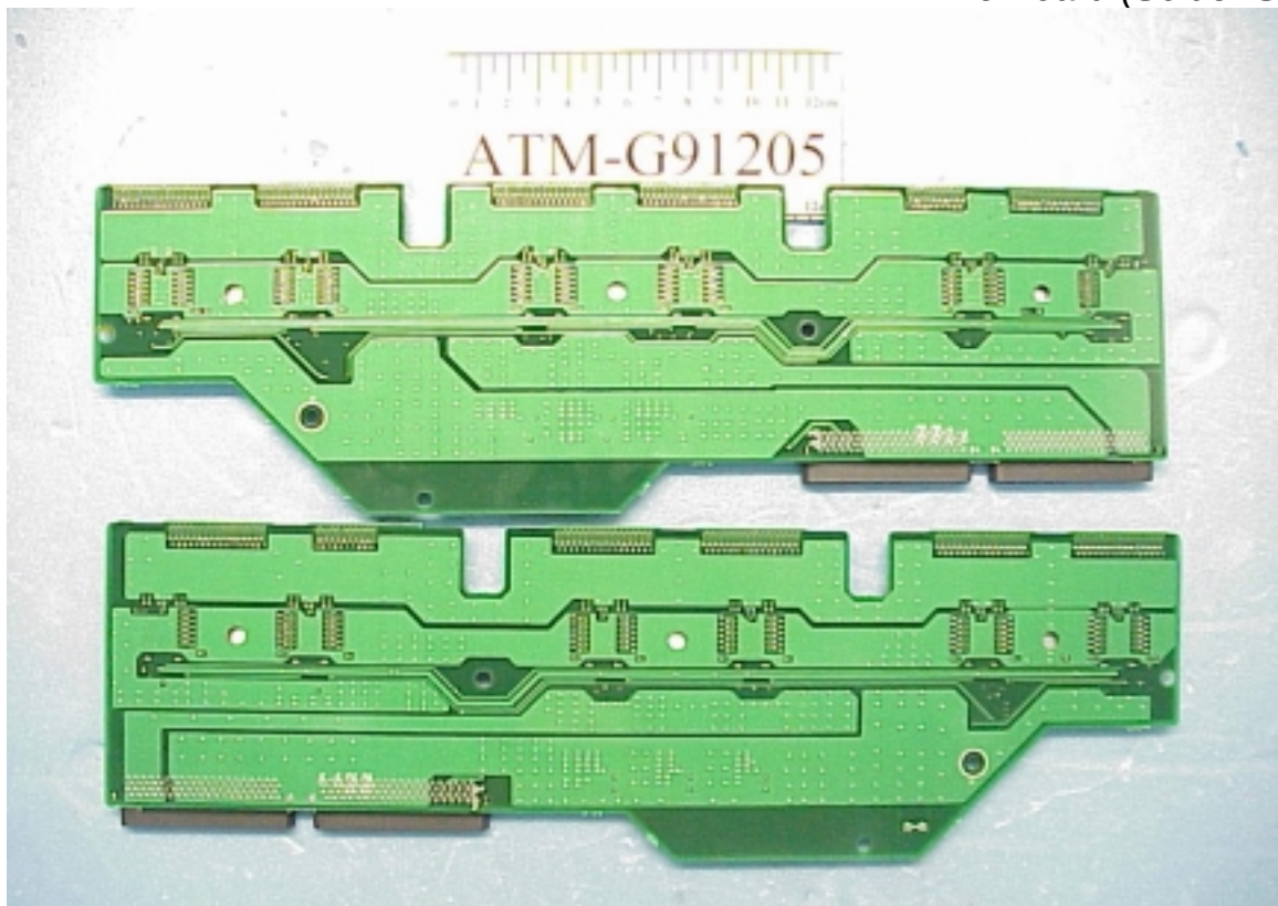
Figure 16 Y-Drive Board (Solder Side)
