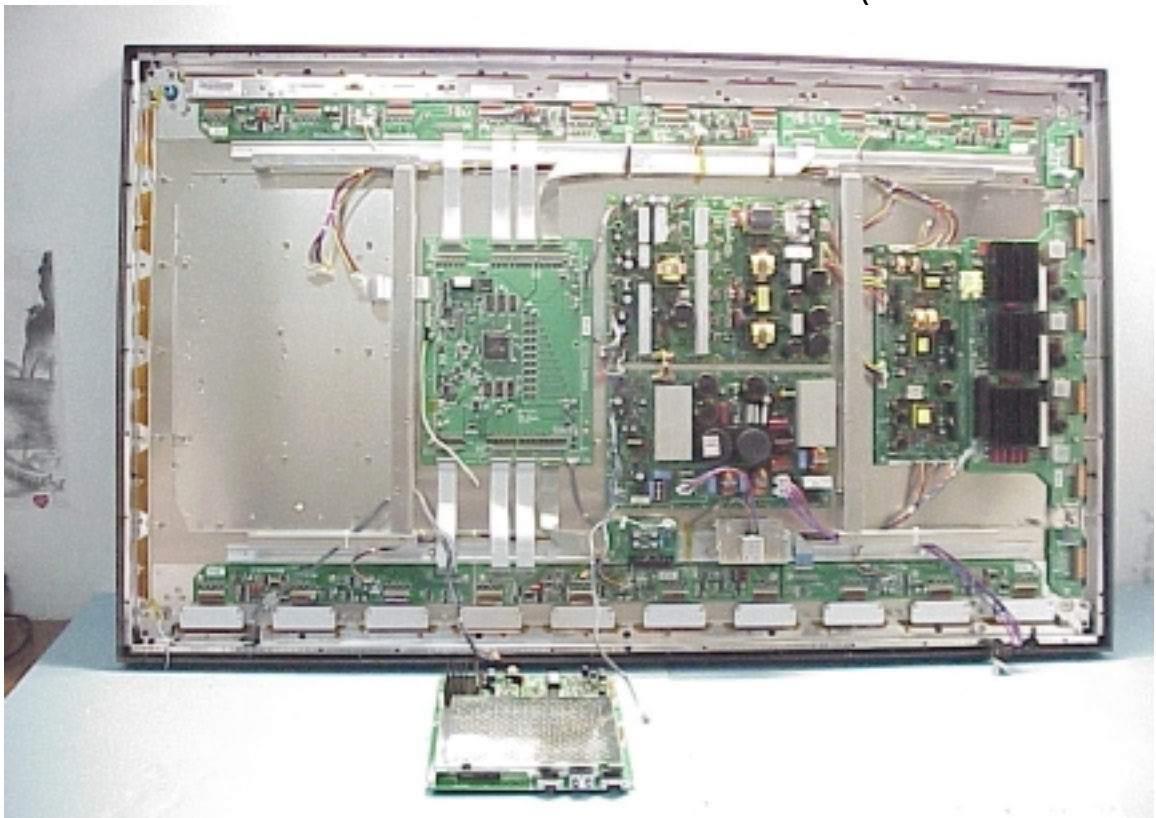
Figure 20 Frame of Internal (Removed VSC Board)
