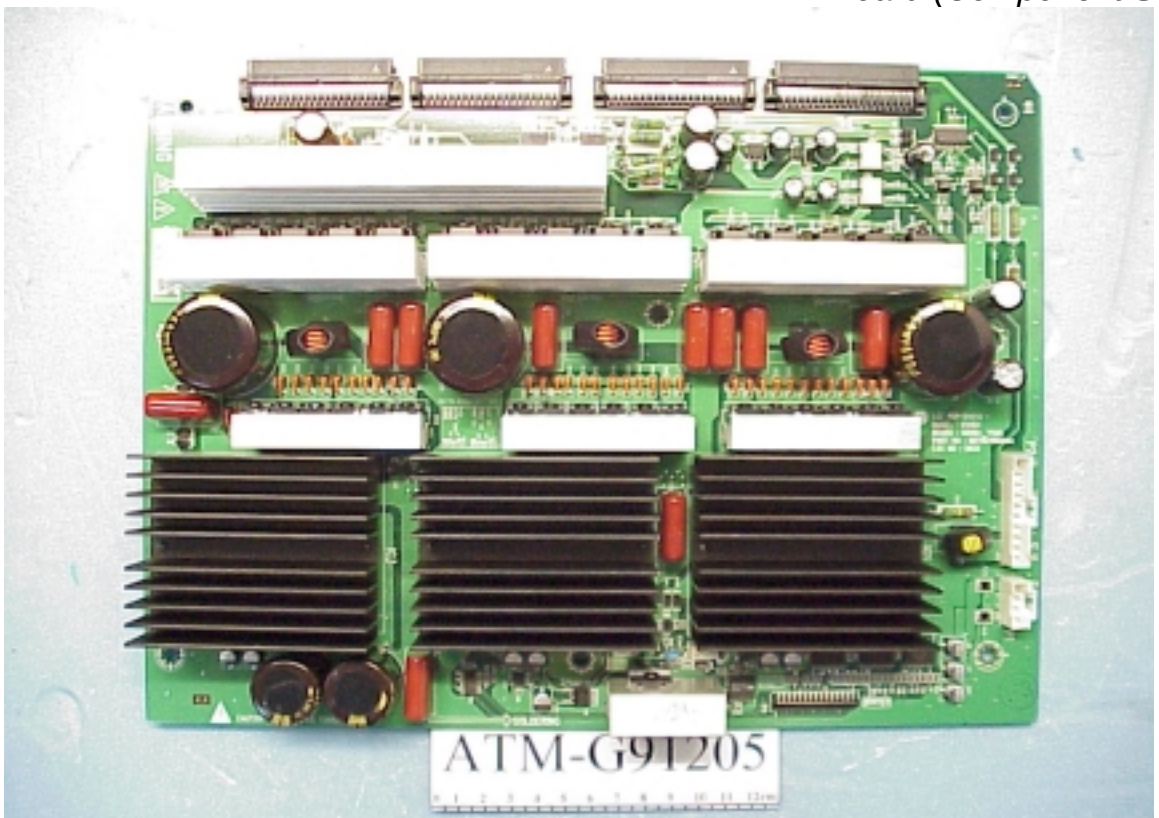
Figure 18 Y Board (Component Side)
