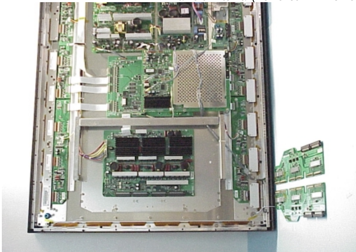
Figure 14 Frame of Internal (Removed Y-Drive Board)
