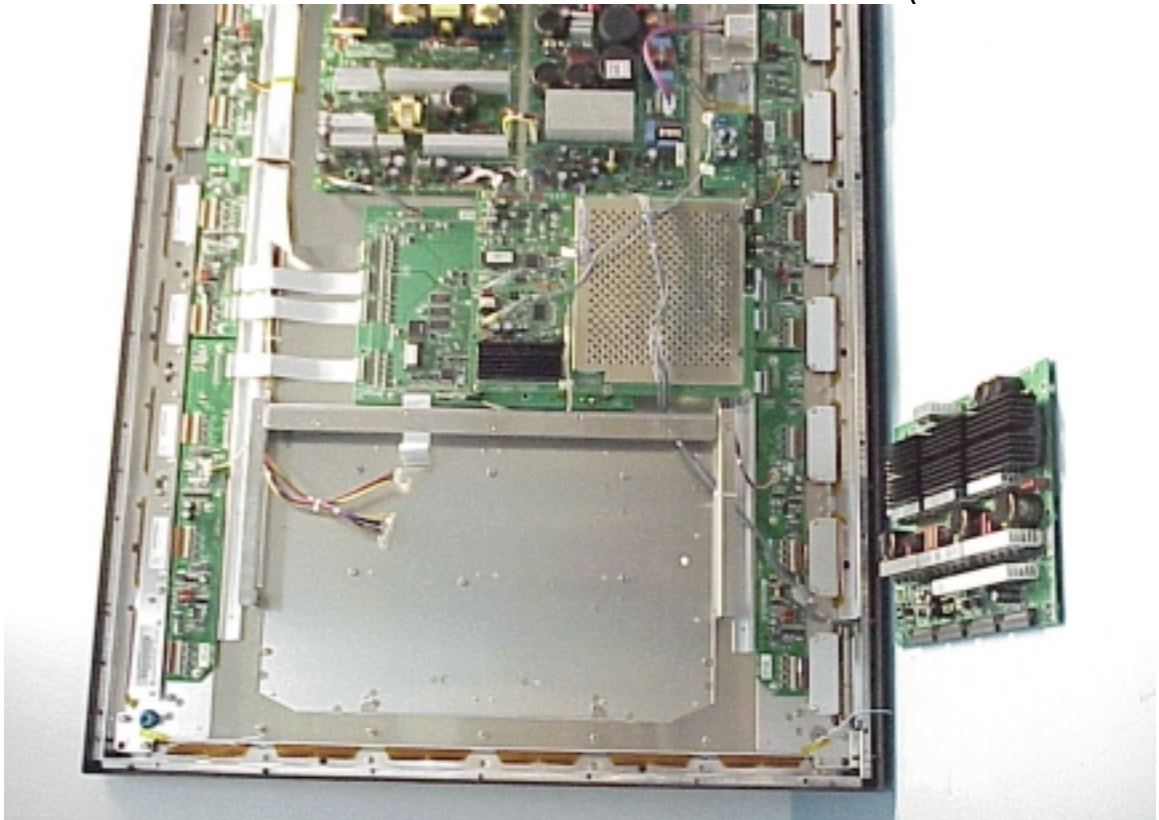
Figure 17 Frame of Internal (Removed Y Board)
