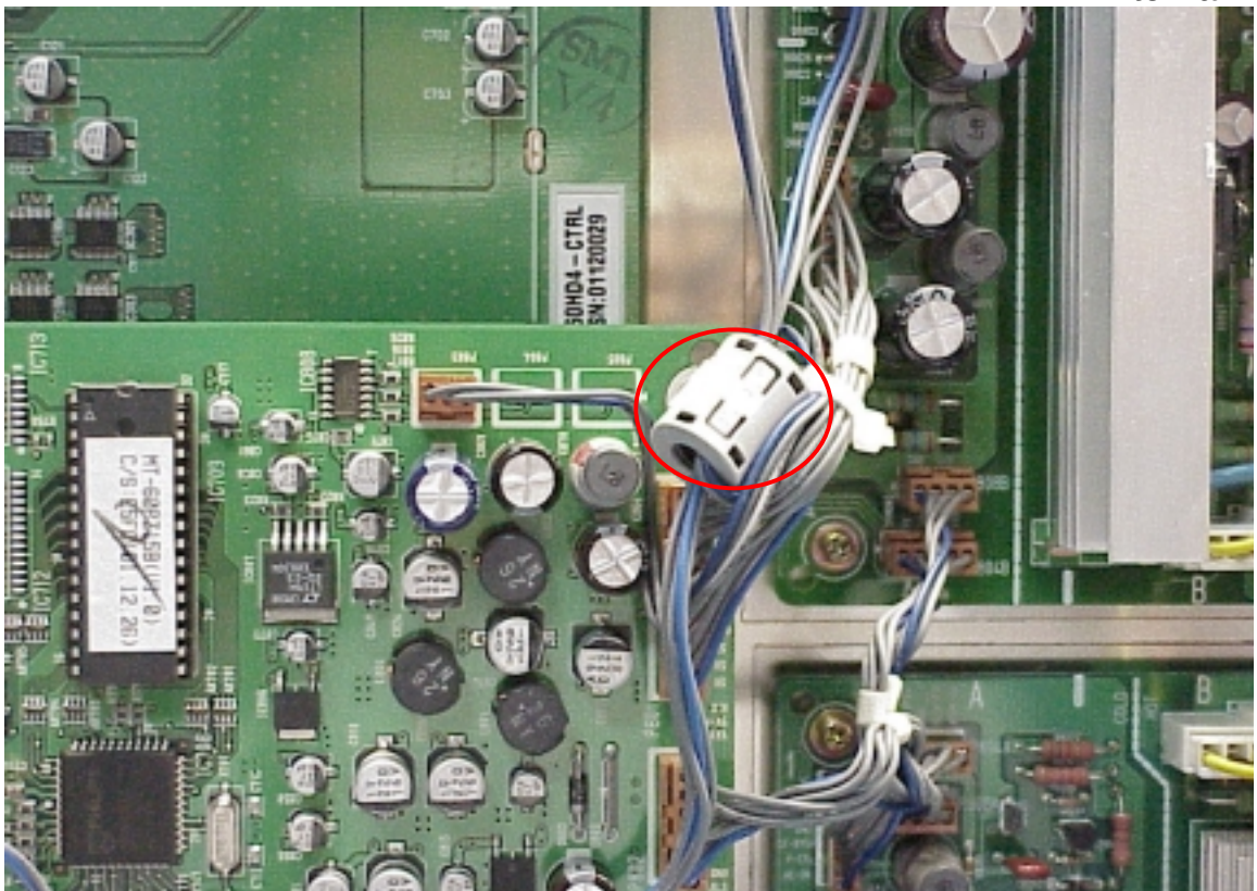
Figure 10 Internal View
