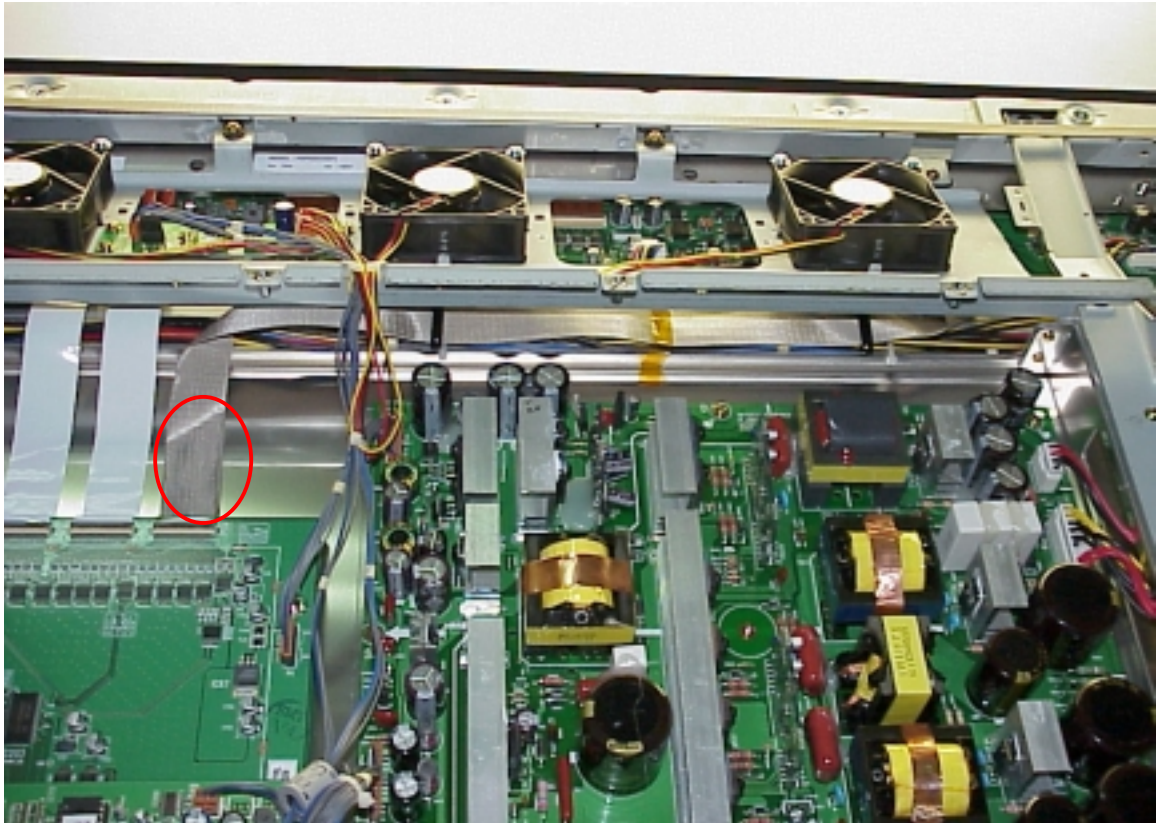
Figure 9 Internal View
