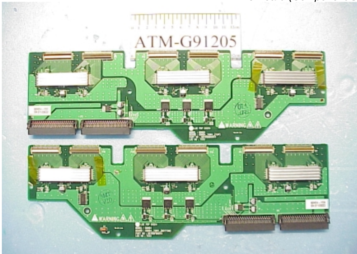
Figure 15 Y-Drive Board (Component Side)
