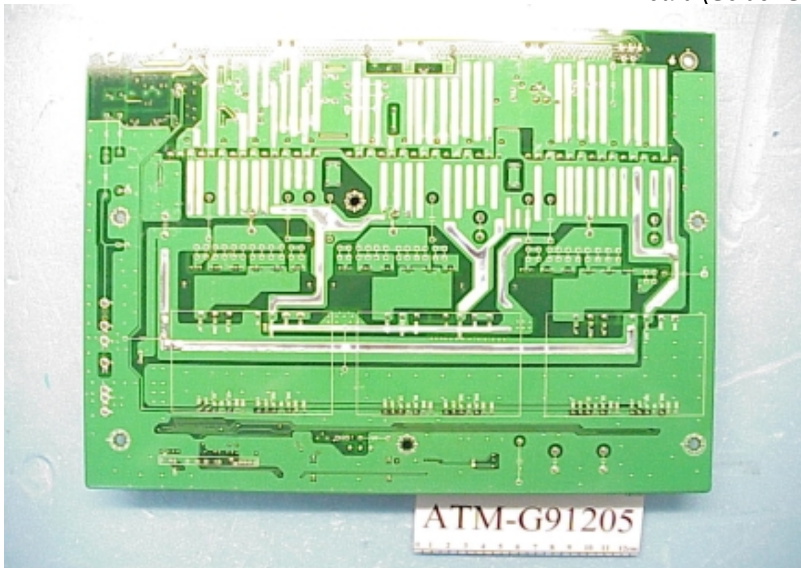
Figure 19 Y Board (Solder Side)
