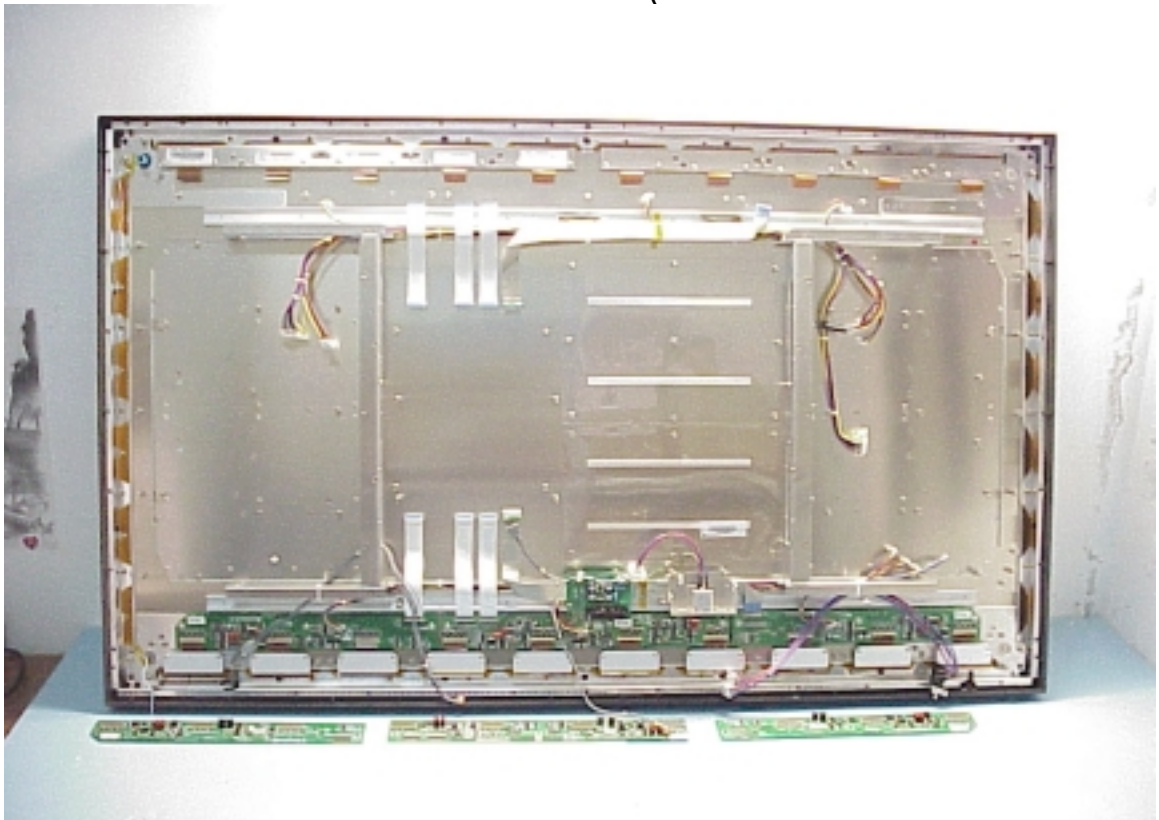
Figure 41 Frame of Internal (Removed X Board & X-Drive Board)
