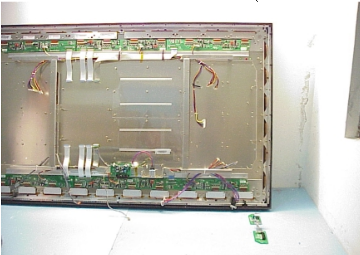
Figure 38 Frame of Internal (Removed Z-Drive Board)
