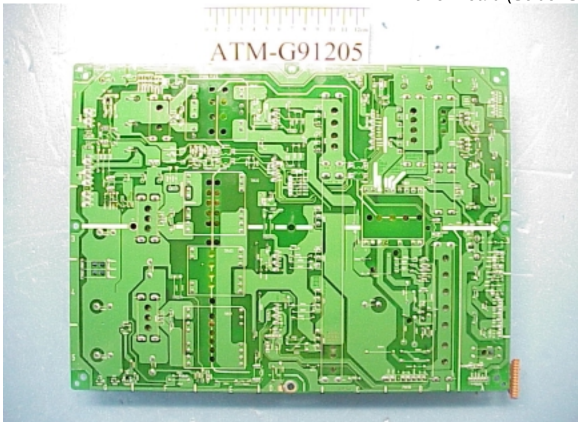
Figure 28 #1 Power Board (Solder Side)
