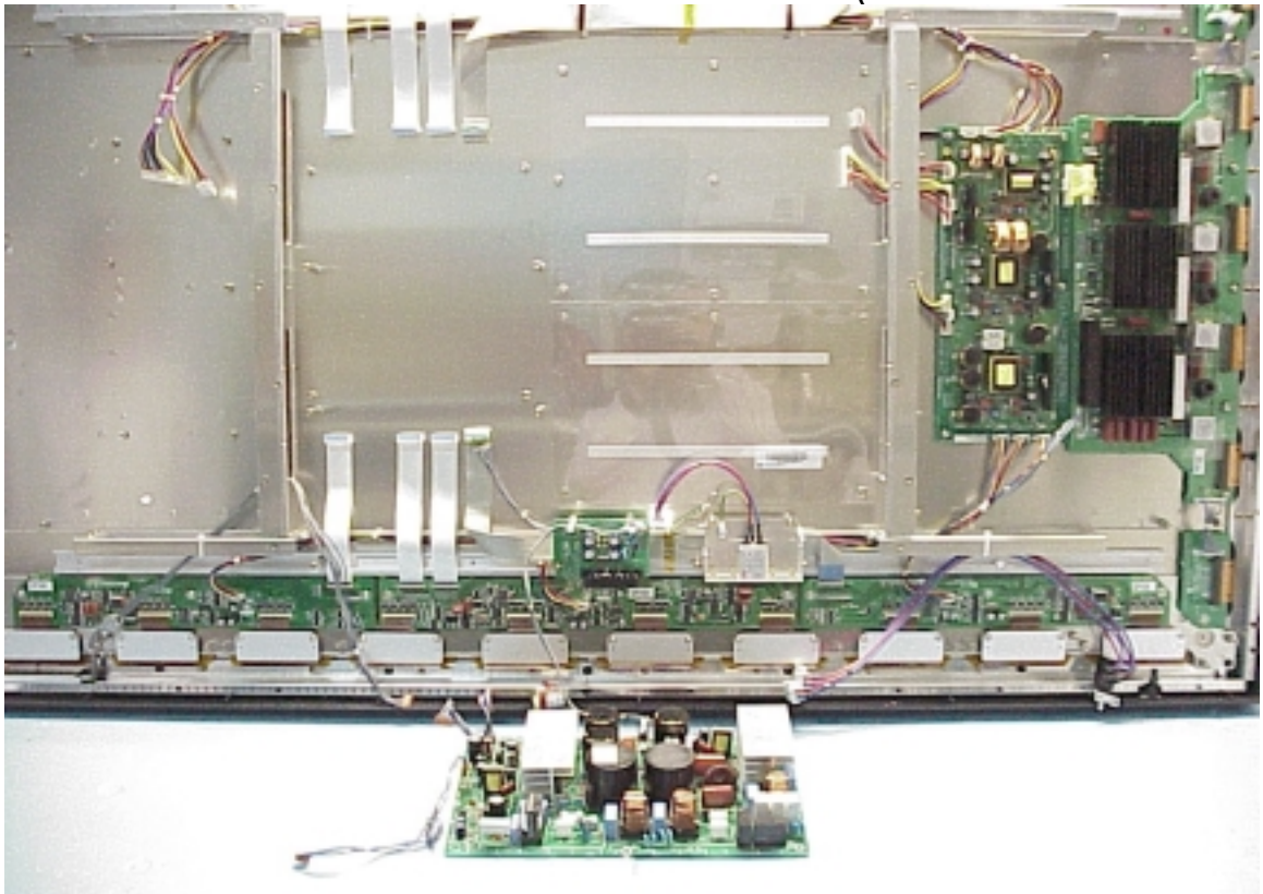
Figure 29 Frame of Internal (Removed #2 Power Board)
