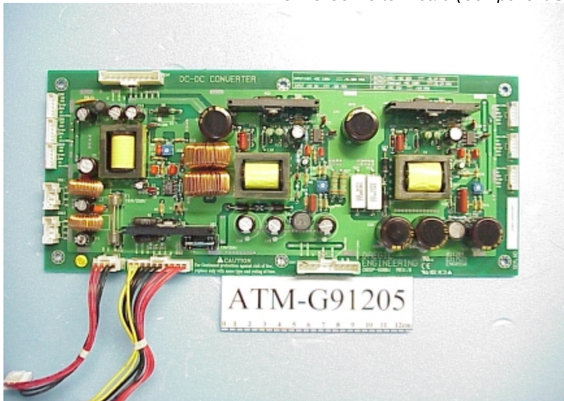
Figure 33 DC-DC Converter Board (Component Side)
