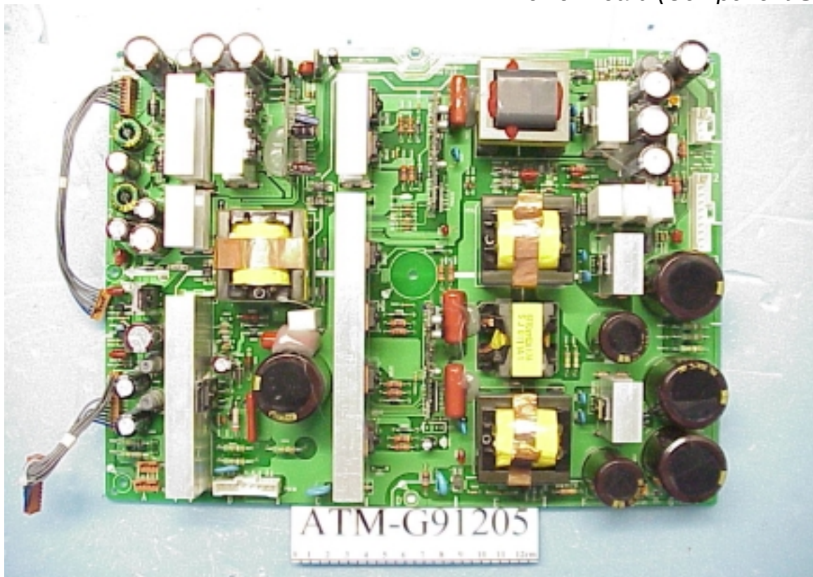
Figure 27 #1 Power Board (Component Side)
