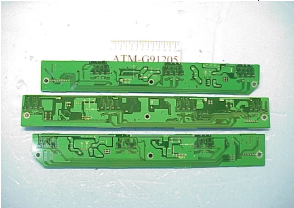
Figure 43 X Board & X-Drive Board (Solder Side)
