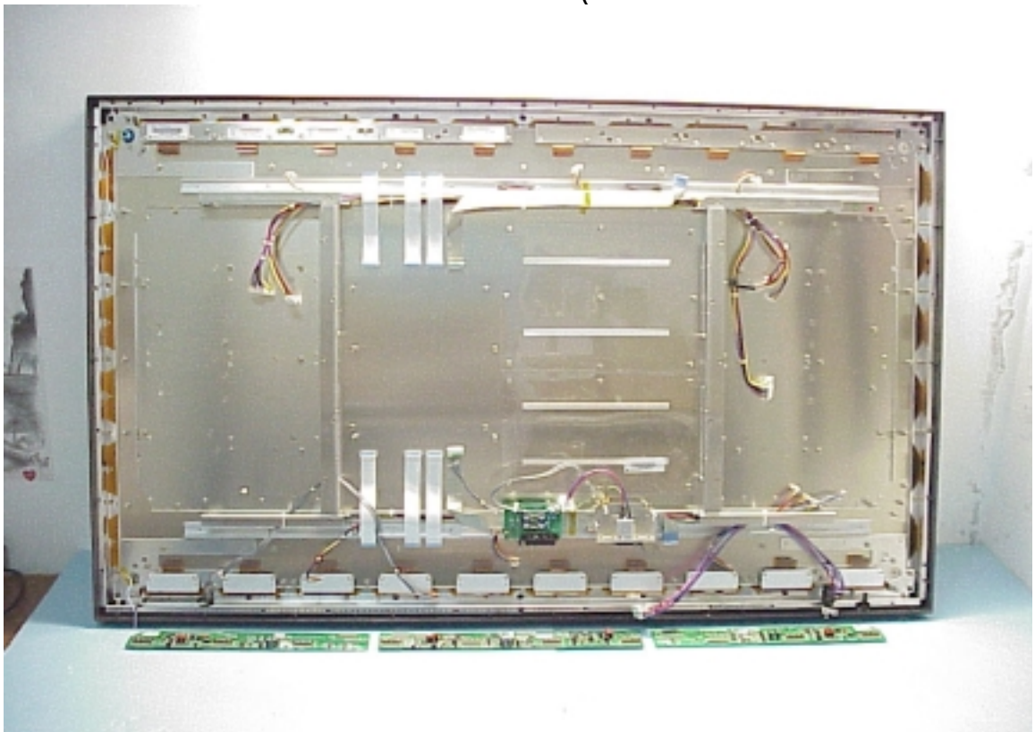
Figure 44 Frame of Internal (Removed X Board & X-Drive Board)
