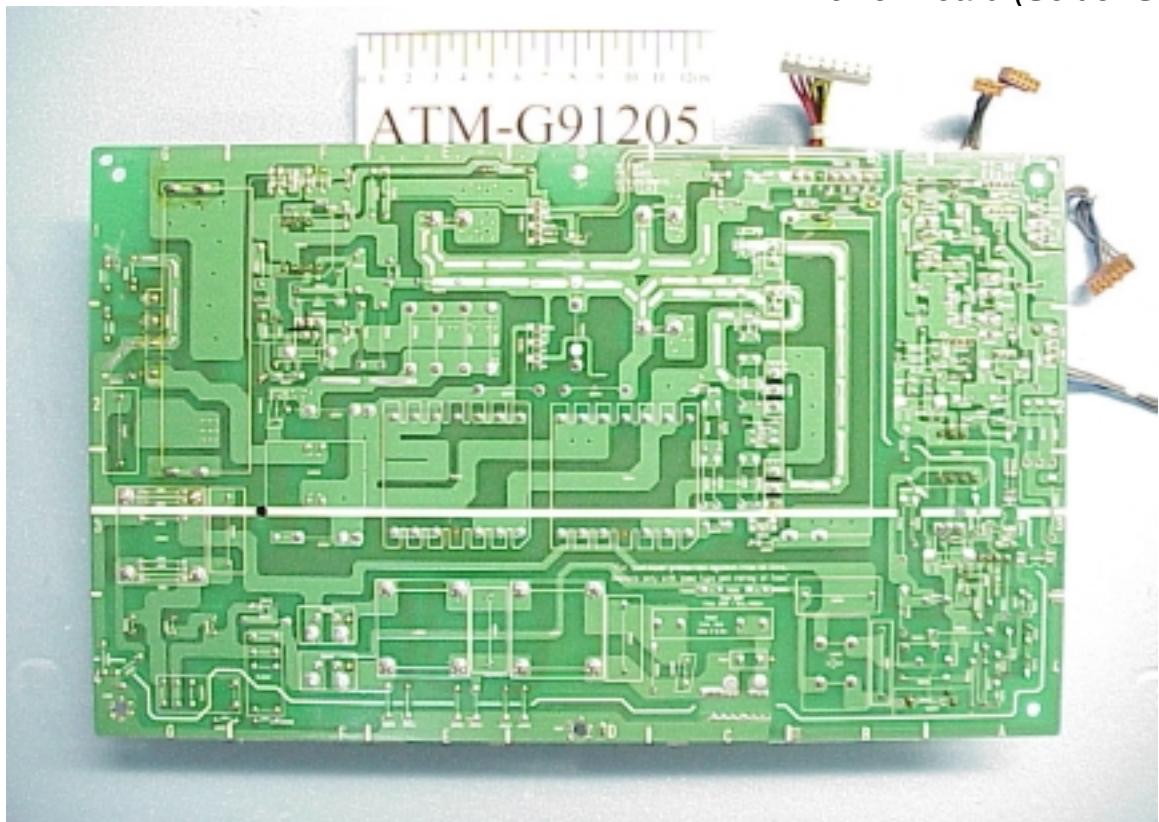
Figure 31 #2 Power Board (Solder Side)
