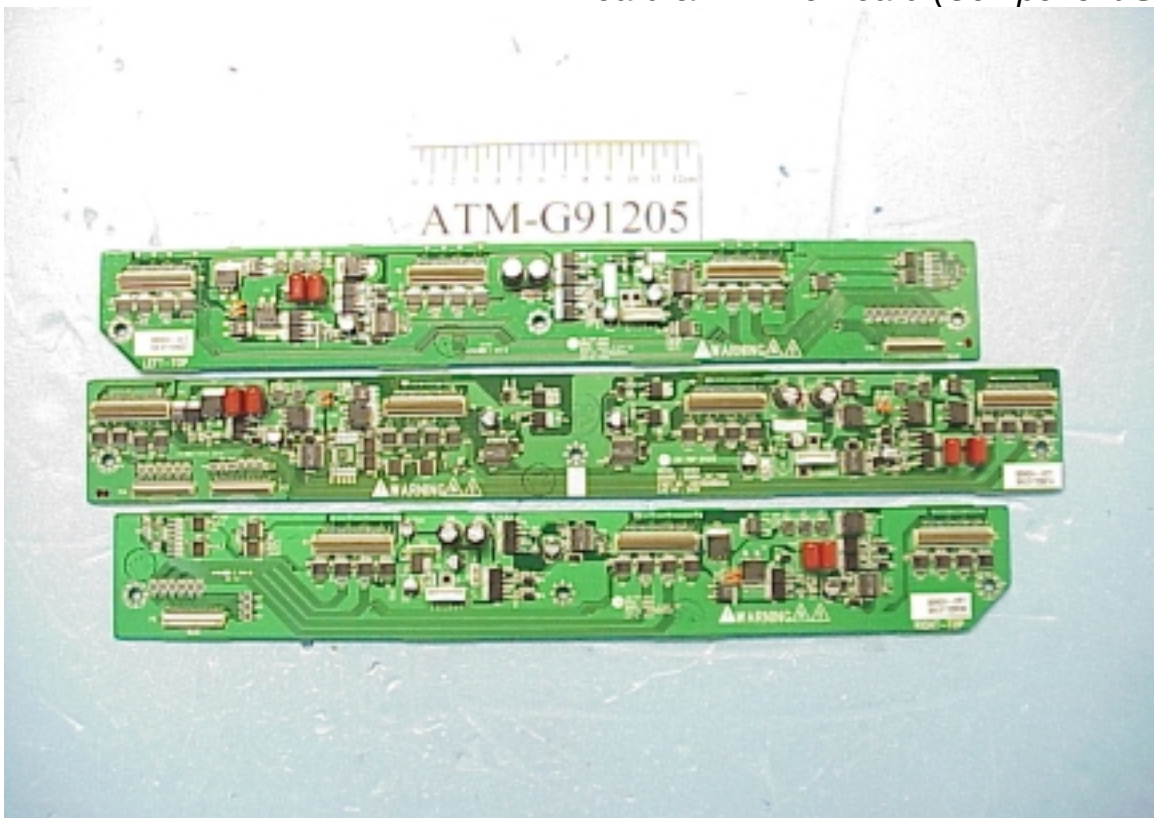
Figure 42 X Board & X-Drive Board (Component Side)
