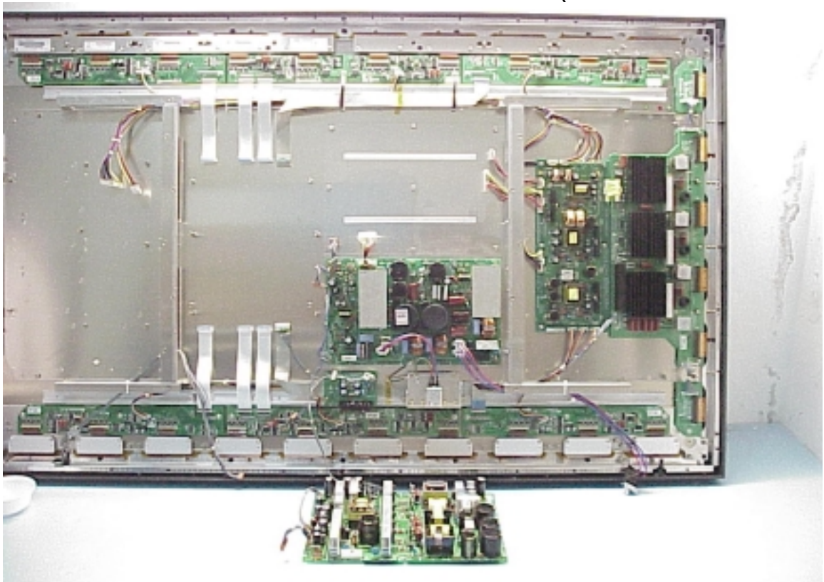
Figure 26 Frame of Internal (Removed #1 Power Board)
