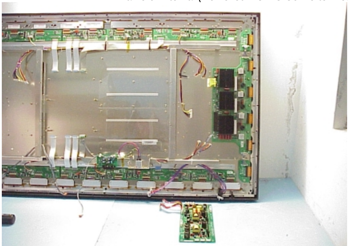
Figure 32 Frame of Internal (Removed DC-DC Converter Board)
