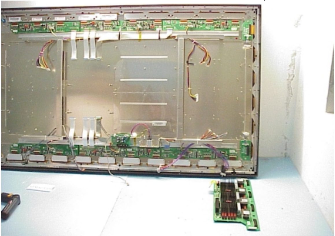
Figure 35 Frame of Internal (Removed Z Board)
