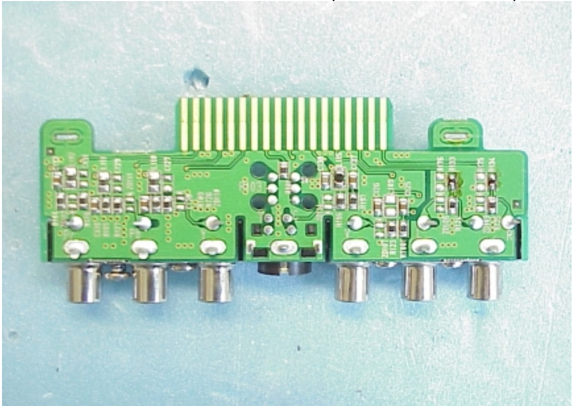
Figure 53 Bracker of A/V & Component Interface Board (Back Side)
