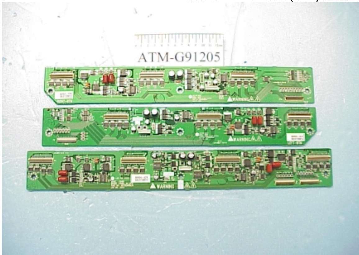
Figure 45 X Board & X-Drive Board (Component Side)
