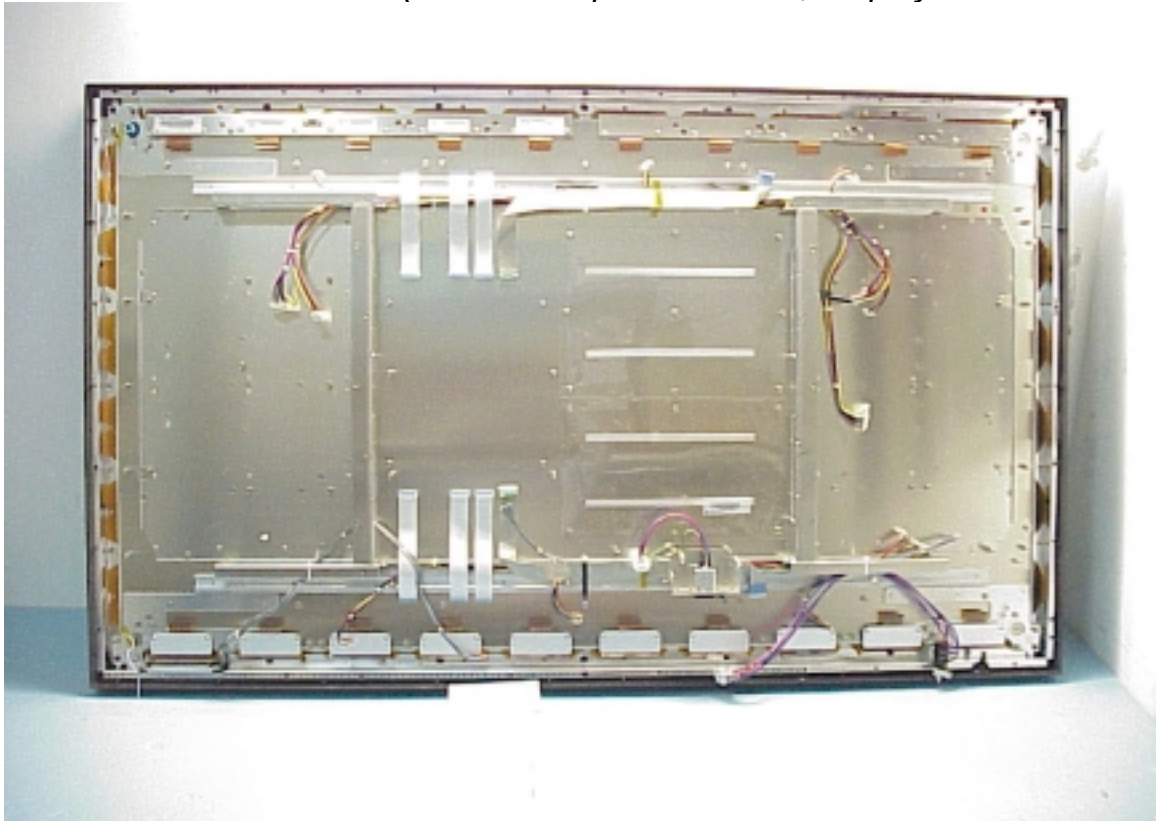
Figure 47 Frame of Internal (Removed Speaker Board, Display Panel/Back View)
