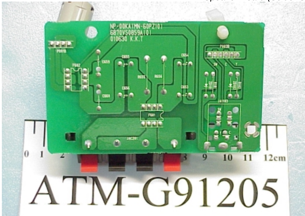
Figure 49 Speaker Board (Solder Side)
