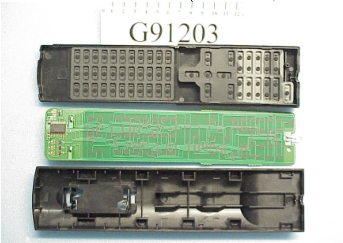
Figure 62 Remote Control (Removed Covers, Frame of Internal)
