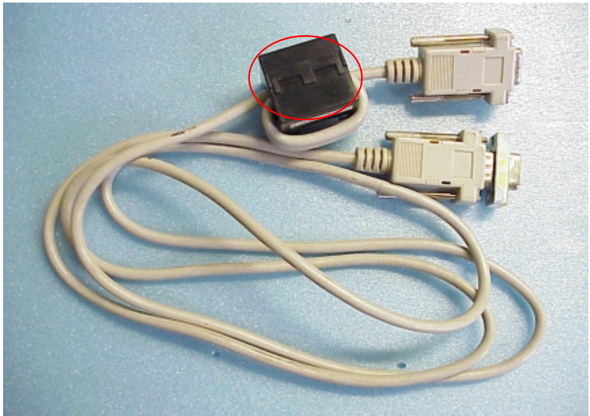
Figure 66 RS232C Cable
