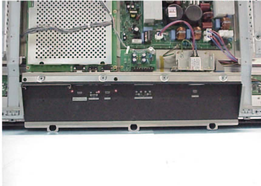
Figure 8 60" Plasma Monitor Internal View
