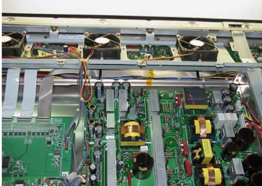
Figure 10 60" Plasma Monitor Internal View
