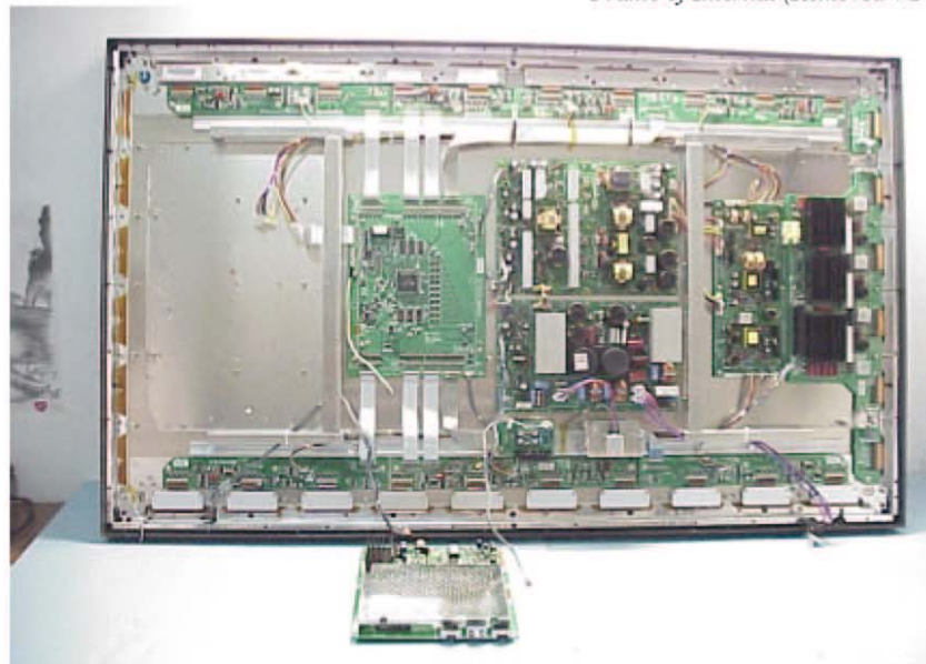
Figure 20 60" Plasma Monitor Frame of Internal (Removed VSC Board)
