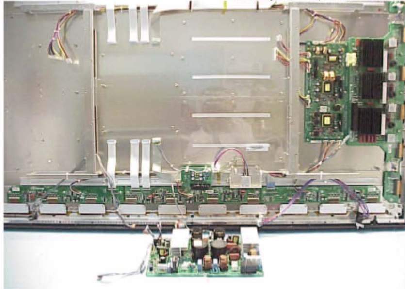
Figure 30 60" Plasma Monitor #2 Power Board (Component Side)
