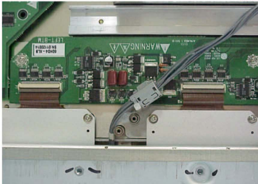
Figure 6 60" Plasma Monitor Internal View
