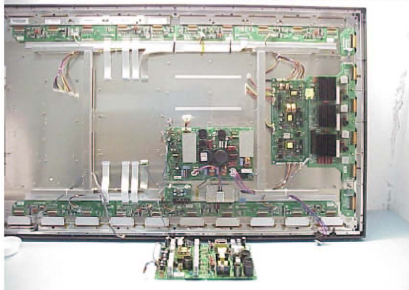
Figure 26 60" Plasma Monitor Frame of Internal (Removed #1 Power Board)
