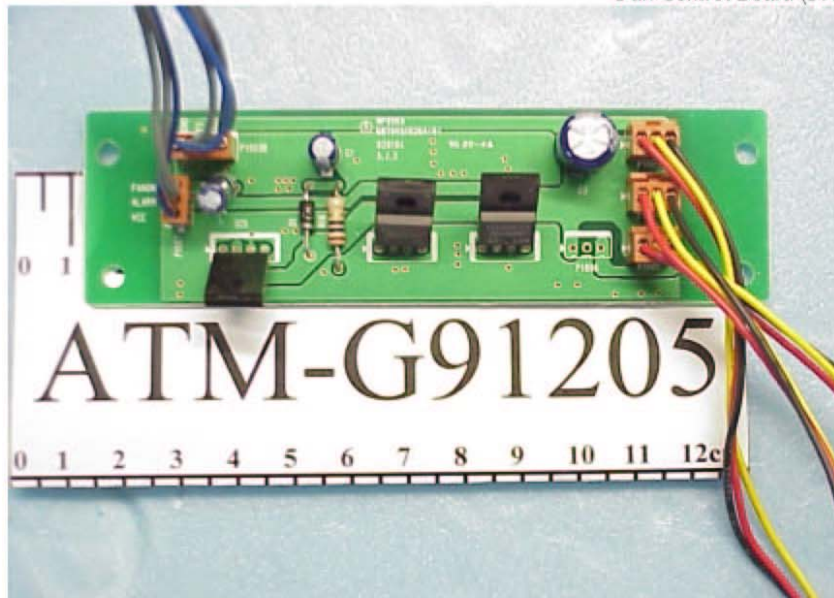
Figure 12 60" Plasma Monitor Fan Control Board (Front Side)
