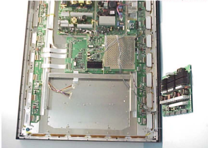
Figure 18 60" Plasma Monitor Y Board (Component Side)
