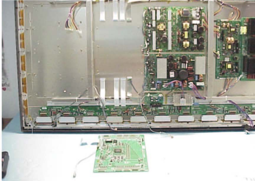
Figure 24 60" Plasma Monitor Control Board (Component Side)
