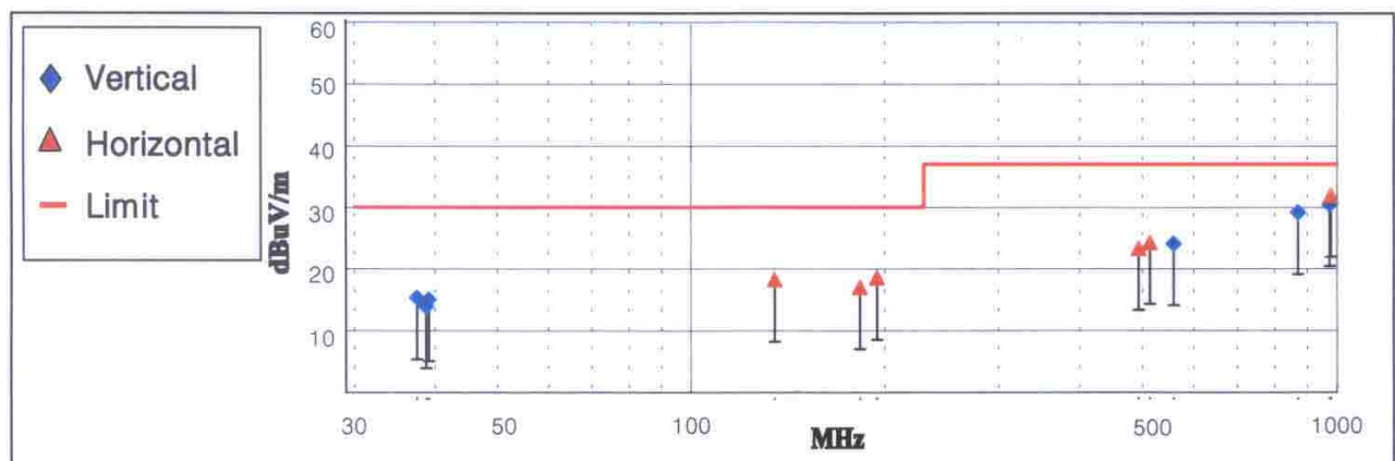
< Fig 6-1. Radiated emission result >
