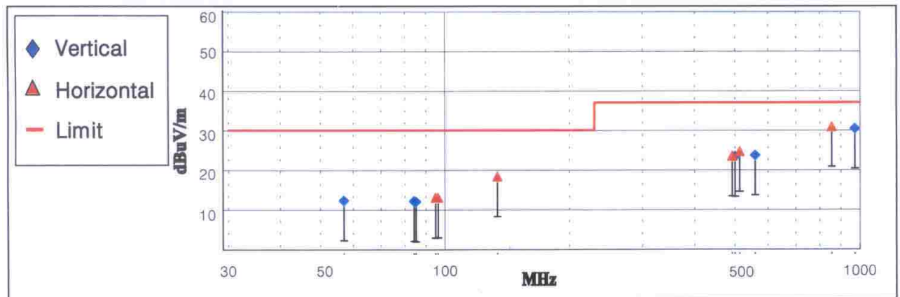
< Fig 6-2. Radiated emission result >
