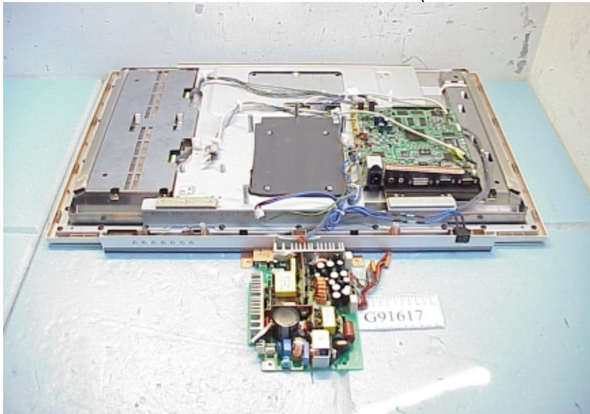
Figure 15 Internal View (Remove the Power Board)
