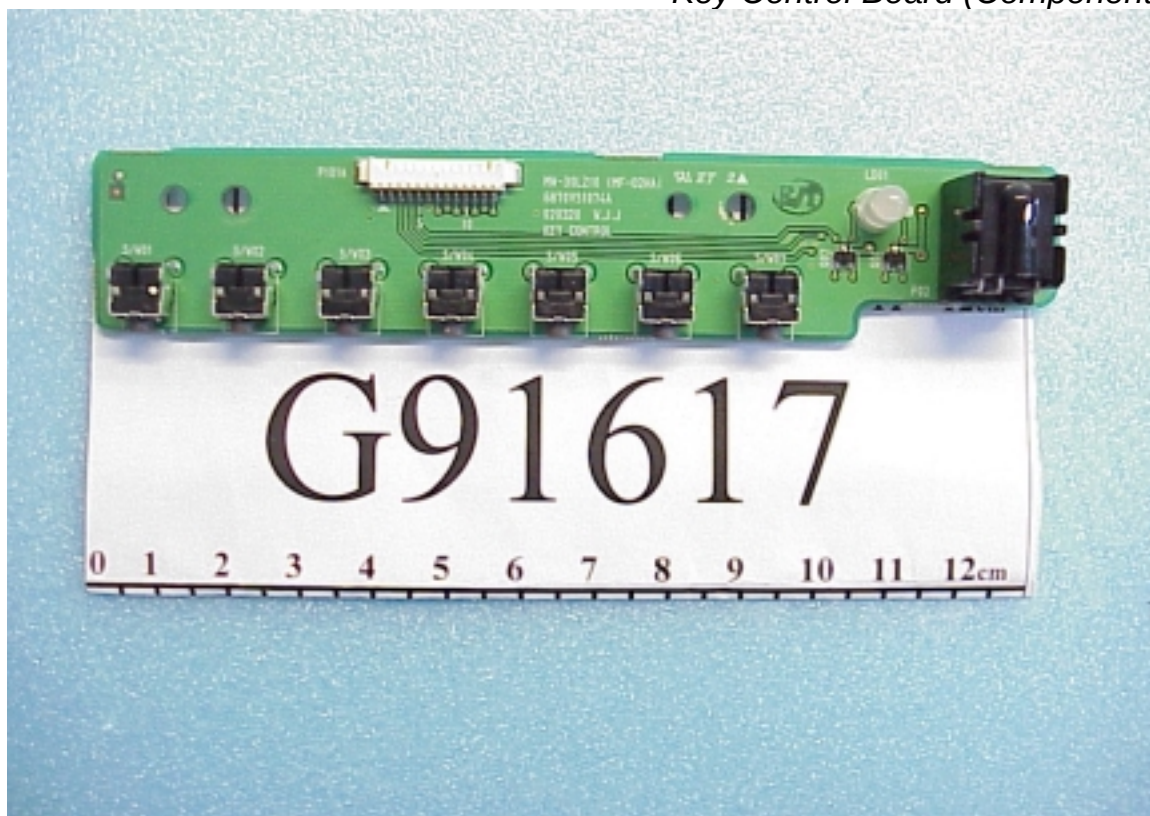
Figure 13 Key Control Board (Component Side)
