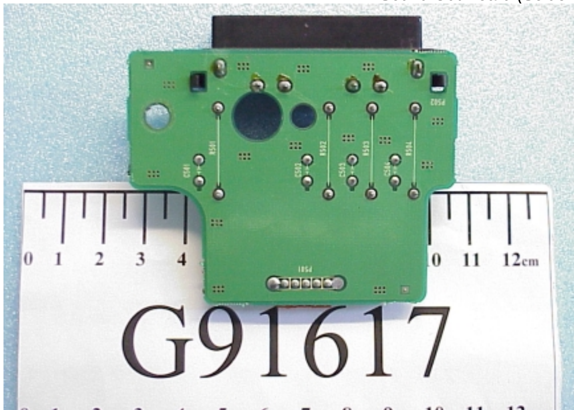
Figure 12 Sound Out Board (Solder Side)
