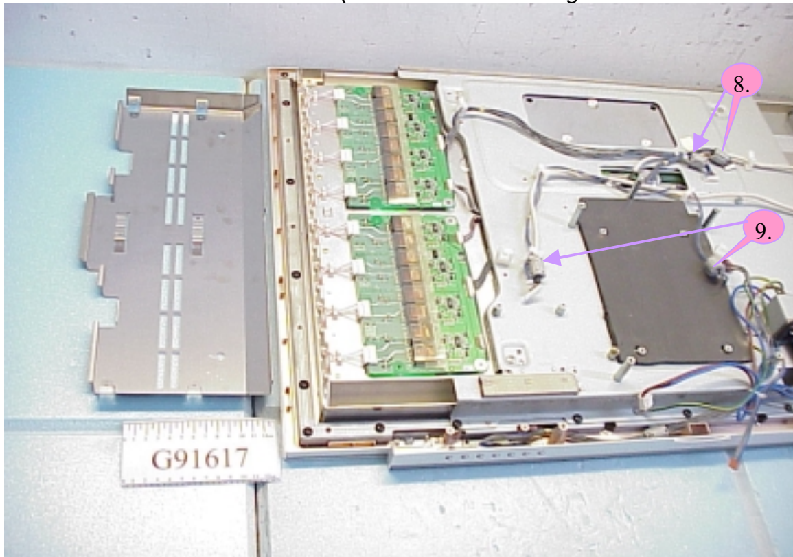
Figure 21 Internal View (Remove the Shielding Cover of Inverter Boards)
