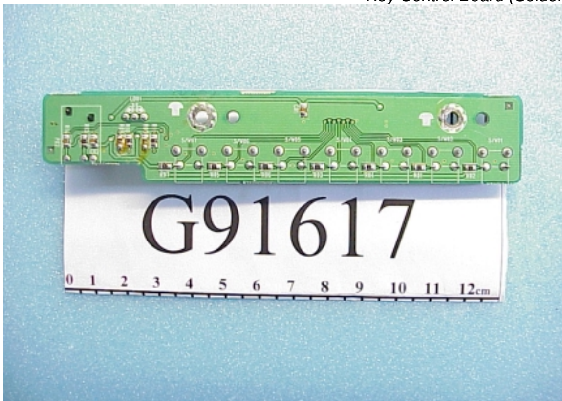
Figure 14 Key Control Board (Solder Side)
