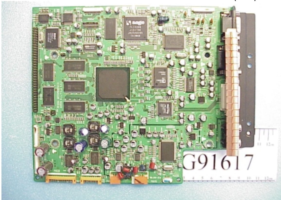
Figure 19 Main Board (Component Side)
