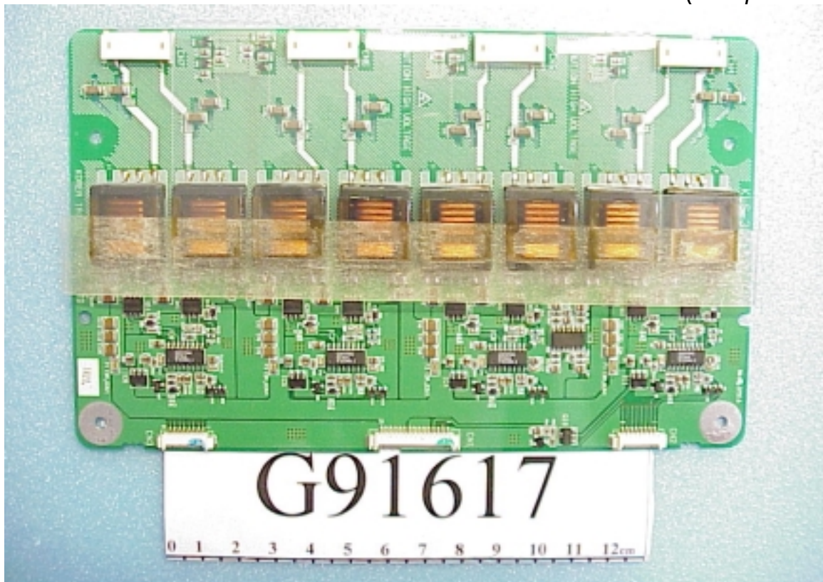
Figure 22 Inverter Board #1 (Component Side)
