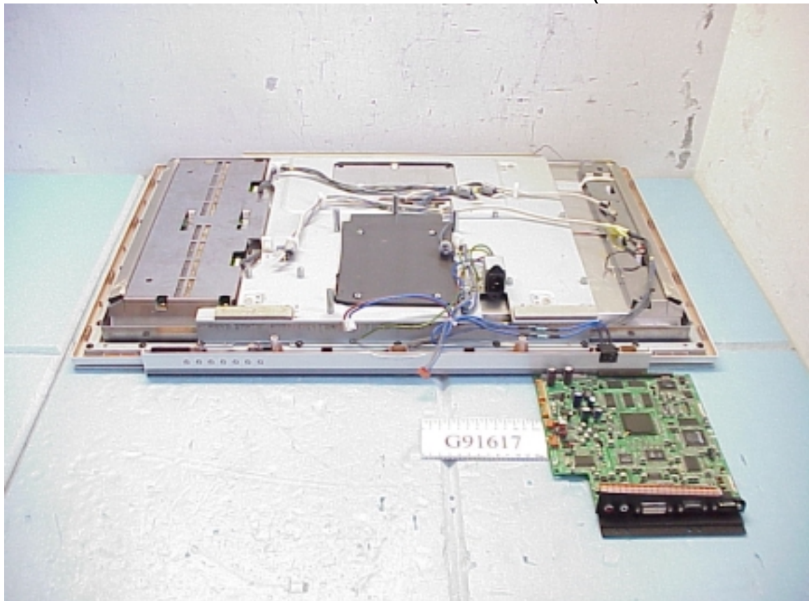
Figure 18 Internal View (Remove the Main Board)
