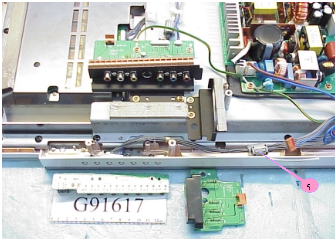
Figure 7 Internal View
