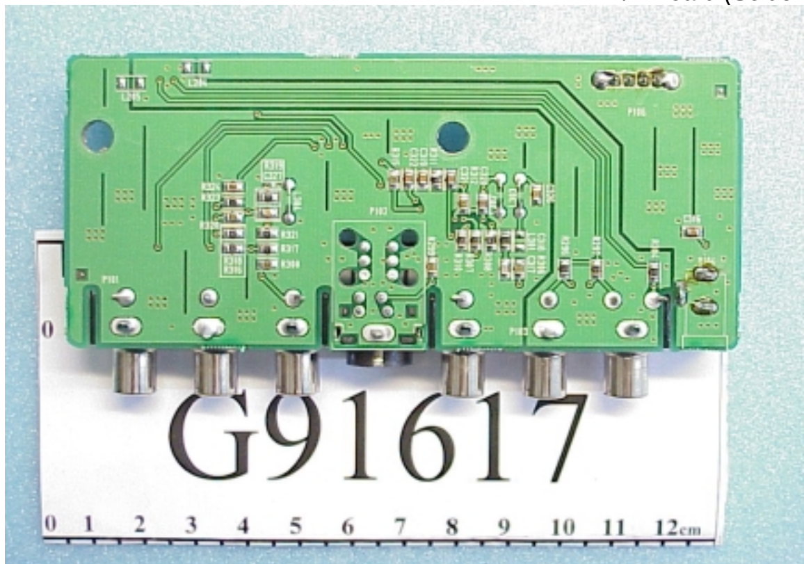
Figure 10 A/V Board (Solder Side)
