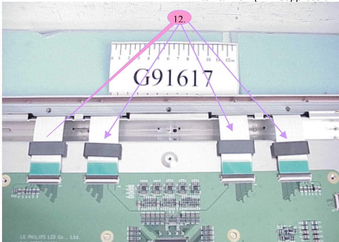
Figure 27 Internal View (EMI Suppression Parts)
