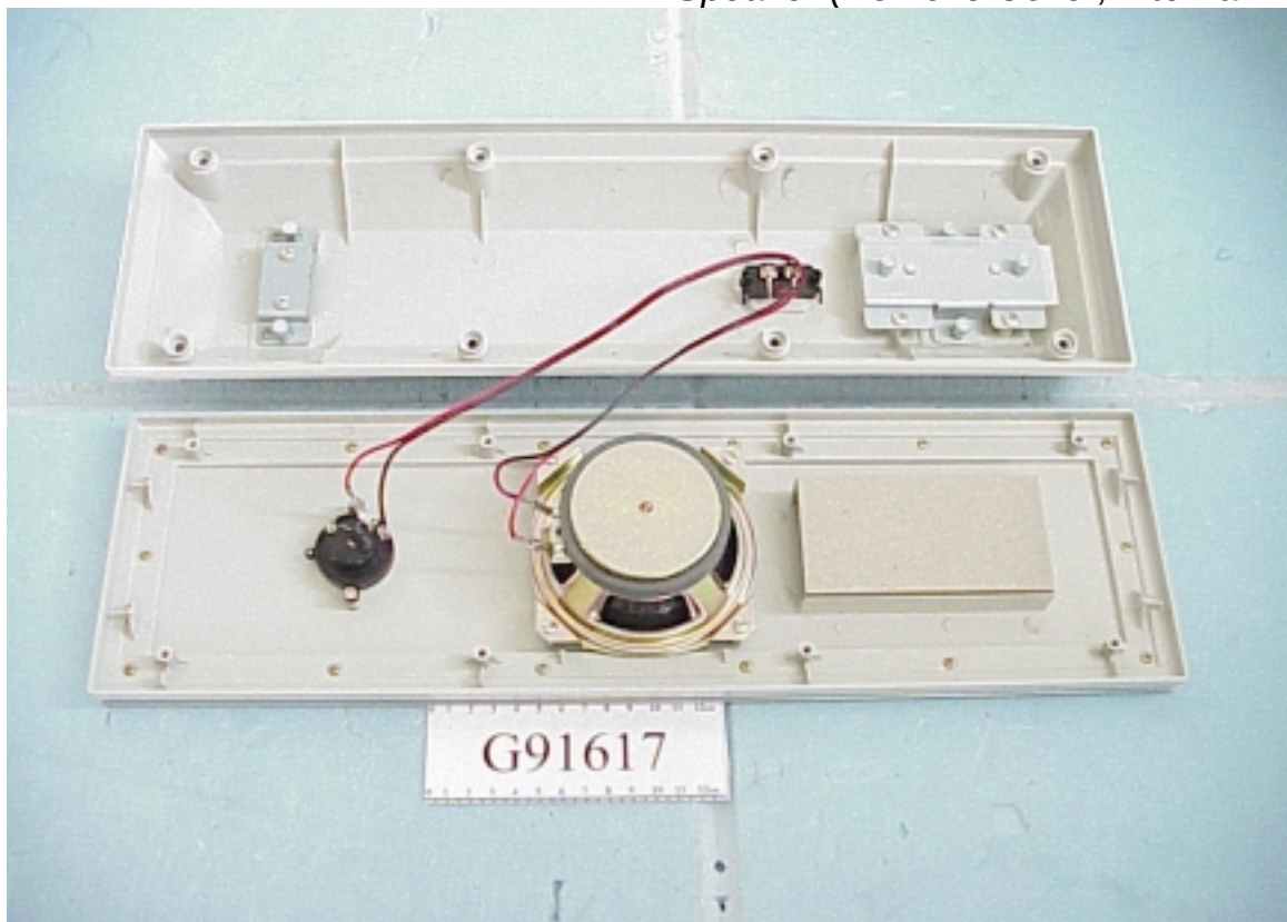
Figure 36 Speaker (Remove Cover, Internal Frame)
