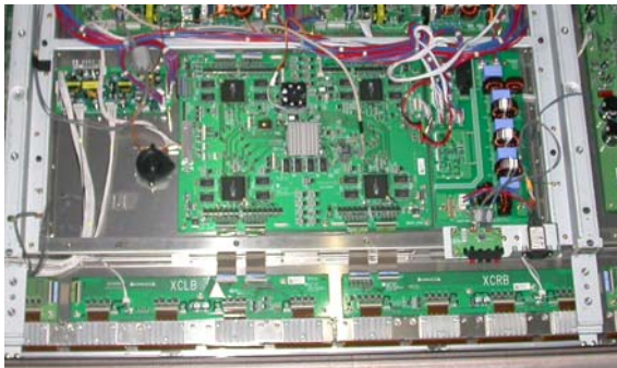
SIDE IN CTRL_LVDS BOARD
