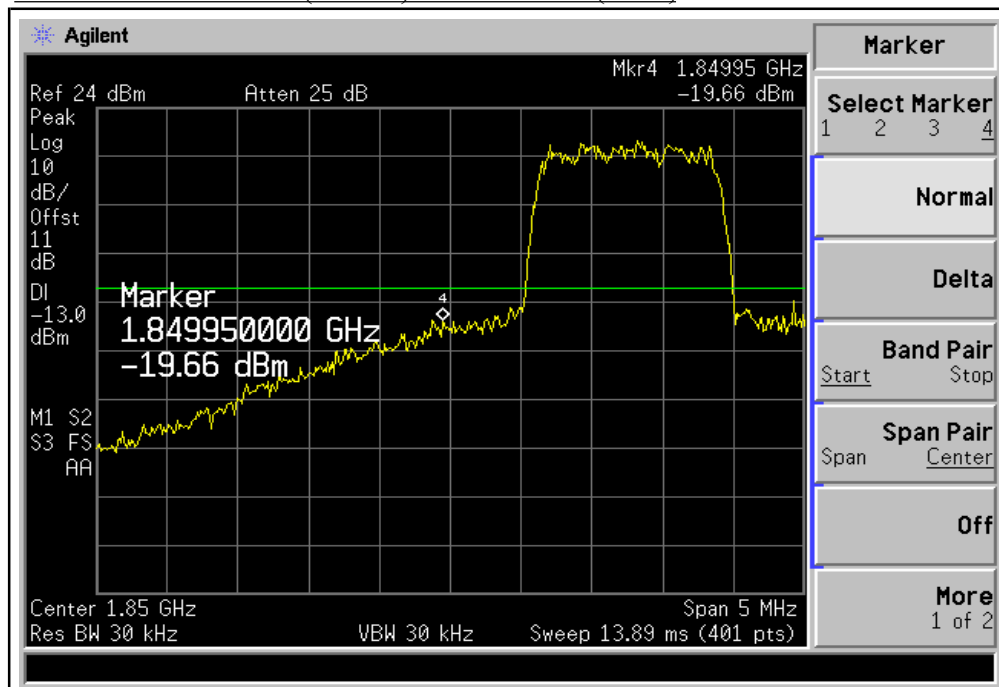
PLOTS OF EMISSION (CDMA): BAND EDGE(Ch25)
