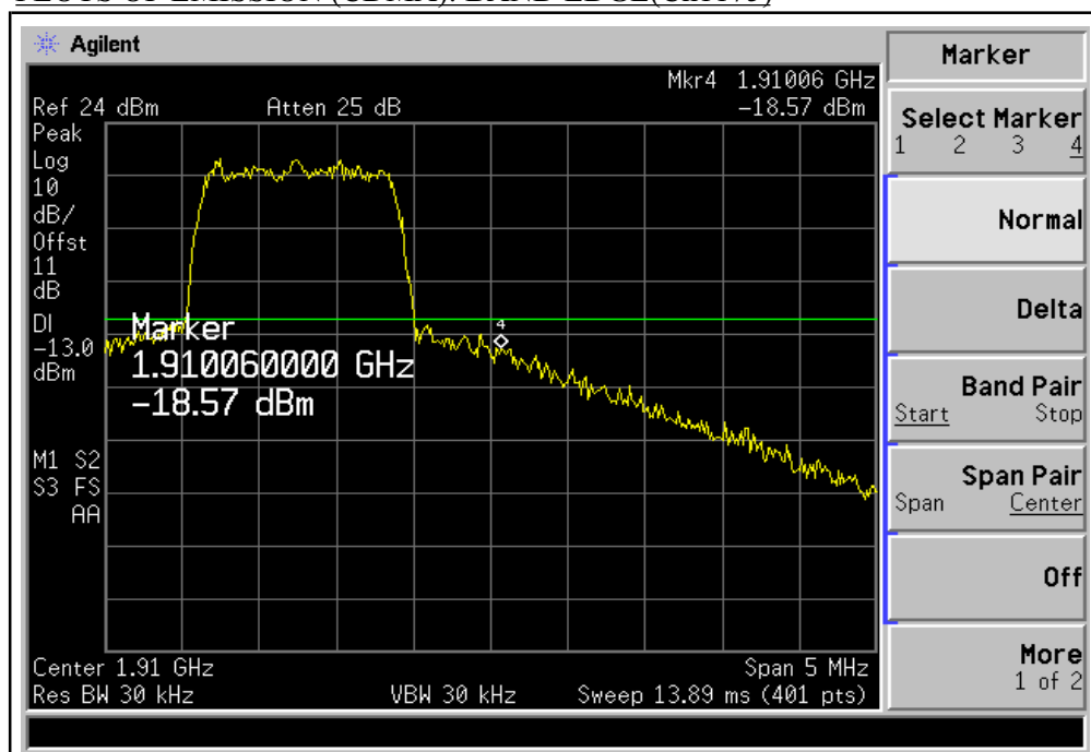
PLOTS OF EMISSION (CDMA): BAND EDGE(Ch1175)
