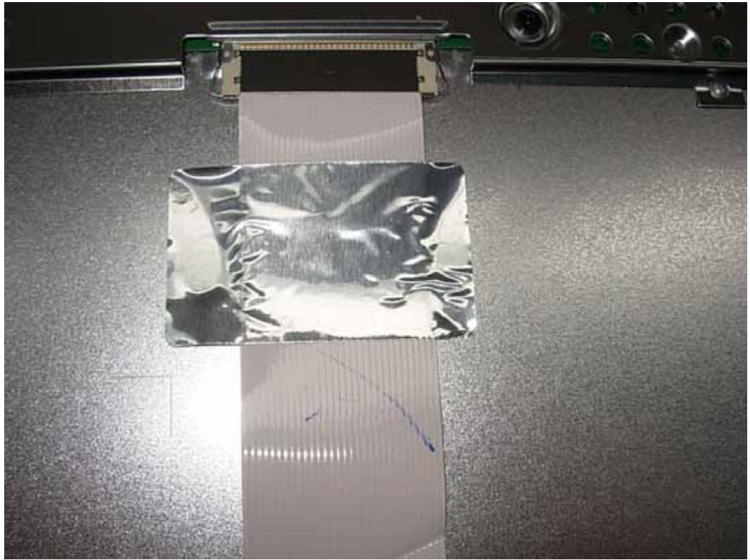
FIGURE 12 NETWORK MONITOR (M/N: N1942HET) DEBUG
