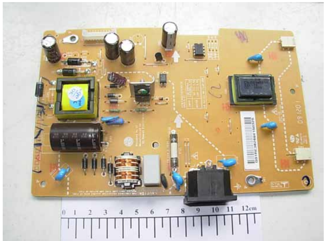
FIGURE 4 NETWORK MONITOR (M/N: N1942HET) POWER BOARD (COMPONENT SIDE)
